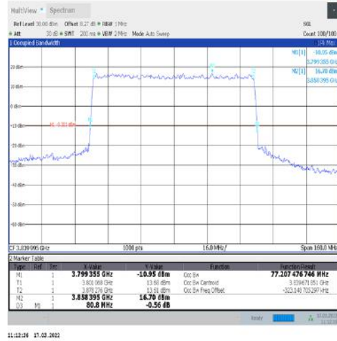
1-N77-3700-3980-30-80-M-1-DFT-QPSK-Outer_Full-216@0-Ant1-77.207-80.800-≤80-PASS
