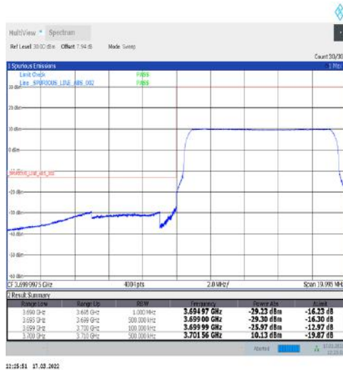
1-N77-3700-3980-30-10-L-6-CP-QPSK-Outer_Full-24@0-Ant1-PASS-see graph
