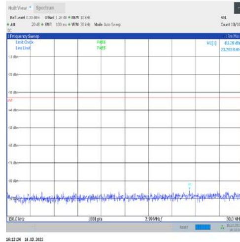
1-N77-3700-3980-30-100-L-1-DFT-PI2BPSK- Inner_1RB_Left-1@1-0.15-30-Ant1--85.28--33-PASS
