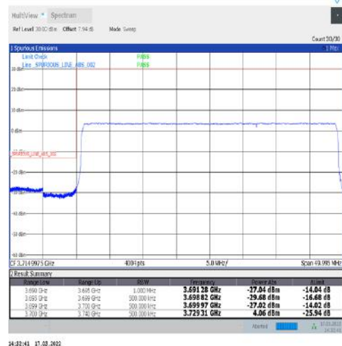
1-N77-3700-3980-30-40-L-6-CP-QPSK-Outer_Full-106@0-Ant1-PASS-see graph
