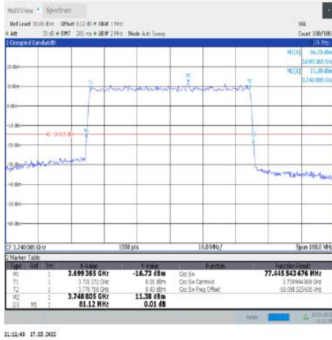
1-N77-3700-3980-30-80-L-9-CP-256QAM-Outer_Full-217@0-Ant1-77.446-81.120-≤80-PASS
