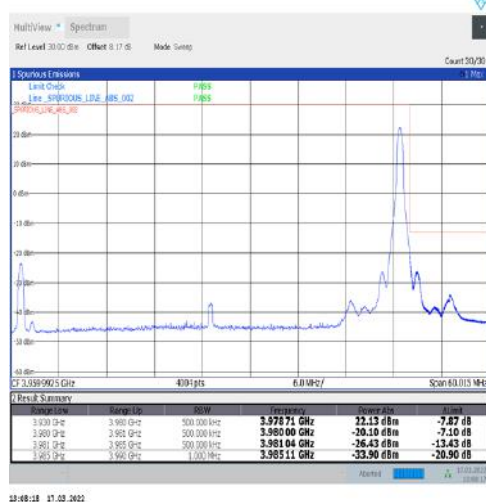
1-N77-3700-3980-30-50-H-5-CP-QPSK-Edge_1RB_Right-1@132-Ant1-PASS-see graph
