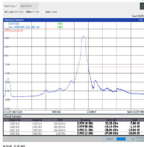
1-N77-3700-3980-30-15-H-2-DFT-PI2BPSK-Edge_1RB_Right-1@37-Ant1-PASS-see graph
