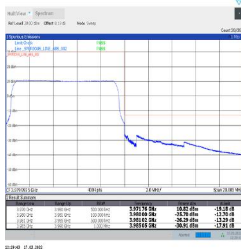
1-N77-3700-3980-30-10-H-6-CP-QPSK-Outer_Full-24@0-Ant1-PASS-see graph
