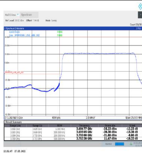
1-N77-3700-3980-30-15-L-3-DFT-PI2BPSK-Outer_Full-36@0-Ant1-PASS-see graph
