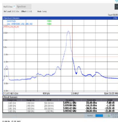
1-N77-3700-3980-30-15-H-5-CP-QPSK-Edge_1RB_Right-1@37-Ant1-PASS-see graph
