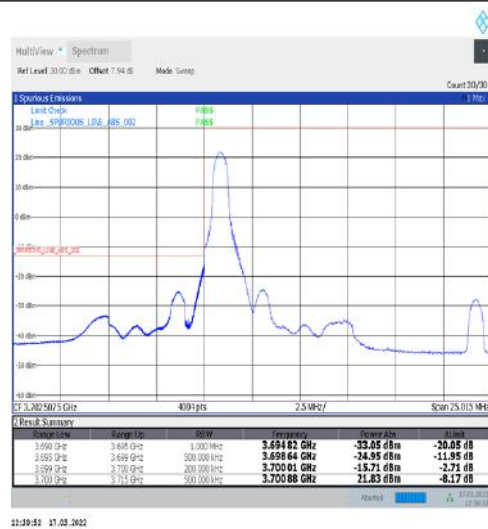
1-N77-3700-3980-30-15-L-1-DFT-PI2BPSK-Edge_1RB_Left-1@0-Ant1-PASS-see graph
