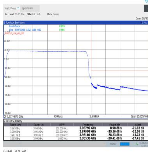
1-N77-3700-3980-30-15-H-6-CP-QPSK-Outer_Full-38@0-Ant1-PASS-see graph
