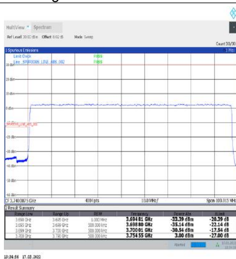
1-N77-3700-3980-30-90-L-3-DFT-PI2BPSK-Outer_Full-240@0-Ant1-PASS-see graph
