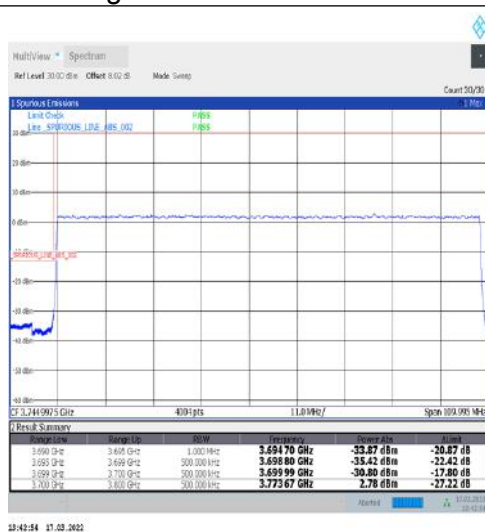
1-N77-3700-3980-30-100-L-3-DFT-PI2BPSK-Outer_Full-270@0-Ant1-PASS-see graph
