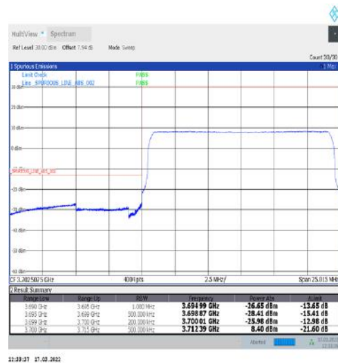
1-N77-3700-3980-30-15-L-6-CP-QPSK-Outer_Full-38@0-Ant1-PASS-see graph
