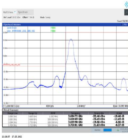
1-N77-3700-3980-30-10-L-4-CP-QPSK-Edge_1RB_Left-1@0-Ant1-PASS-see graph
