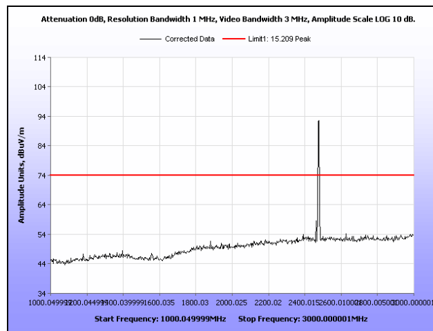
Plot 21. Radiated Spurious Emissions, High Channel, 1 GHz – 3 GHz, Peak
