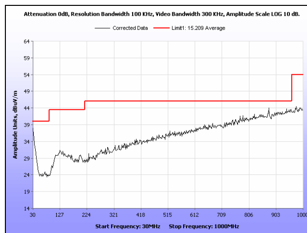
Plot 19. Radiated Spurious Emissions, High Channel, 30 MHz – 1 GHz
