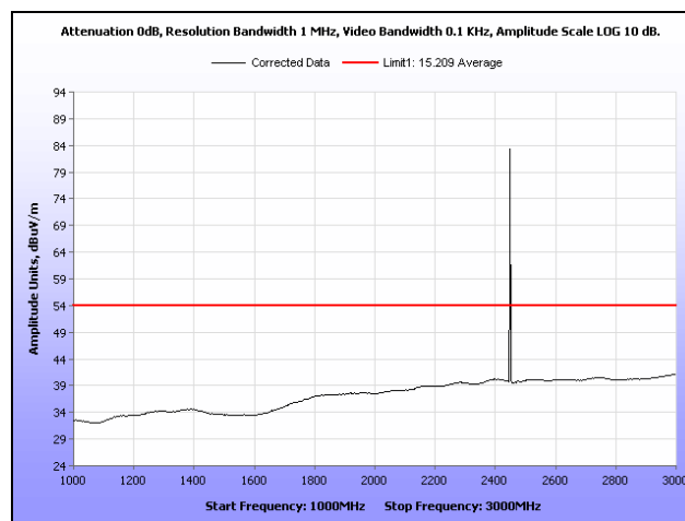
Plot 13. Radiated Spurious Emissions, Mid Channel, 1 GHz – 3 GHz, Average
