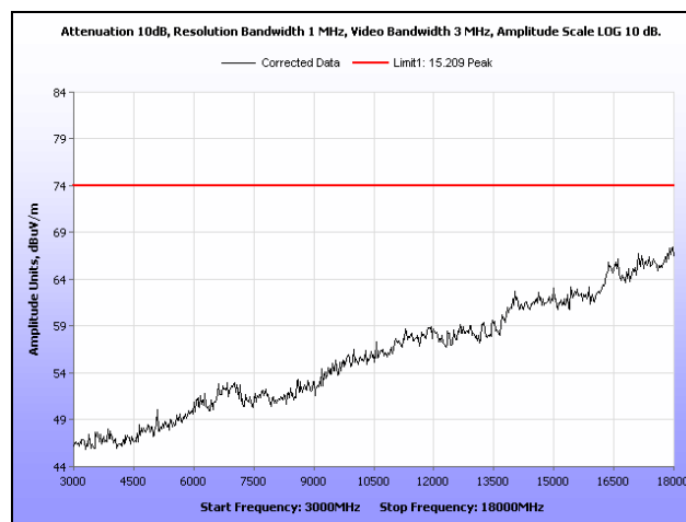
Plot 16. Radiated Spurious Emissions, Mid Channel, 3 GHz – 18 GHz, Peak
