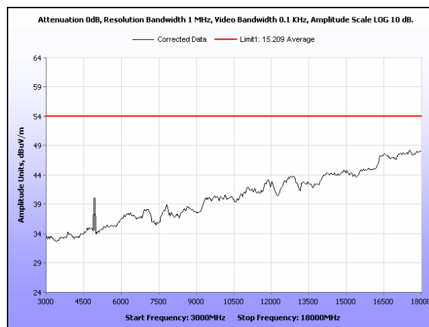
Plot 22. Radiated Spurious Emissions, High Channel, 3 GHz – 18 GHz, Average
