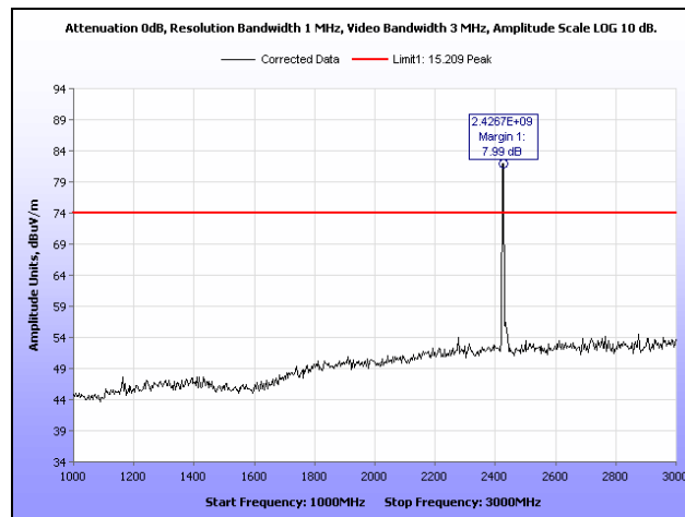
Plot 7. Radiated Spurious Emissions, Low Channel, 1 GHz – 3 GHz, Peak
