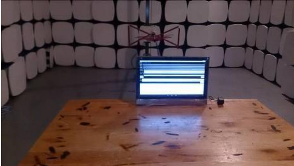
Radiated Emission (above 1GHz)
