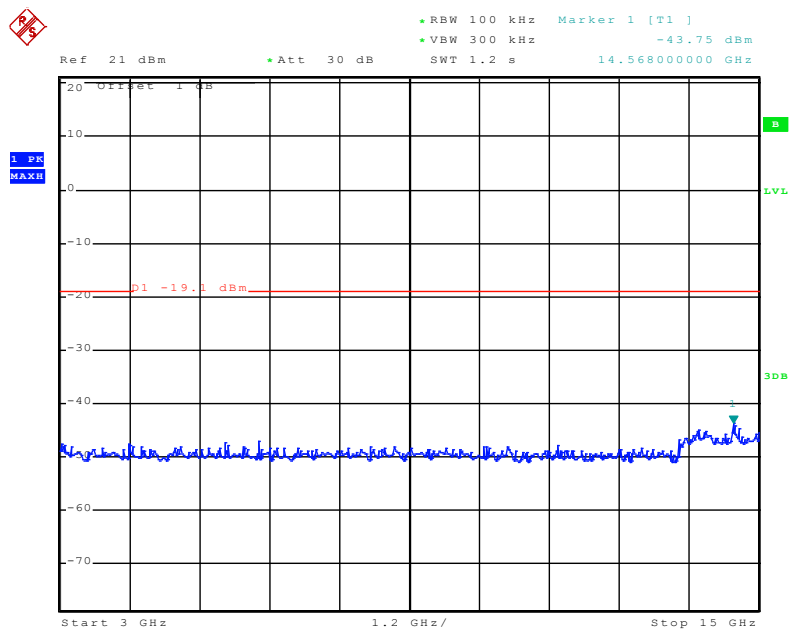
(Plot 3.7.3 A1: Channel 1: 2412MHz @ 802.11n(20MHz))
