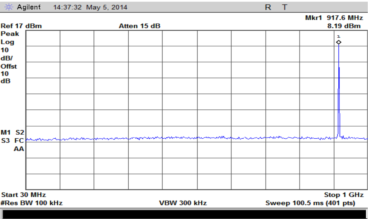
Plot 4 – Conducted Spurious 30MHz – 1GHz
