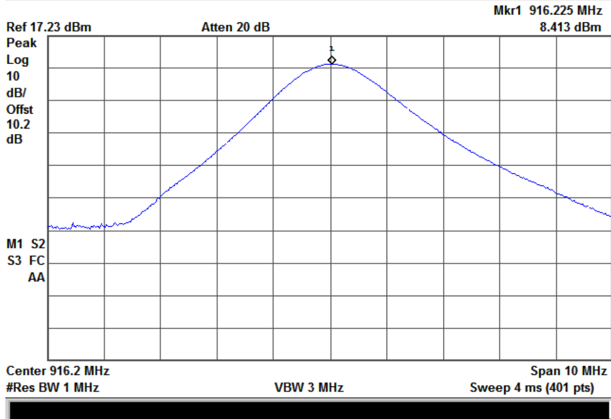
Plot 3 – Output Power
