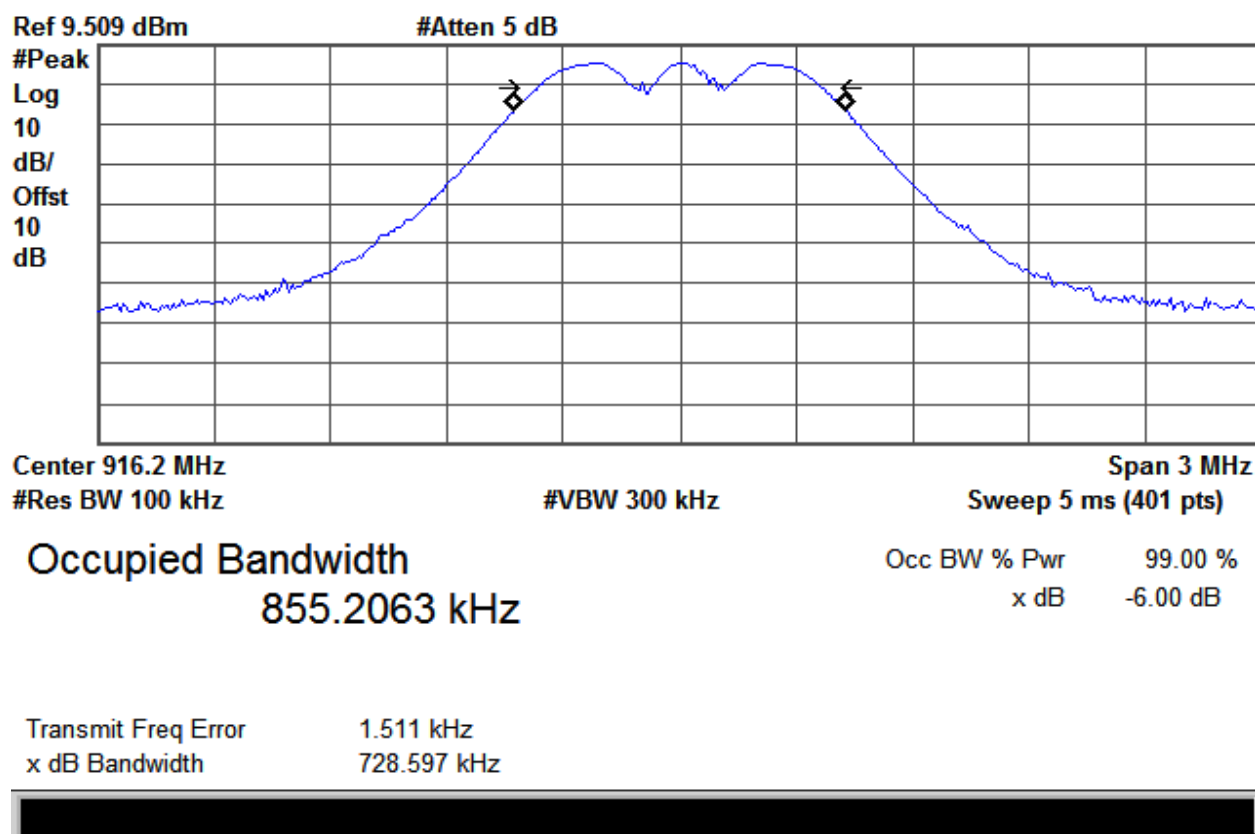
Plot 2 – Occupied Bandwidth – 6dB BW
