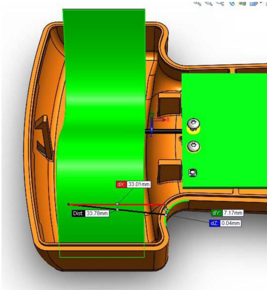
Figure 1 - Measurement from closest point the hand might contact the enclosure to the radiating structure on the antenna
