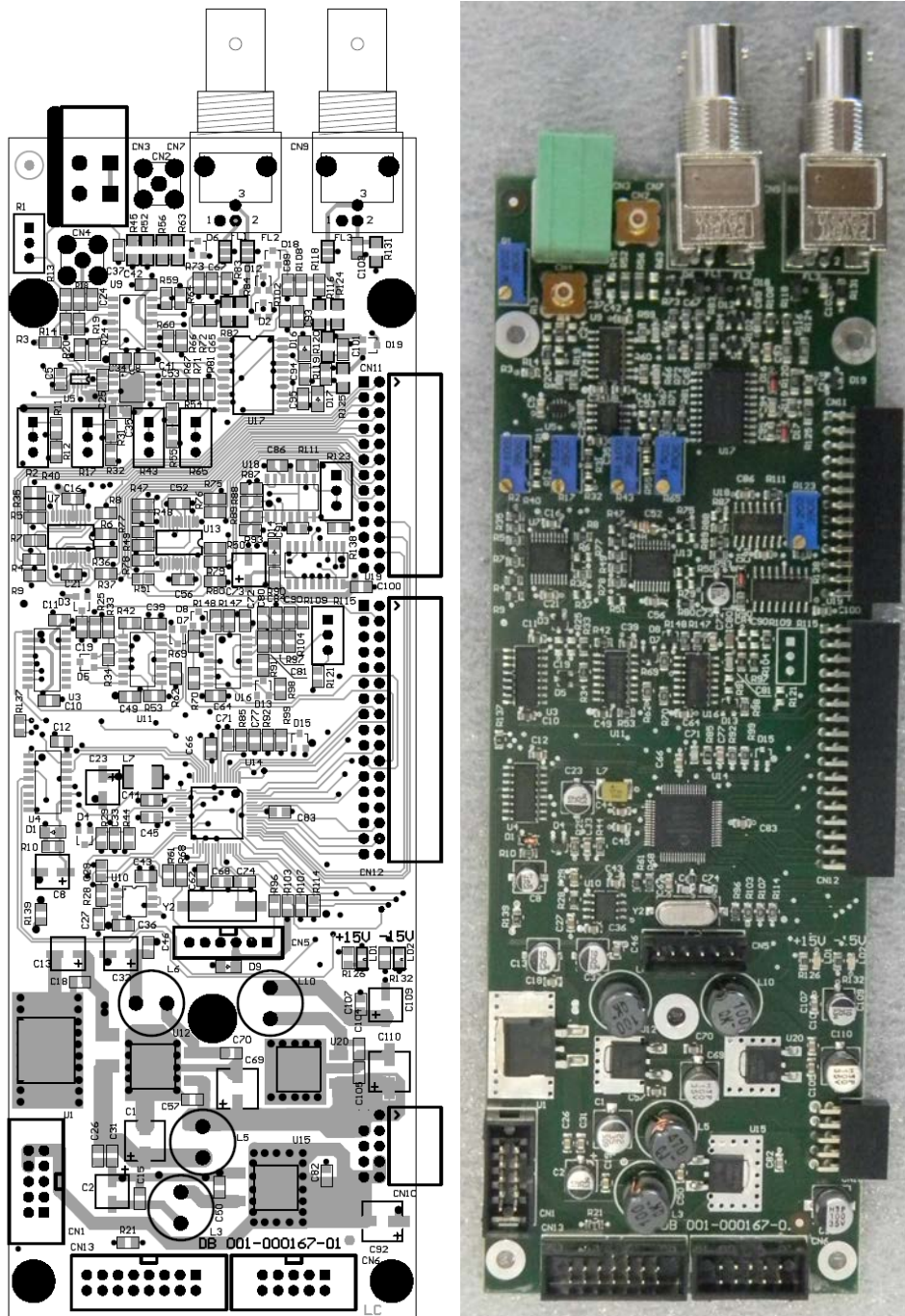
Fig. 6.10 – MPX IN BOARD LAYOUT (L02-000167)
