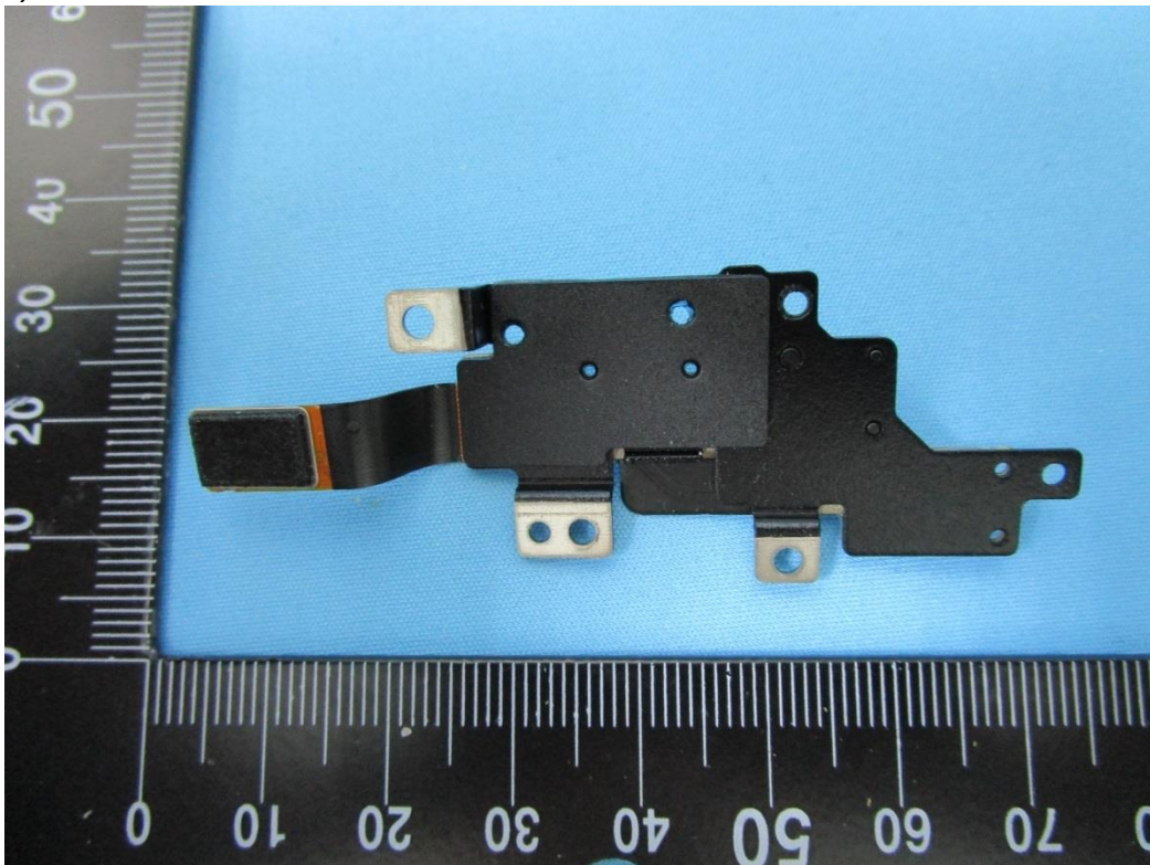
(22) EUT Photo
