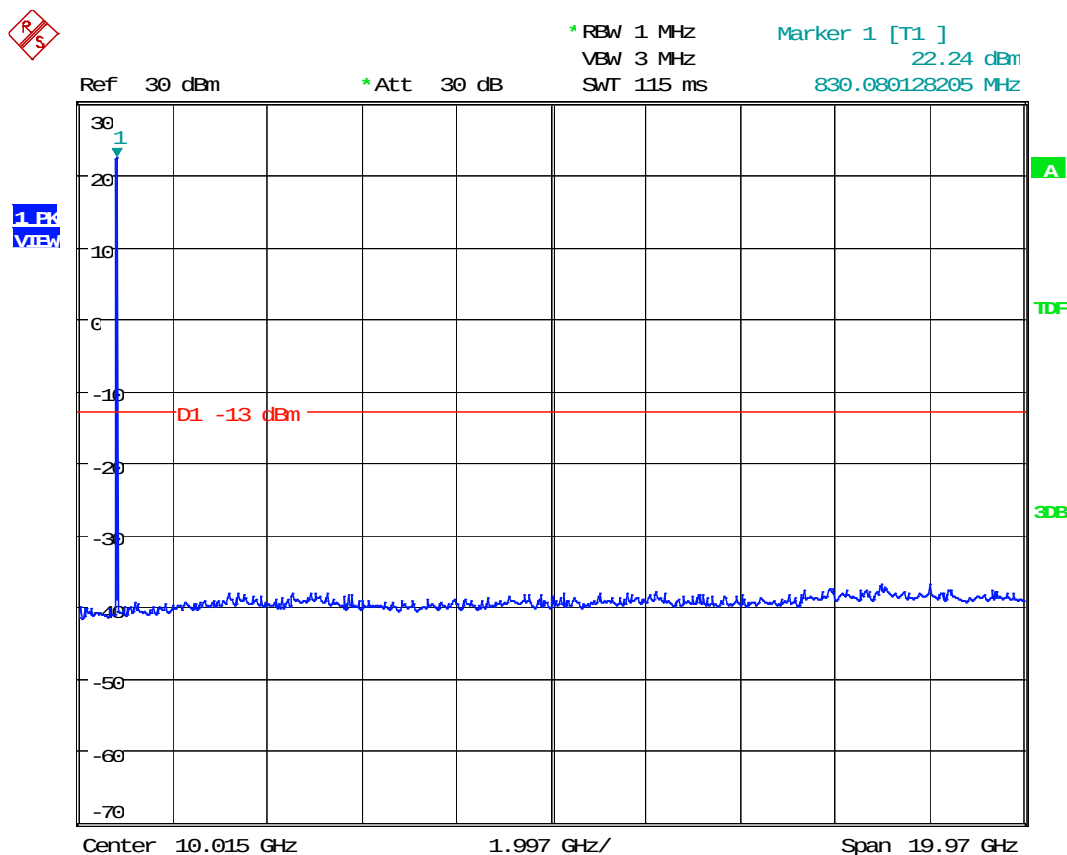
Conducted Emission Transmitting Mode WCDMA BAND V CH 4132
