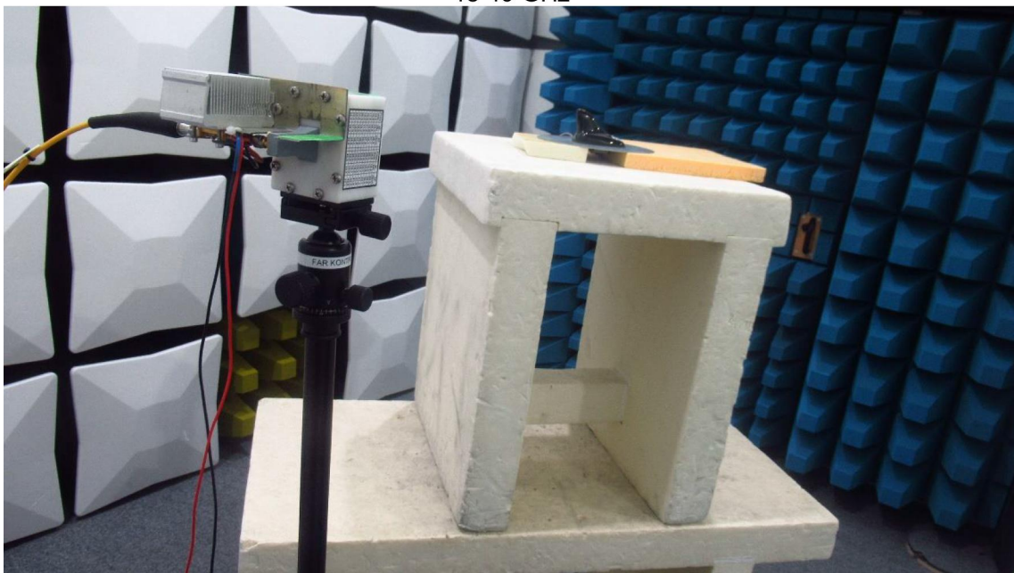
18-40 GHz
