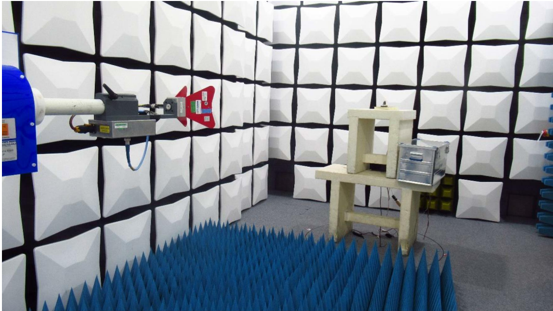
18-40 GHz
