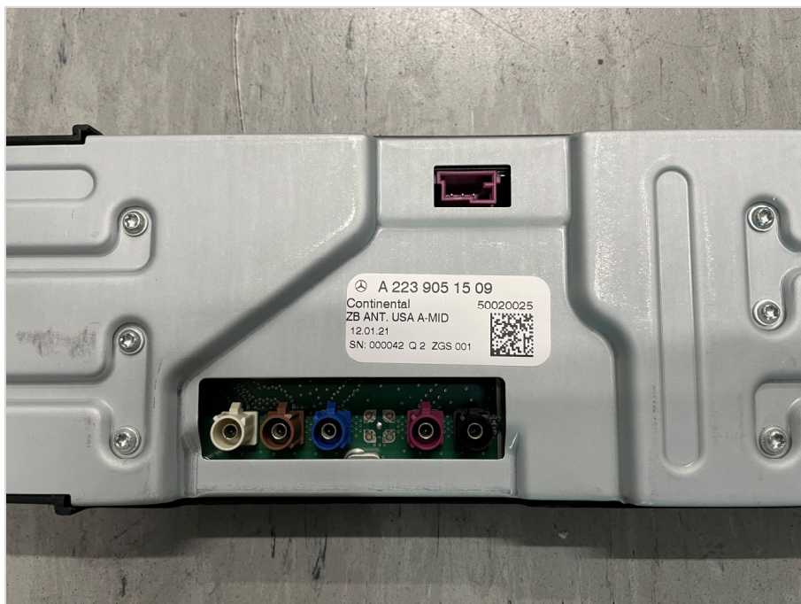
Photograph 3: EUT 1_Close up view on connector
