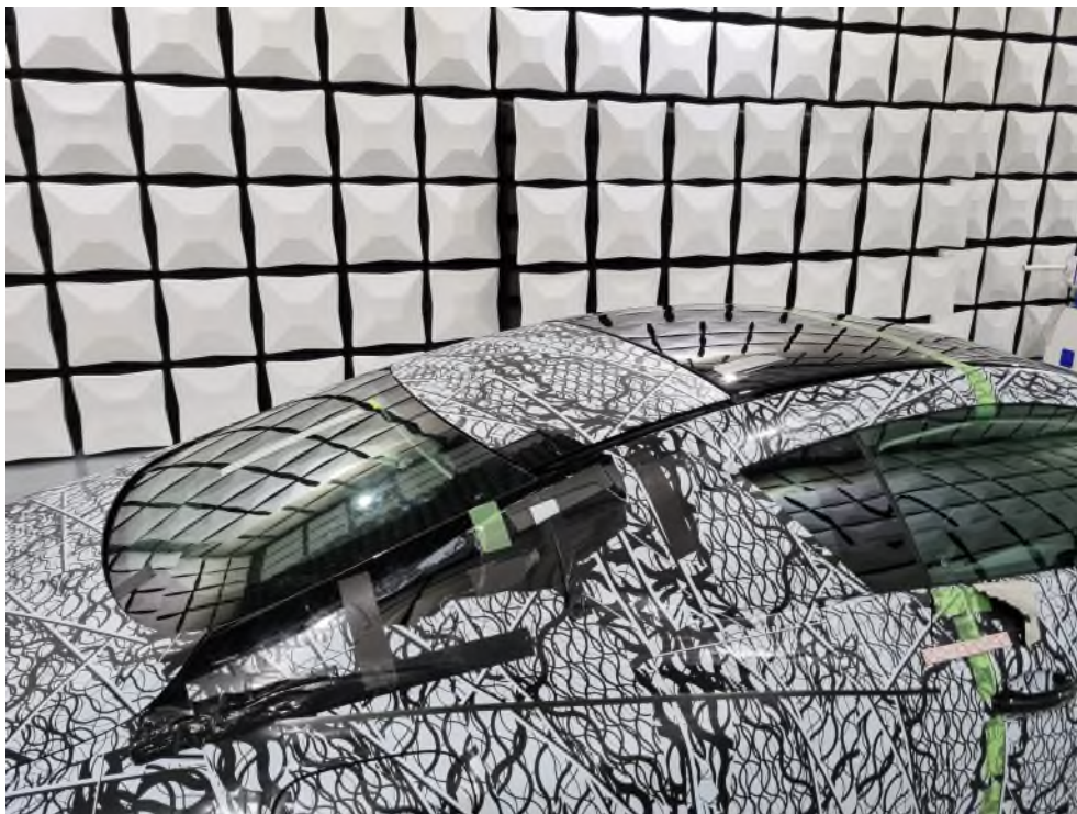
Fig. 6: EUT support details: set up when measuring the real antenna installed at the car
