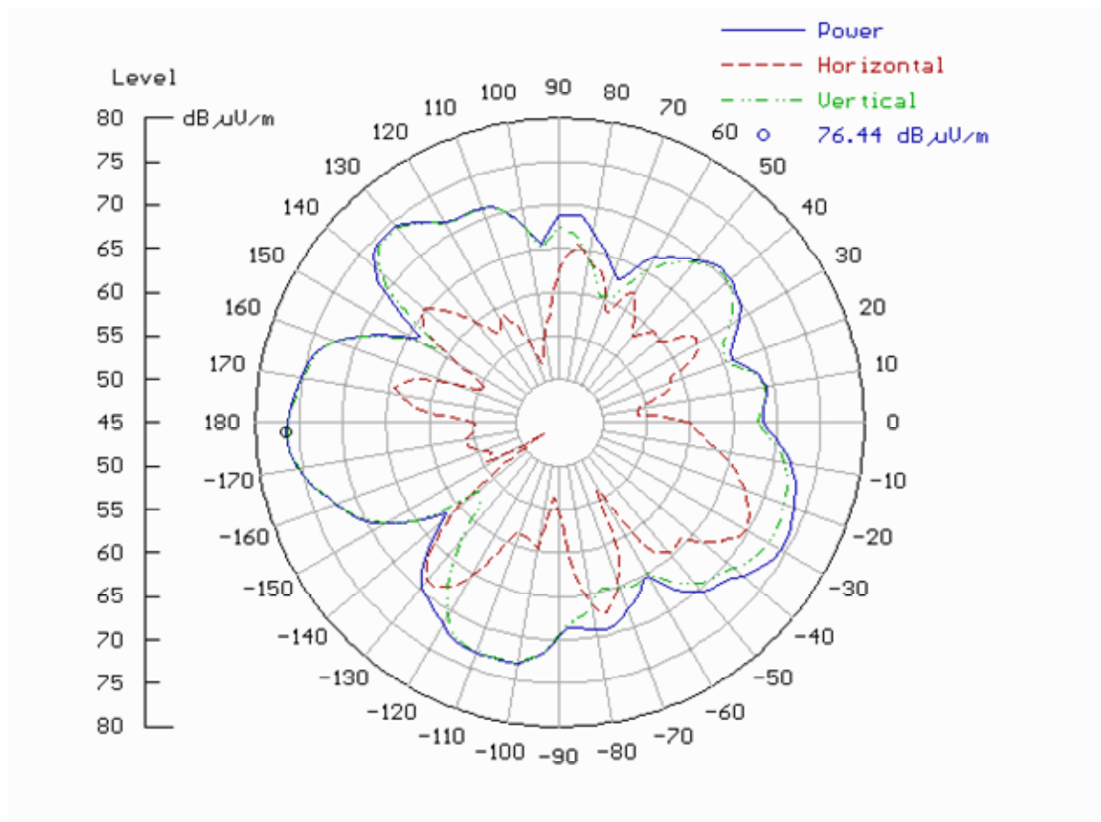
Fig. 7: Maximum EIRP value found for 434 MHz antenna when attached to real car in worst case scenario and when set to appropriate modulation, timing and power value 0x2D.
