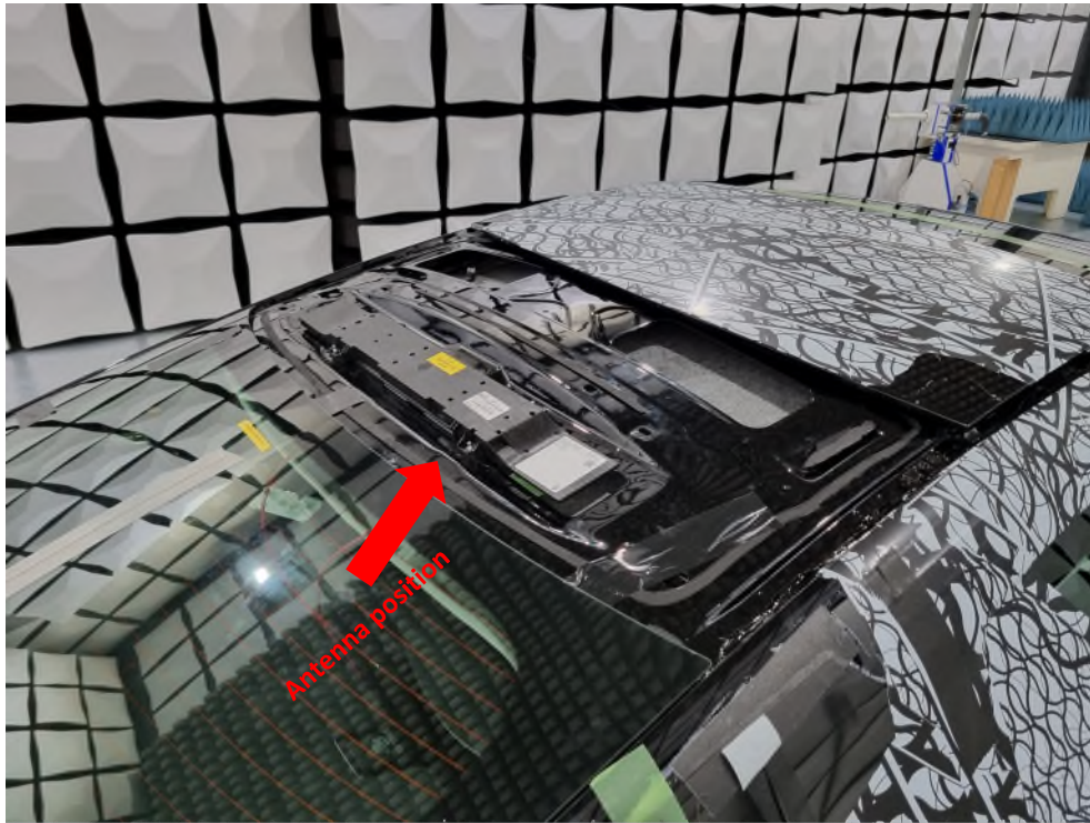
Fig. 3: Photo and indication of antenna position
