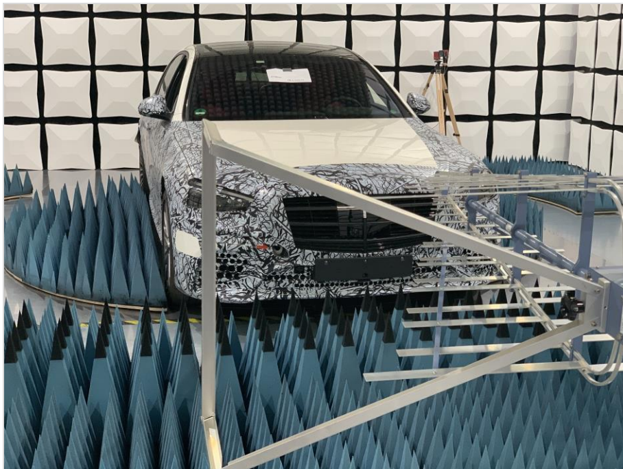
Photograph 2: EUT Test Setup in the anechoic chamber, Radiated interference field strength, frequencies above 1GHz
