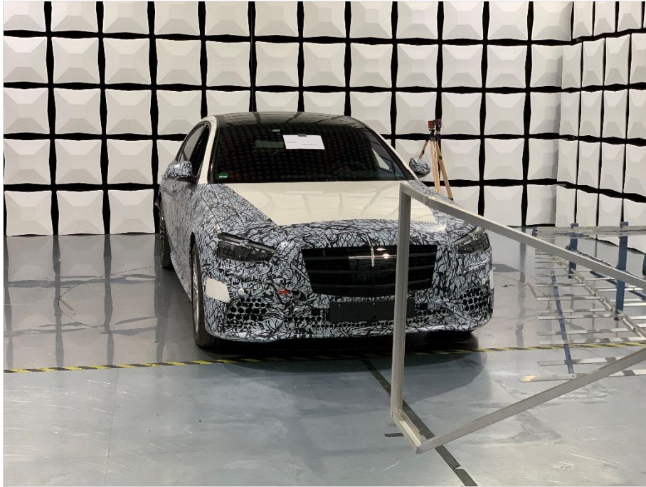
Photograph 1: EUT Test Setup in the anechoic chamber, Radiated interference field strength (frequency range below 1GHz)
