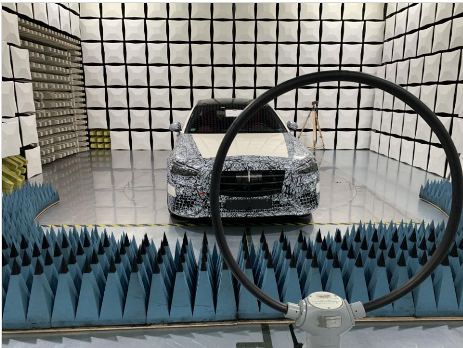
Photograph 4: EUT Setup Magnetic Field Measurements in the Semi anechoic chamber (9kHz to 30MHz frequency range)
