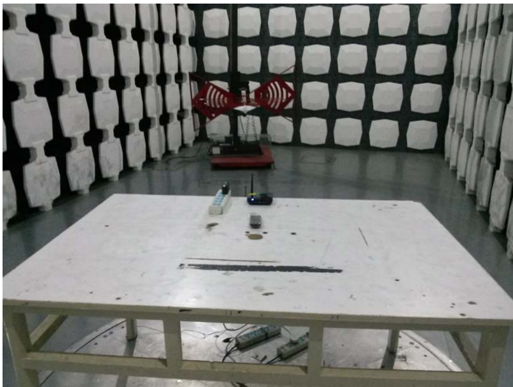
Set-up for Radiated Emission Test
