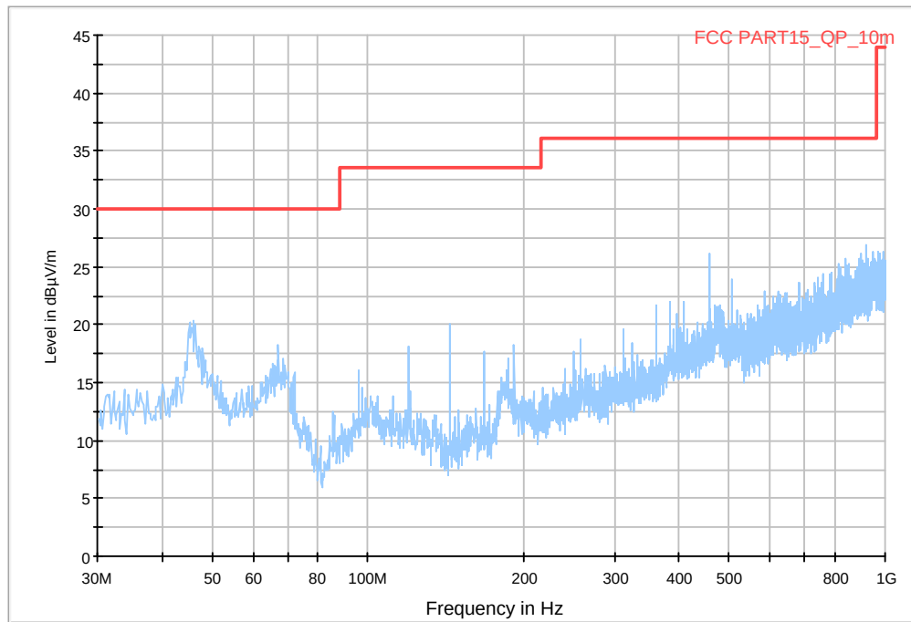
Fig.5 Radiated Emission from 30MHz to 1GHz
