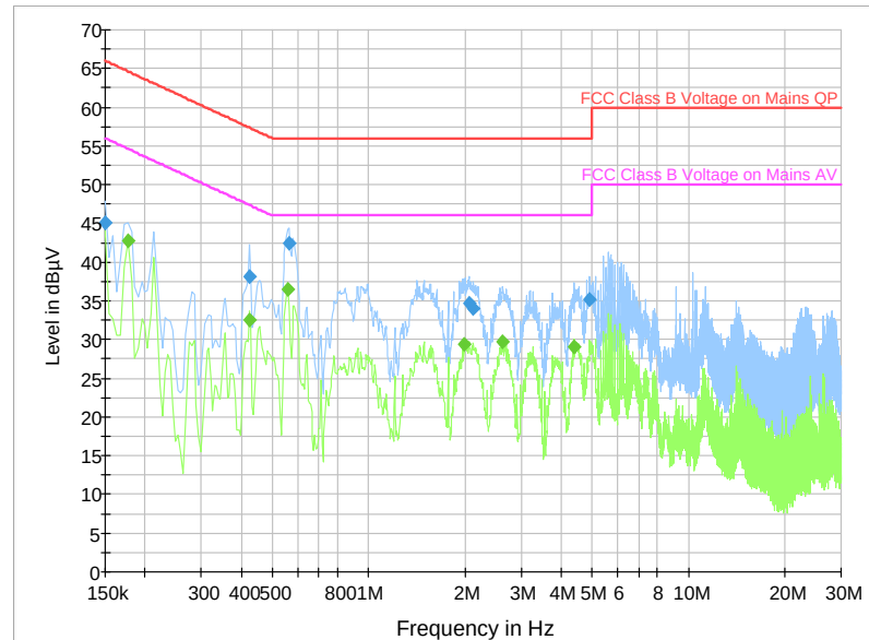
Fig.9 Conducted Emission
