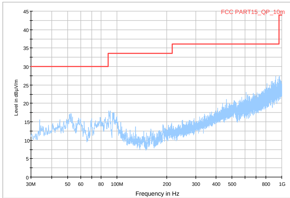
Fig.3 Radiated Emission from 30MHz to 1GHz
