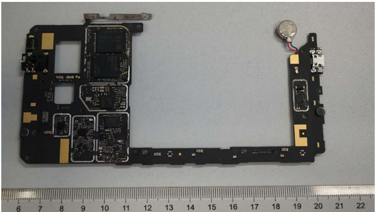
Mobile Phone Disassembly
