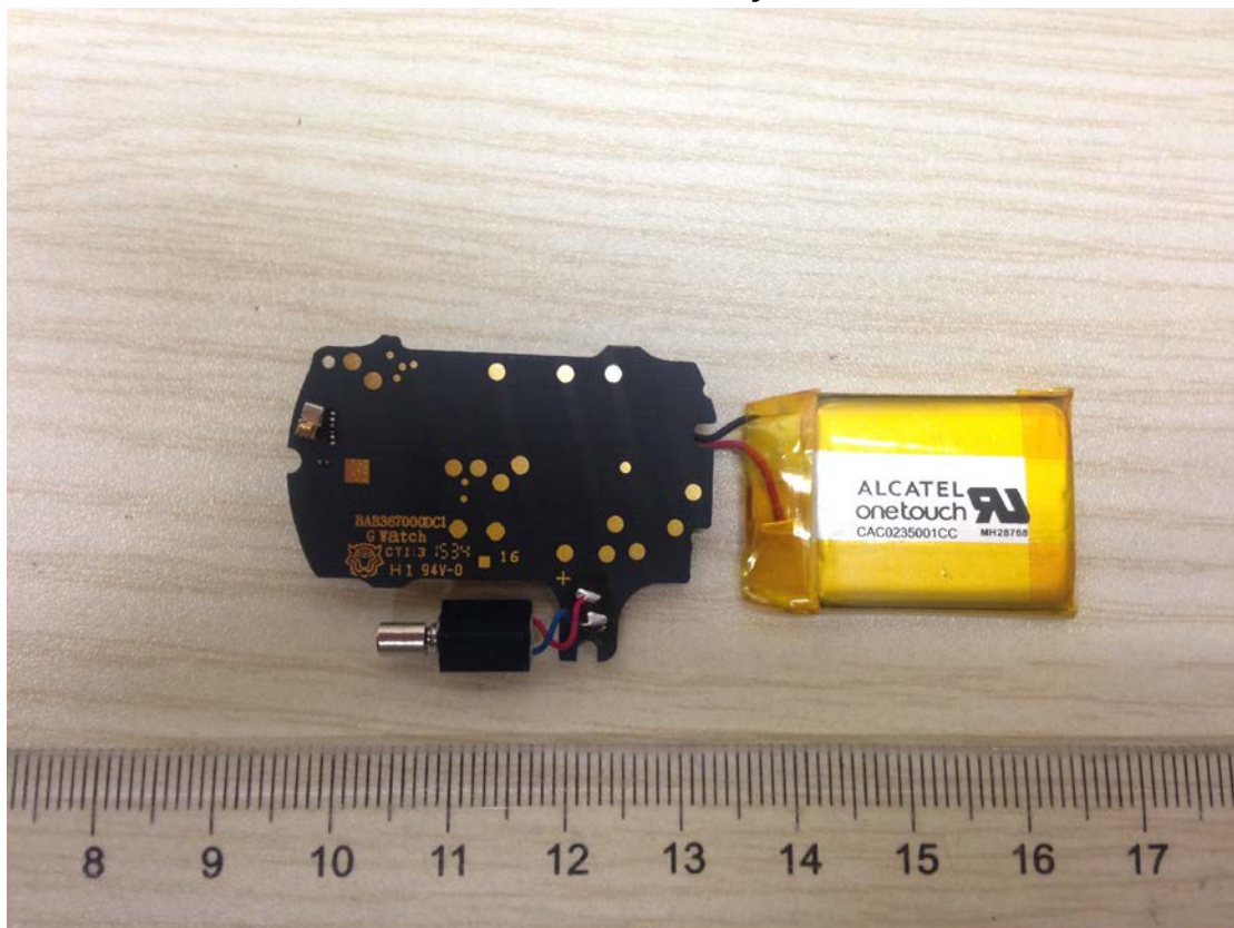
Watch Disassembly
