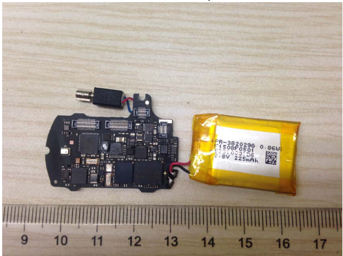
Watch Disassembly
