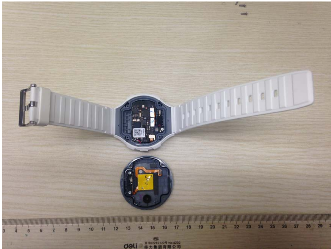
Watch Disassembly
