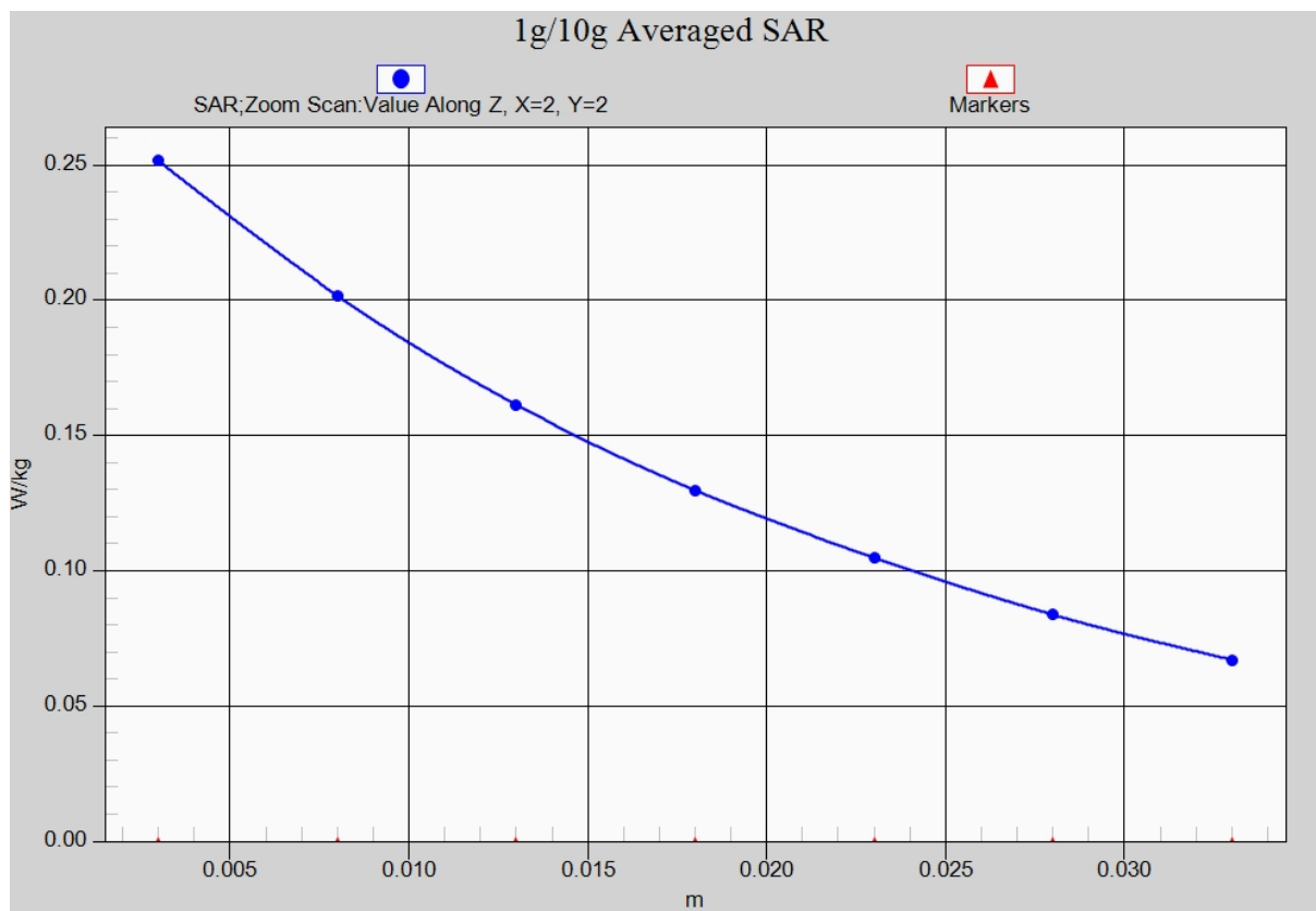
Fig. 14-1 Z-Scan at power reference point (CDMA BC0)
