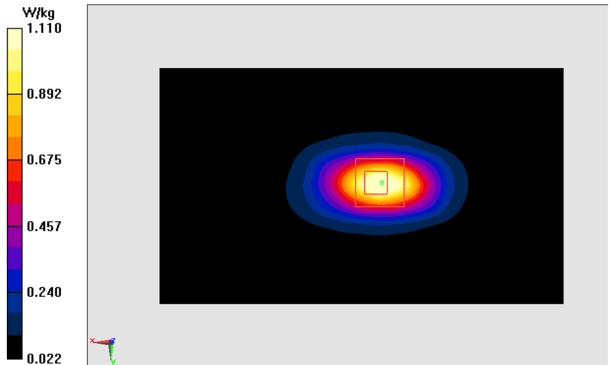
Fig.45 LTE Band66
