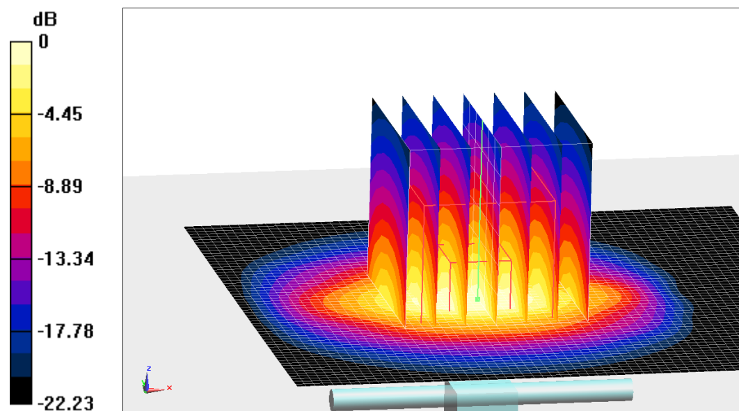
Fig.B.12 validation 2600 MHz 250mW
