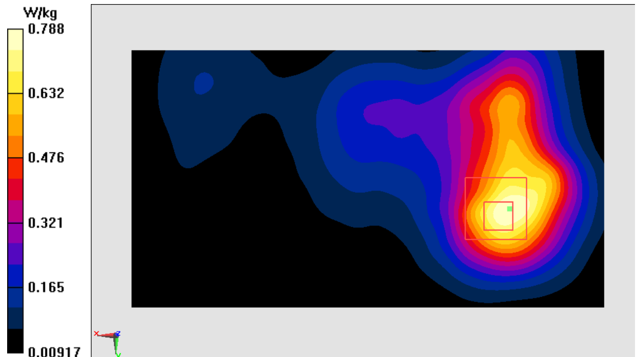
Fig.47 2450 MHz
