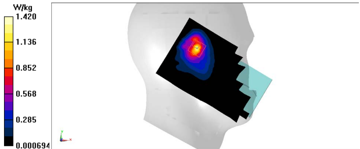
Fig.46 2450 MHz
