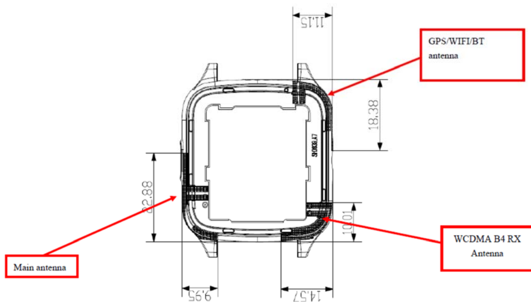
Picture 4: Antenna Location
