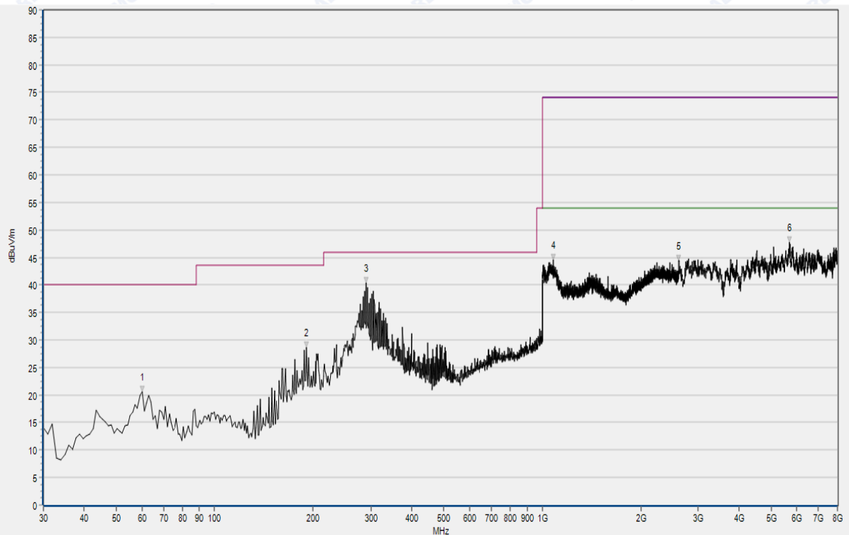
(Plot D: Battery TLp040FD, ANT-Horizontal, 30MHz – 8GHz)
