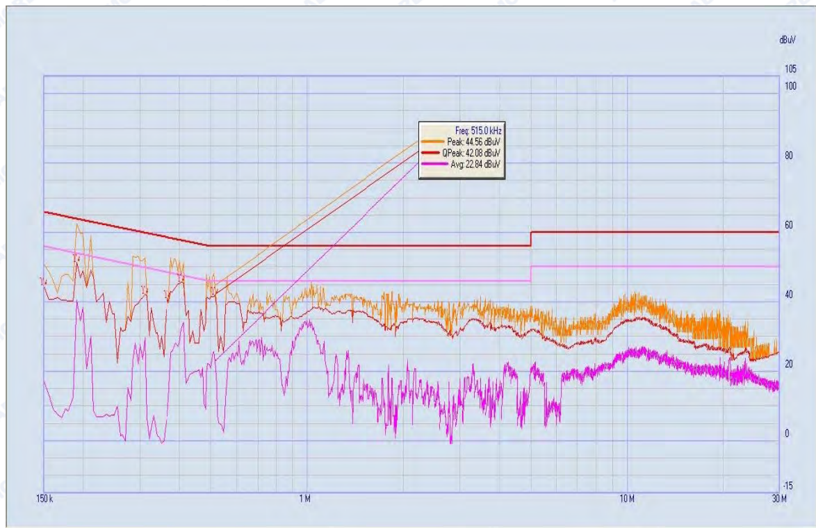
(Plot C: battery TLp040FD, L Phase)
