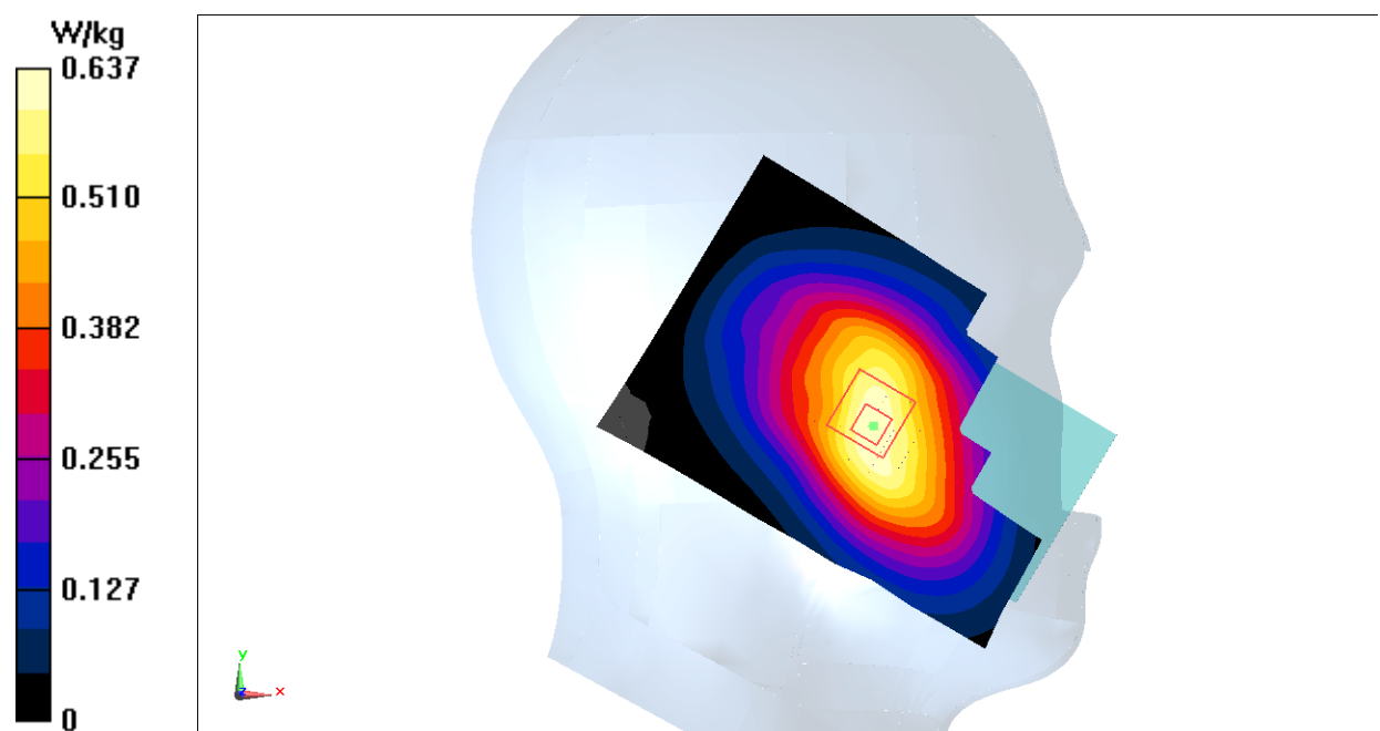
Fig.1 CDMA BC0
