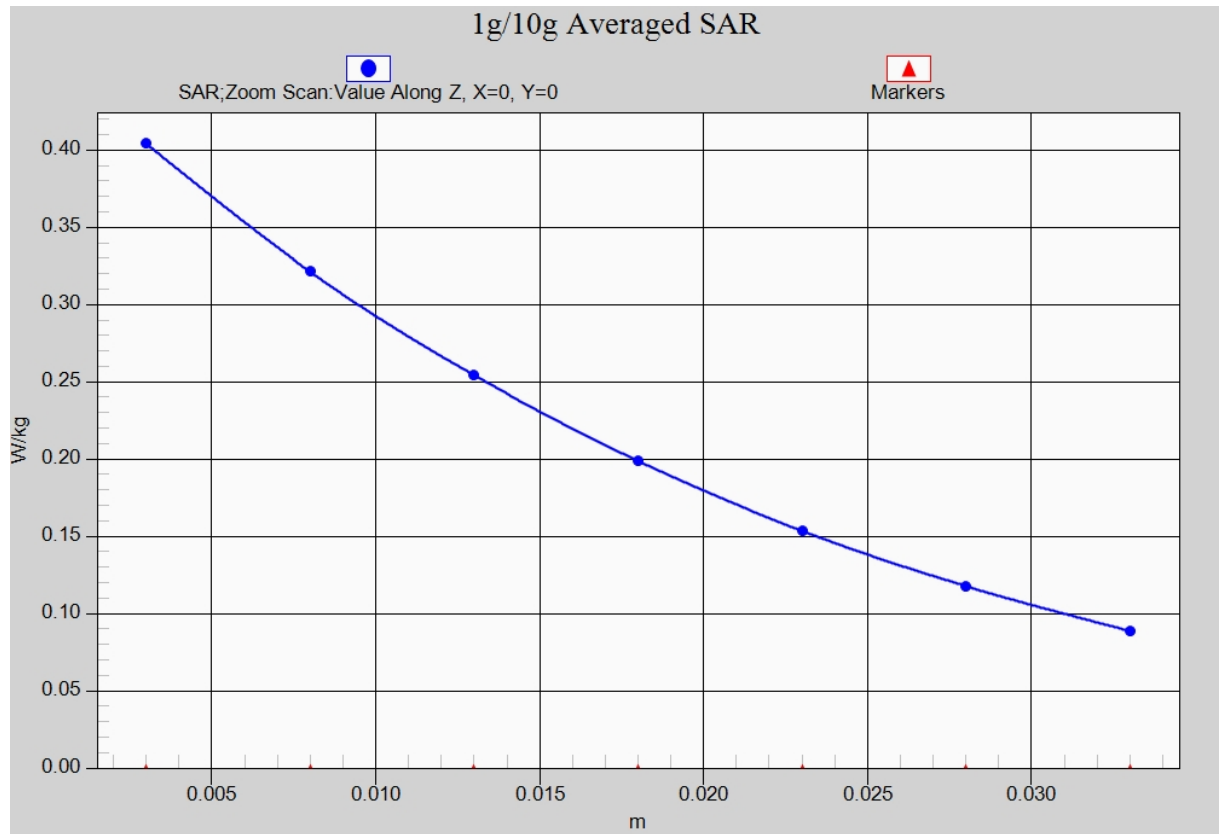
Fig. 1-1 Z-Scan at power reference point (CDMA BC0)
