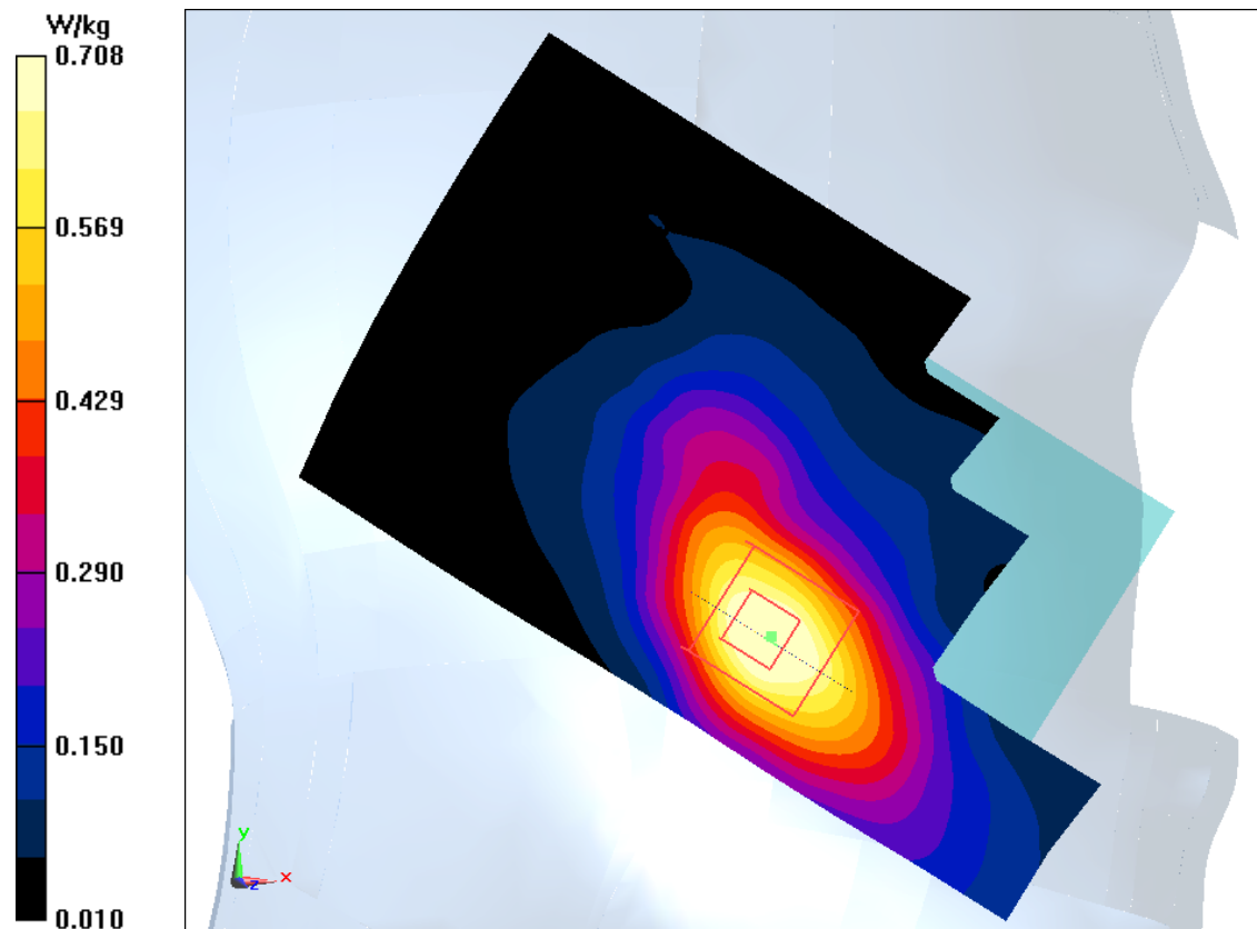
Fig.I.2 CDMA BC1
