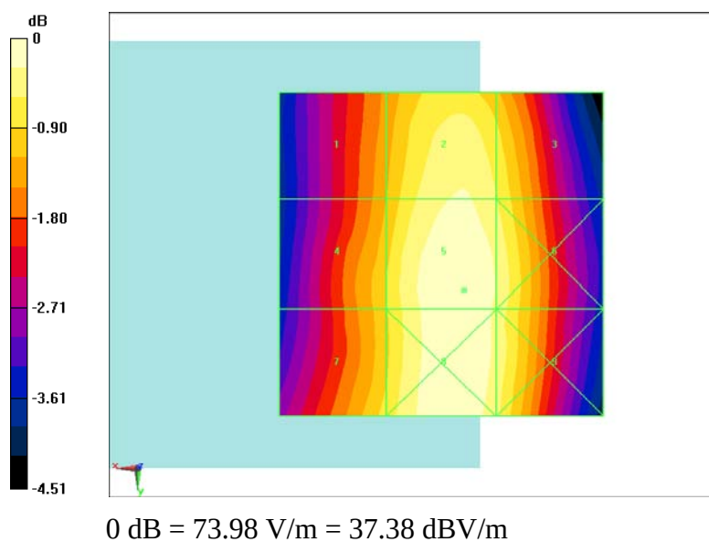
Fig B.2 HAC RF E-Field GSM 850 Middle
