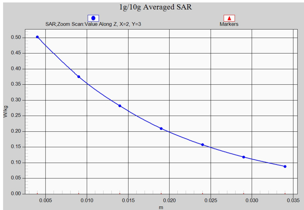
Fig.17-1 Z-Scan at power reference point (LTE Band13)
