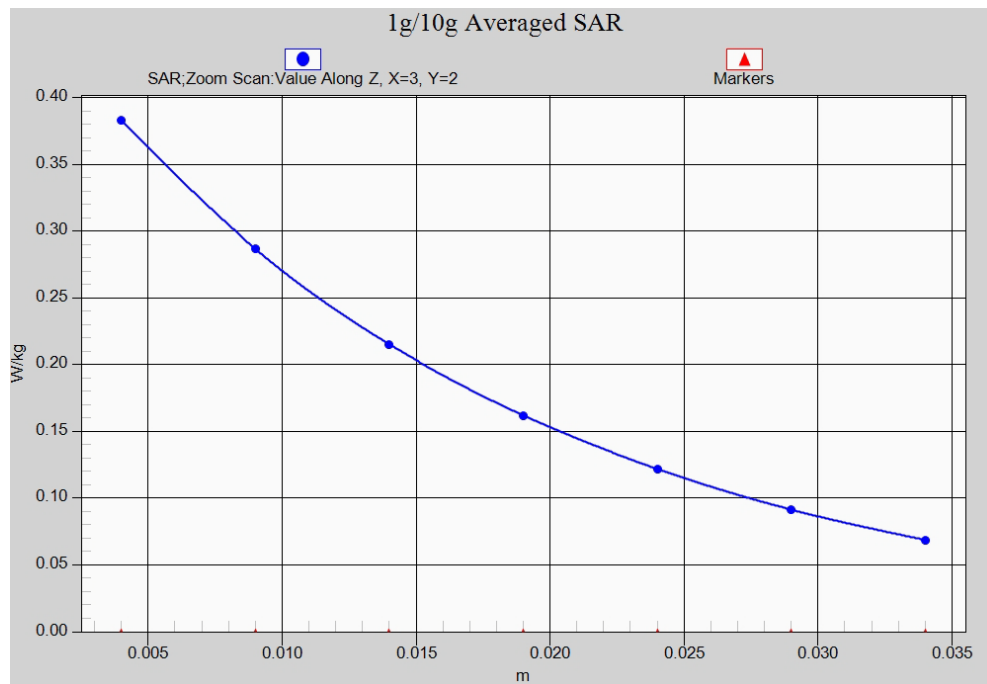
Fig. 19-1 Z-Scan at power reference point (LTE Band17)
