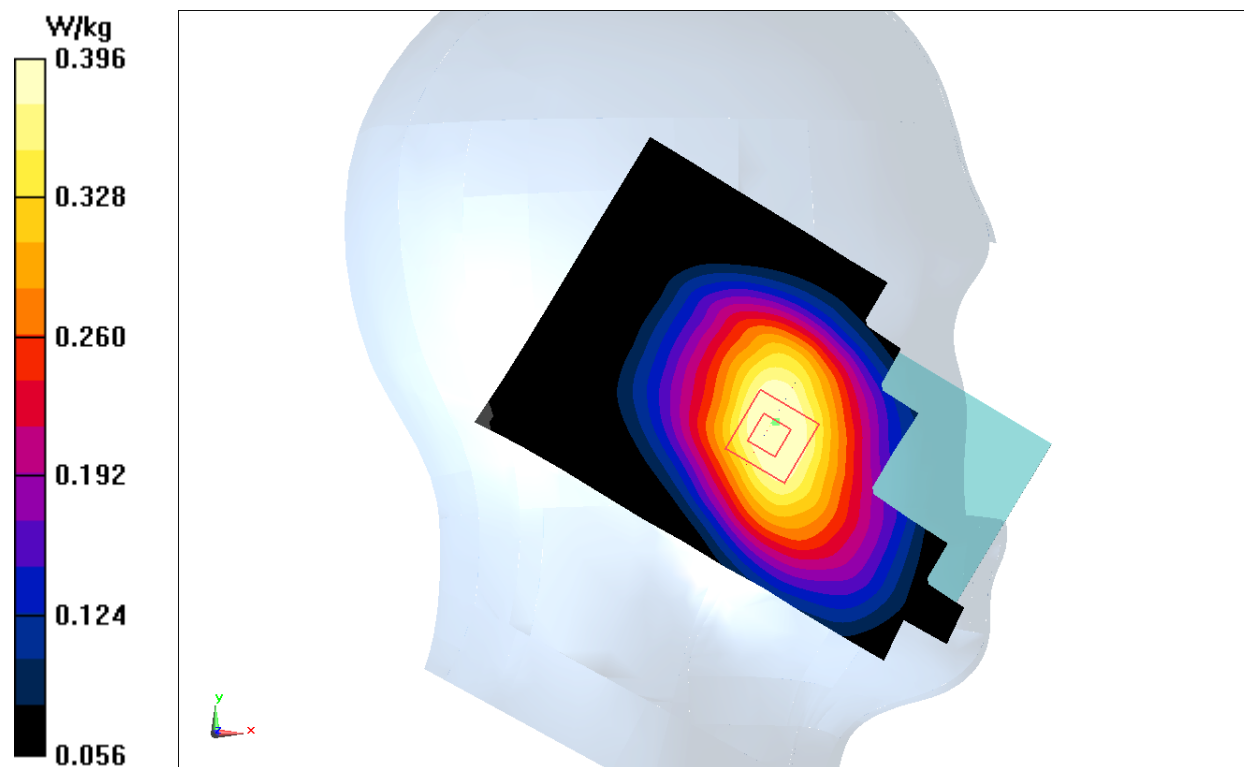
Fig.16 LTE Band 13
