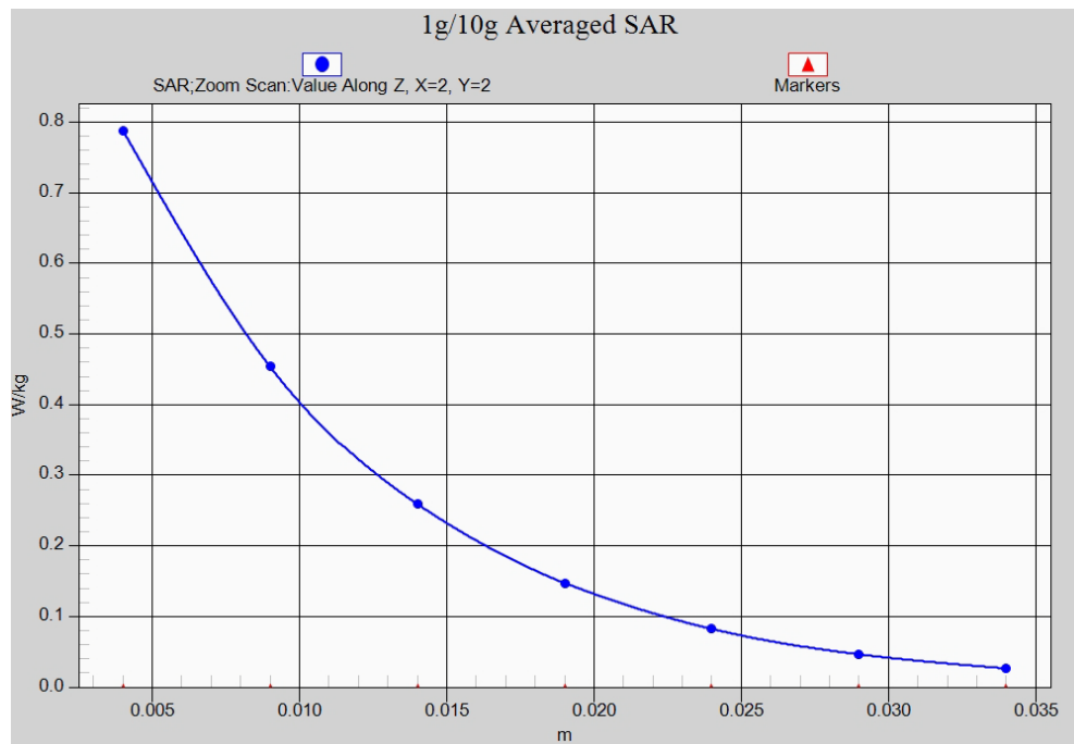
Fig. 14-1 Z-Scan at power reference point (LTE Band7) AP OFF
