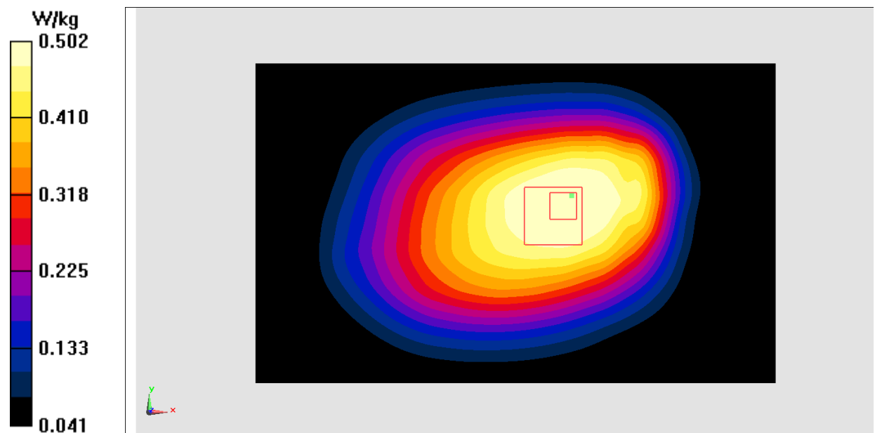
Fig.17 LTE Band 13
