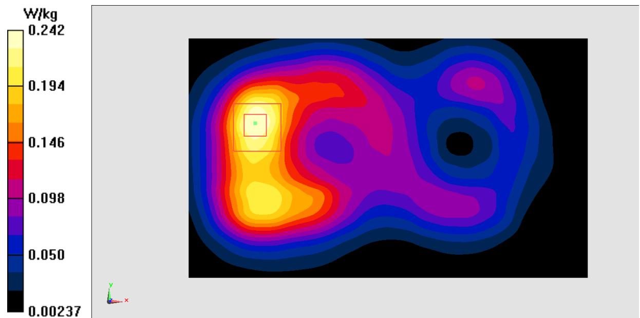
Fig.21 2450 MHz
