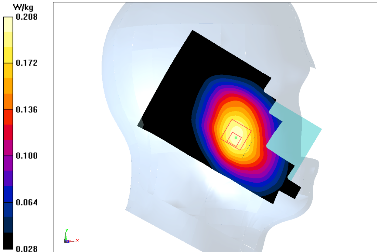
Fig.18 LTE Band17
