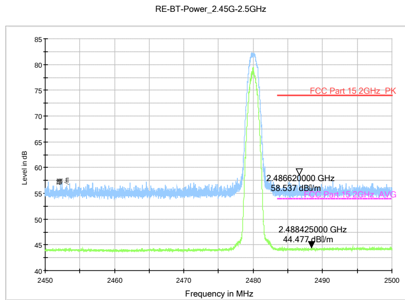
Fig.77. Radiated emission (Power): \pi/4 DQPSK, high channel
