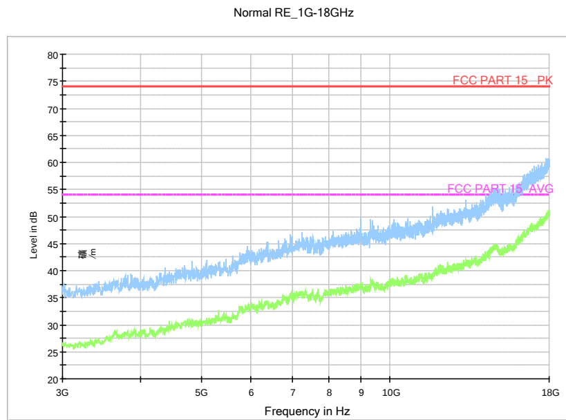
Fig.75. Radiated emission: \pi/4 DQPSK, Channel 78, 3 GHz - 18 GHz
