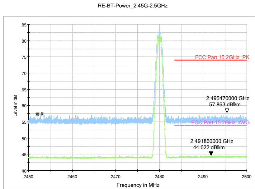
Fig.67. Radiated emission (Power) GFSK, high channel
