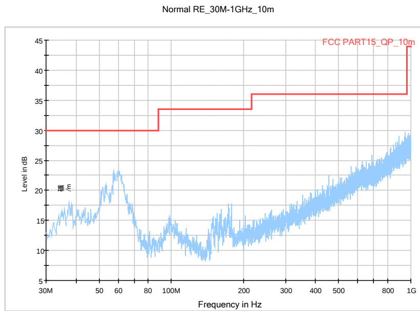
Fig.61. Radiated emission: GFSK, Channel 39, 30 MHz - 1 GHz
