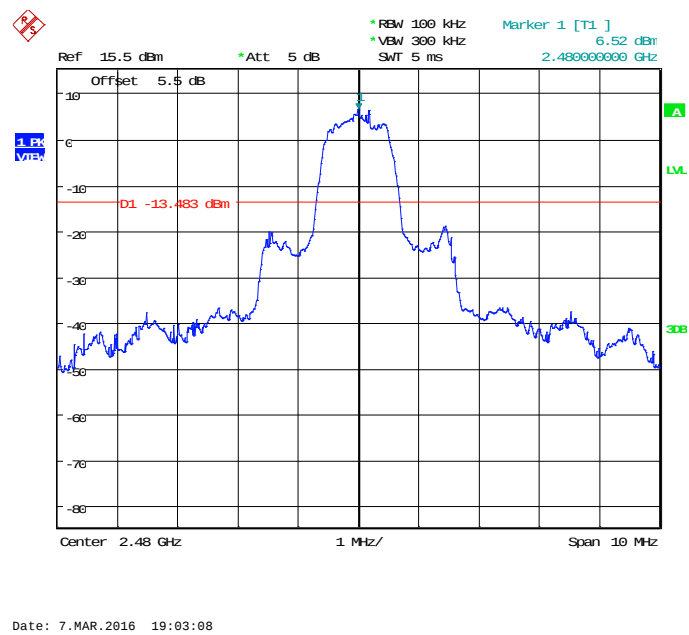
Fig.53. Conducted spurious emission: 8DPSK, Channel 78, 2480MHz
