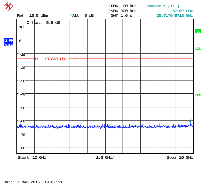
Fig.52. Conducted spurious emission: 8DPSK, Channel 39, 10GHz – 26GHz
