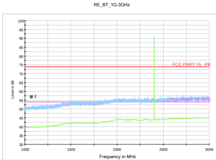
Fig.79. Radiated emission: 8DPSK, Channel 0, 1 GHz - 3 GHz
