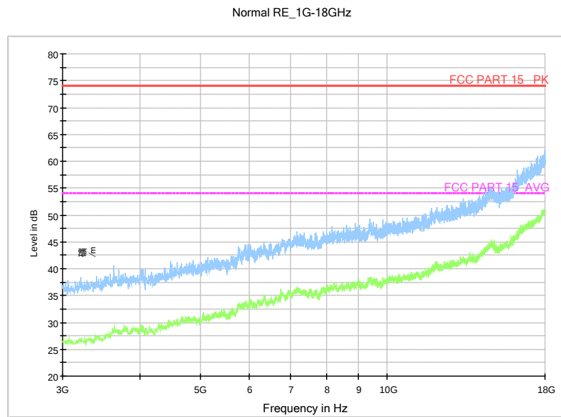
Fig.73. Radiated emission: \pi/4 DQPSK, Channel 39, 3 GHz - 18 GHz
