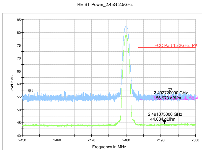
Fig.87. Radiated emission (Power): 8DPSK, high channel
