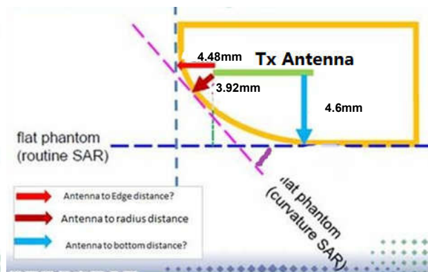
X=4.48 mm, Y=4.6mm, Z=3.92mm Exterior Radius Dimension for WLAN
