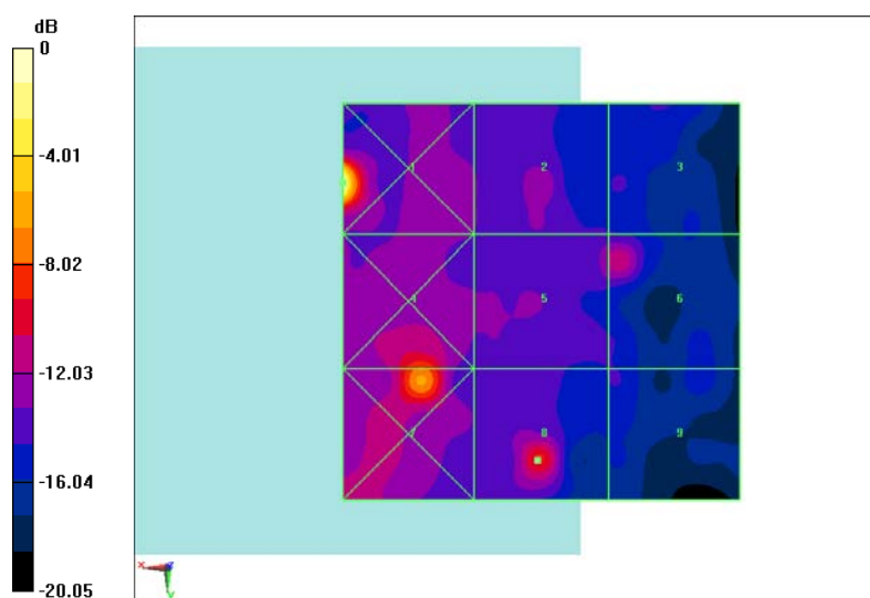
Fig B.14 HAC RF E-Field CDMA 835 Middle
