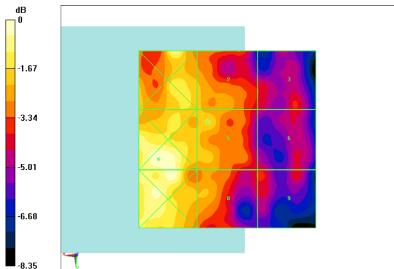
Fig B.9 HAC RF E-Field CDMA 835 Low
