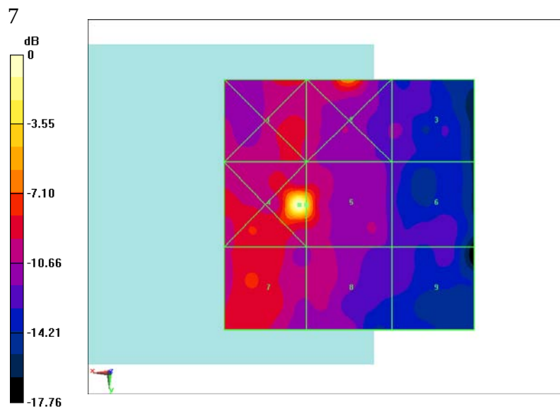
Fig B.11 HAC RF E-Field CDMA 1900 Middle
