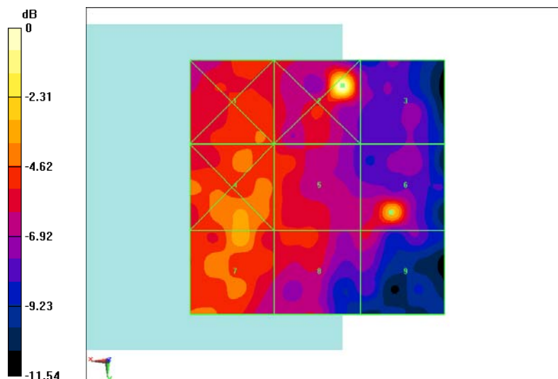
Fig B.15 HAC RF E-Field CDMA 835 Low
