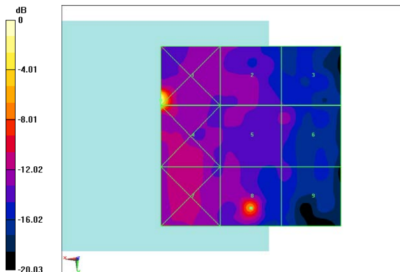
Fig B.10 HAC RF E-Field CDMA 1900 High
