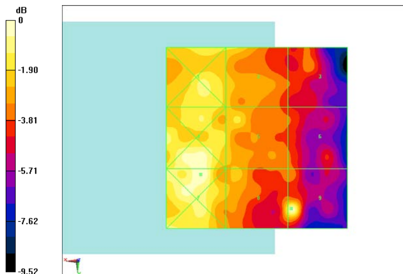
Fig B.12 HAC RF E-Field CDMA 1900 Low
