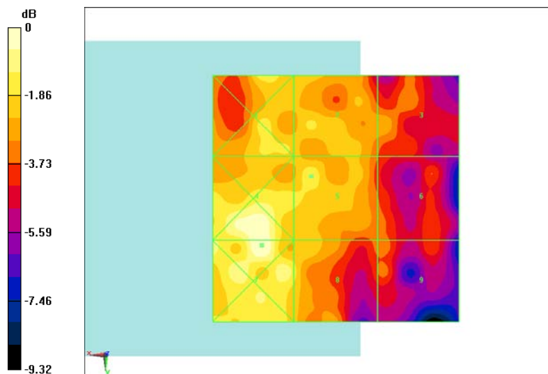
Fig B.8 HAC RF E-Field CDMA 835 Middle
