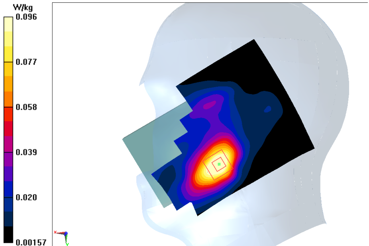
Fig.3 1900 MHz
