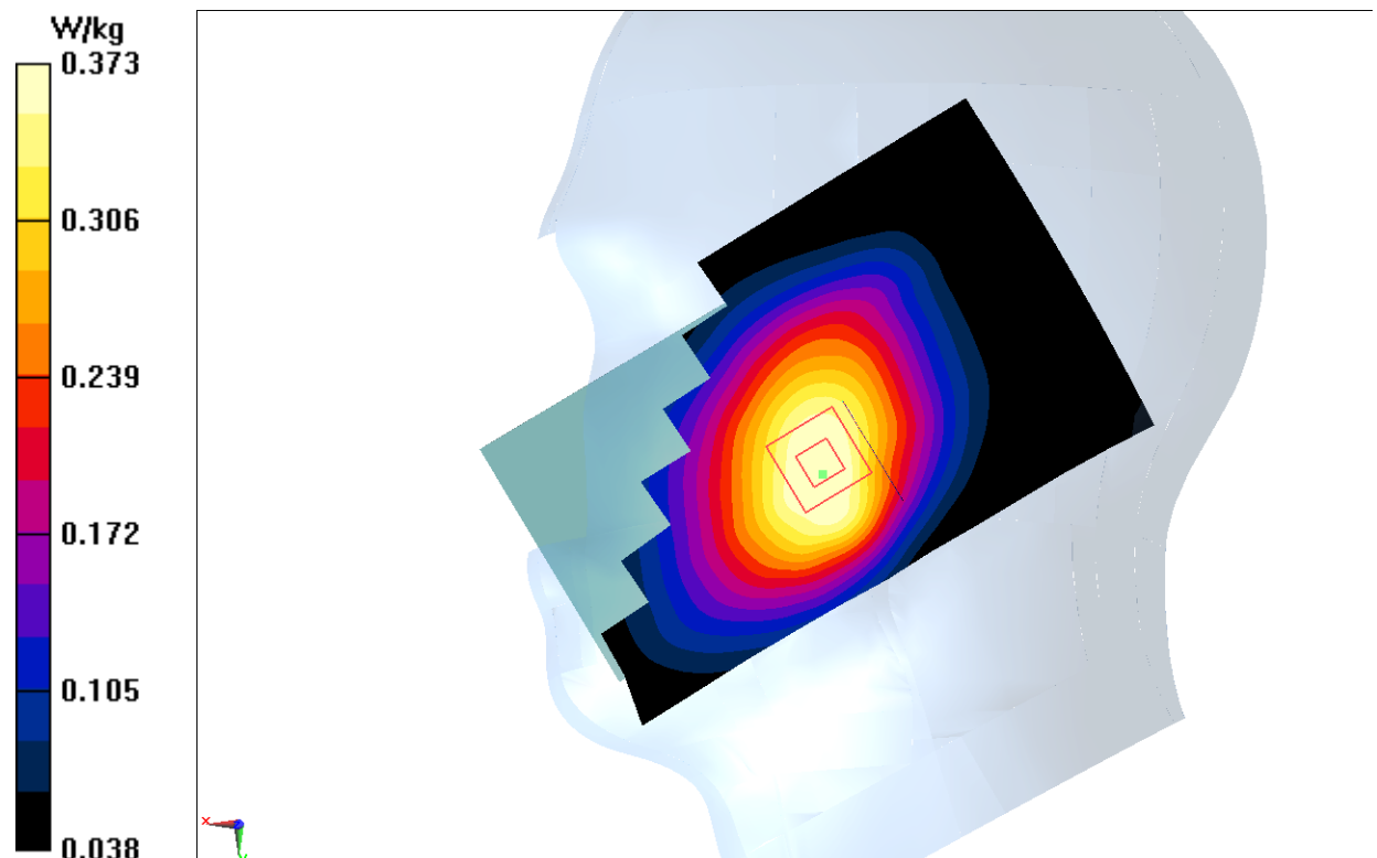
Fig.1 850MHz
