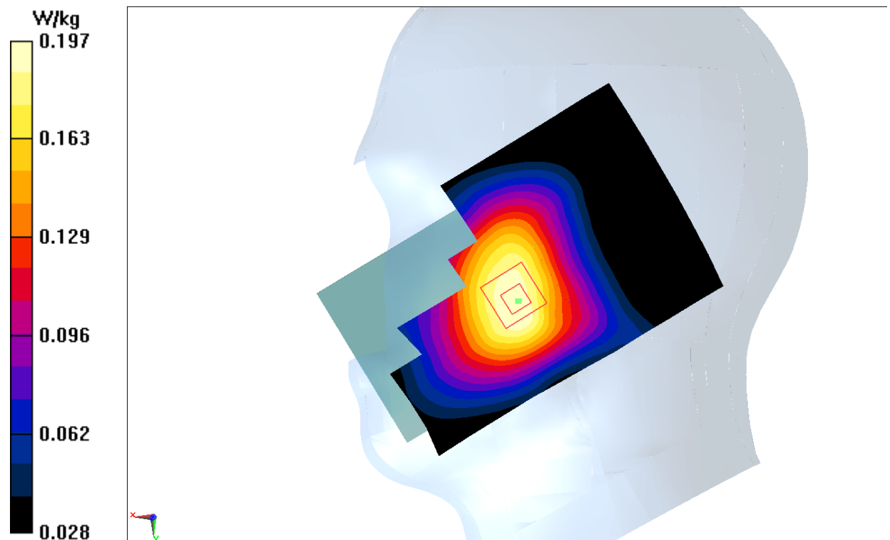
Fig.23 LTE Band12
