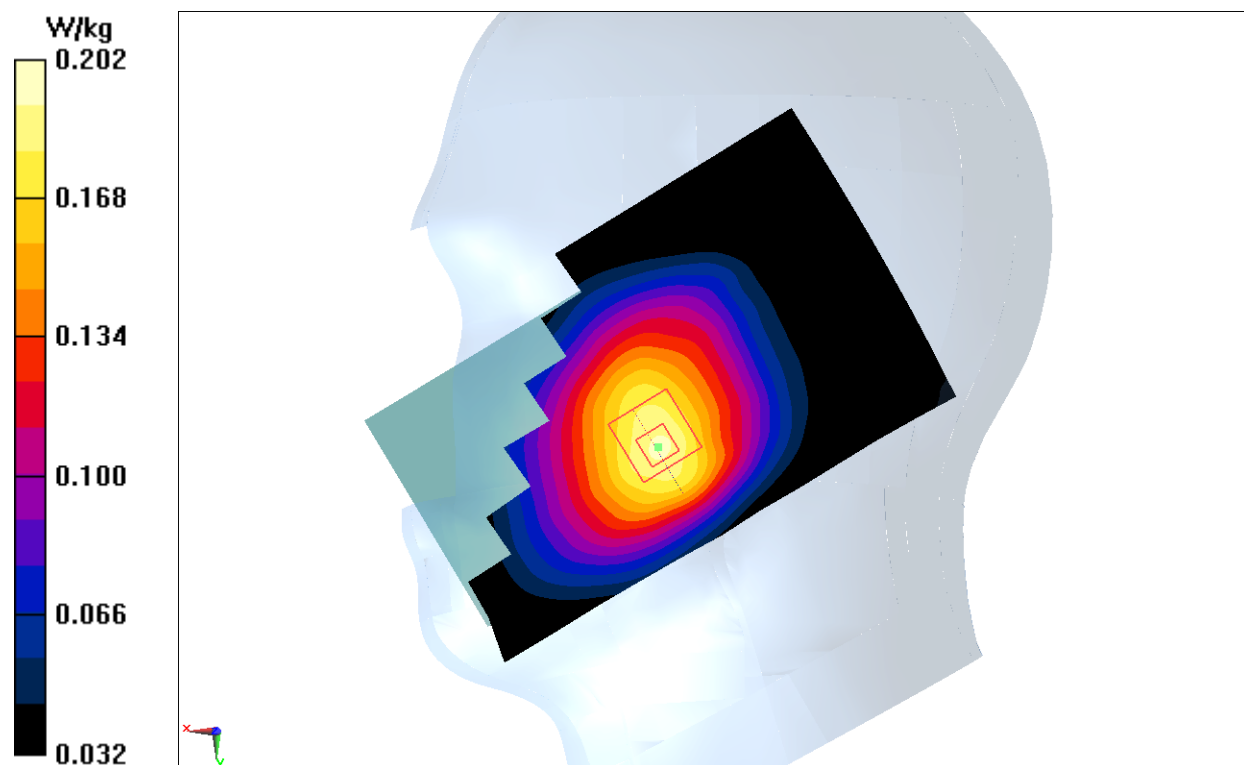
Fig.17 LTE Band17
