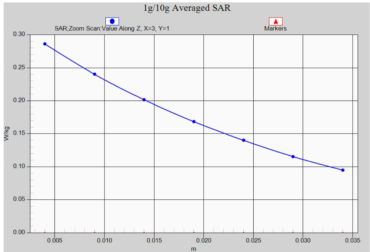
Fig. 24-1 Z-Scan at power reference point (LTE Band12)
