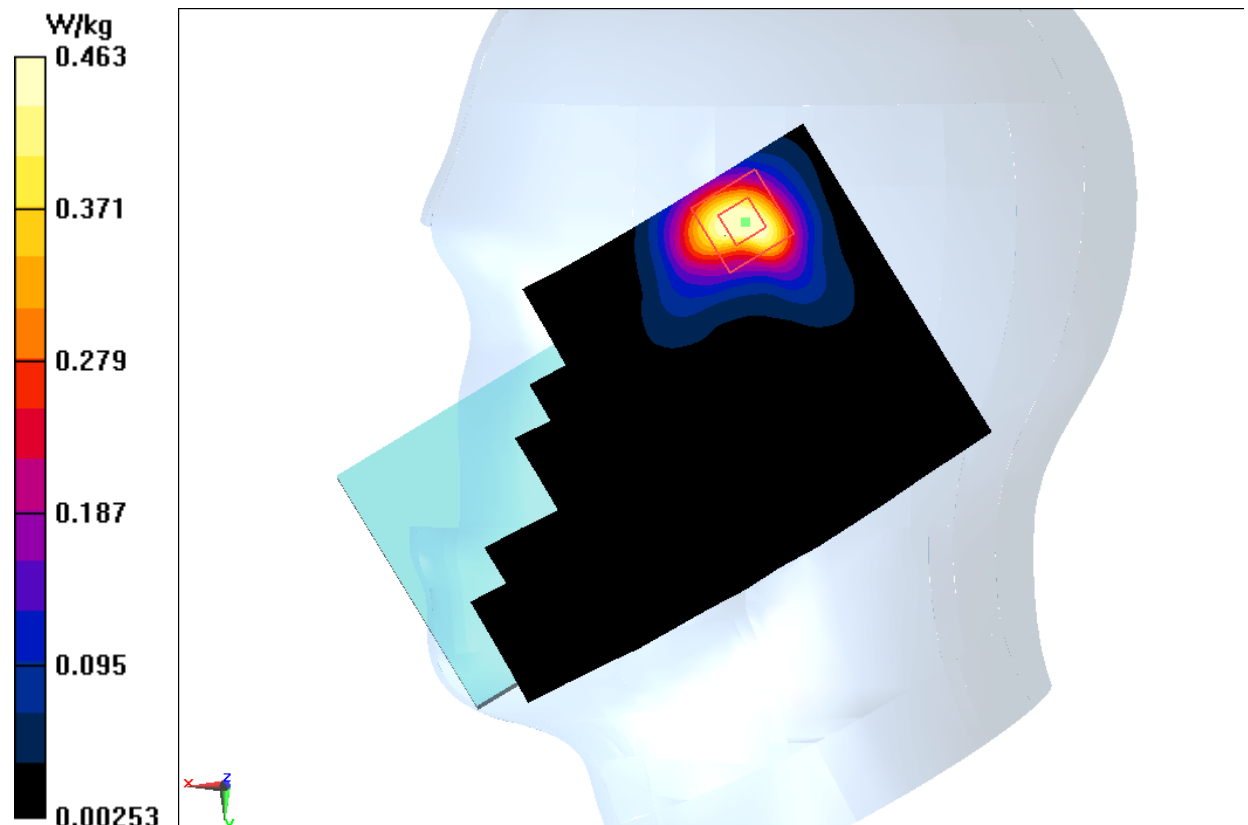
Fig.25 2450 MHz
