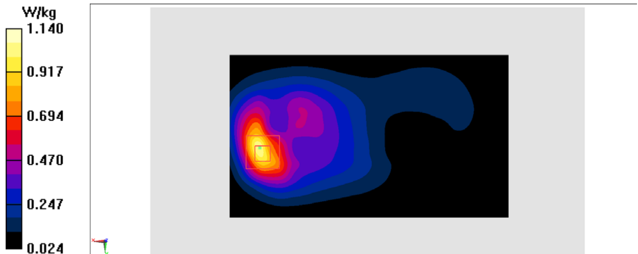
Fig.20 1700 MHz
