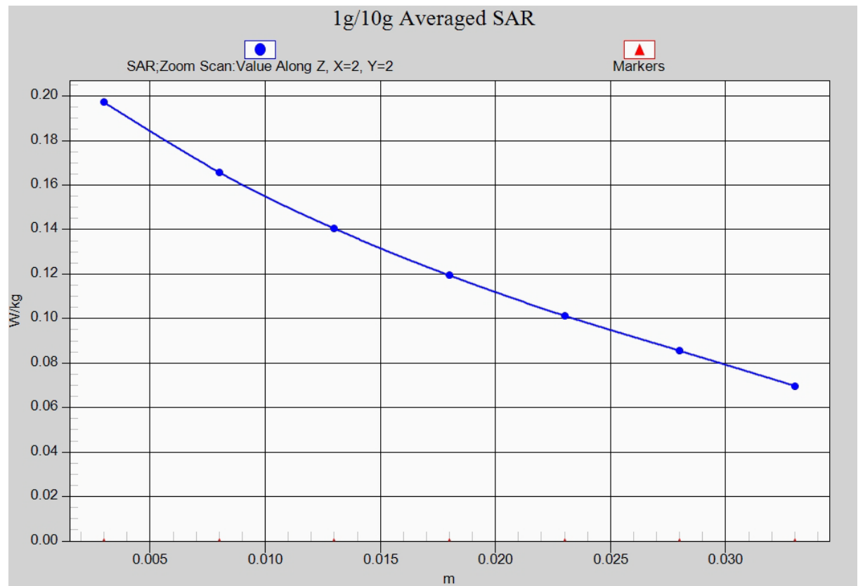
Fig. 23-1 Z-Scan at power reference point (LTE Band12)
