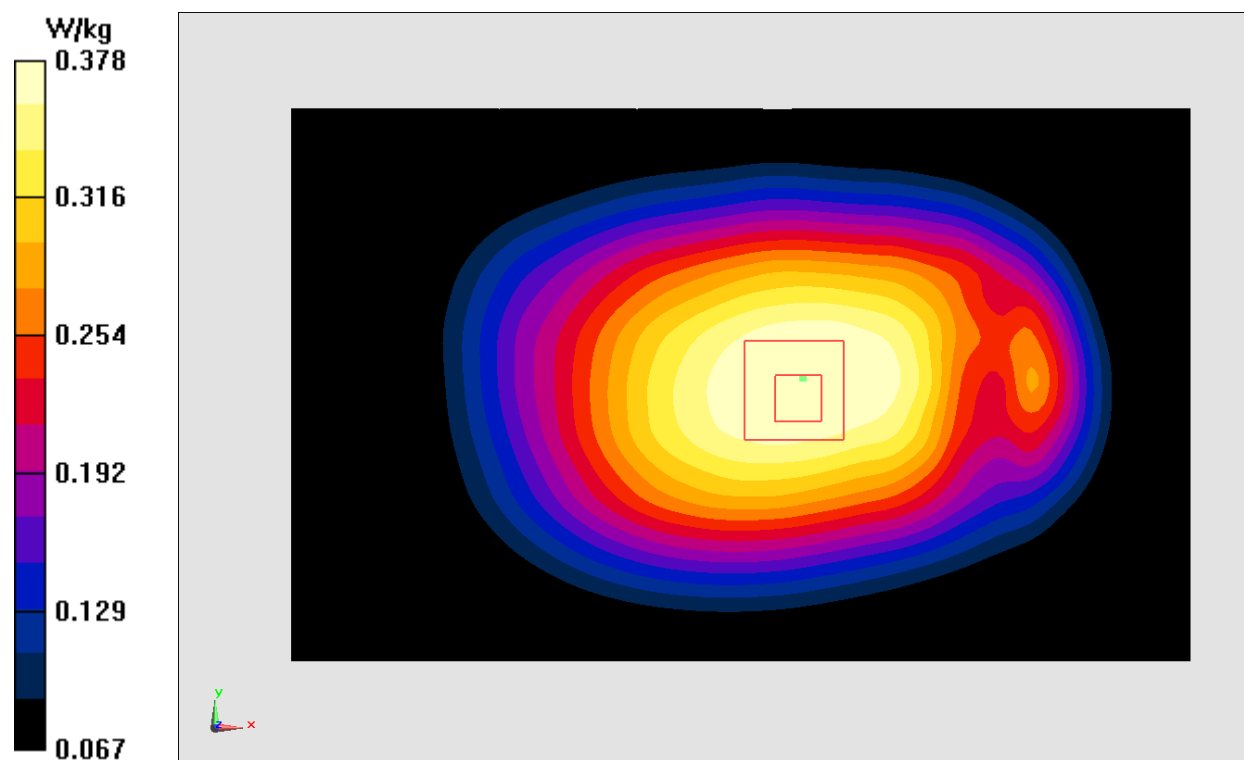
Fig.24 LTE Band12
