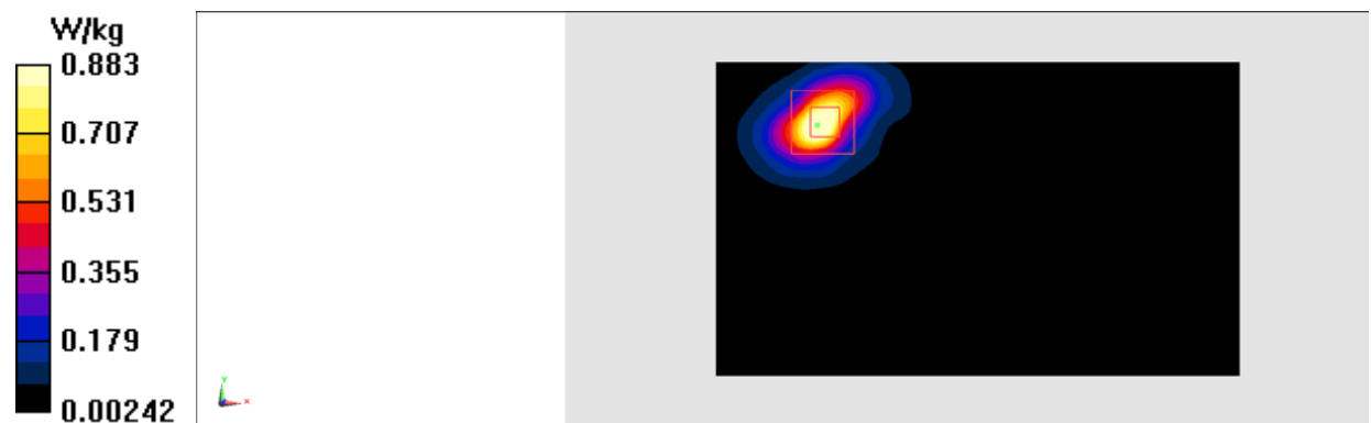
Fig.26 2450 MHz
