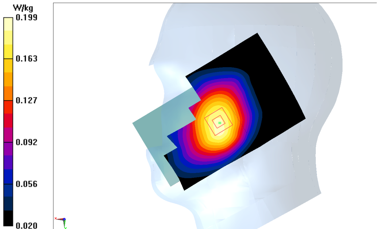
Fig.17 LTE Band17
