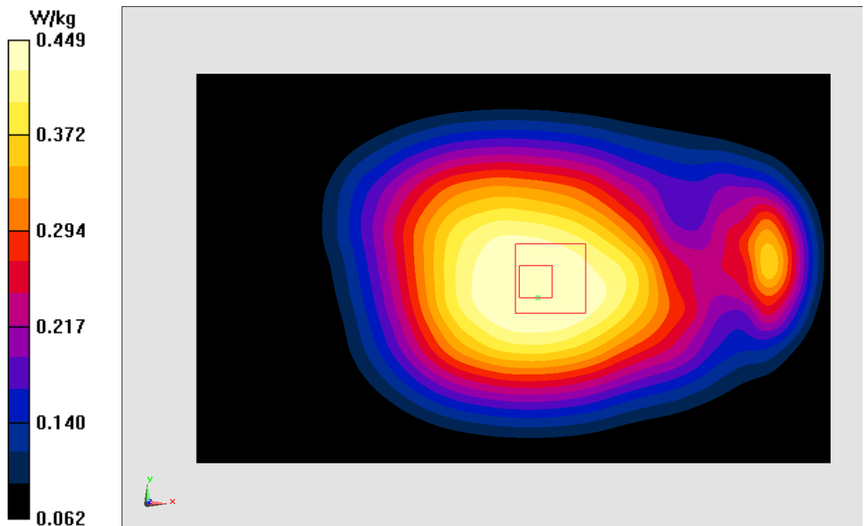
Fig.22 LTE Band5
