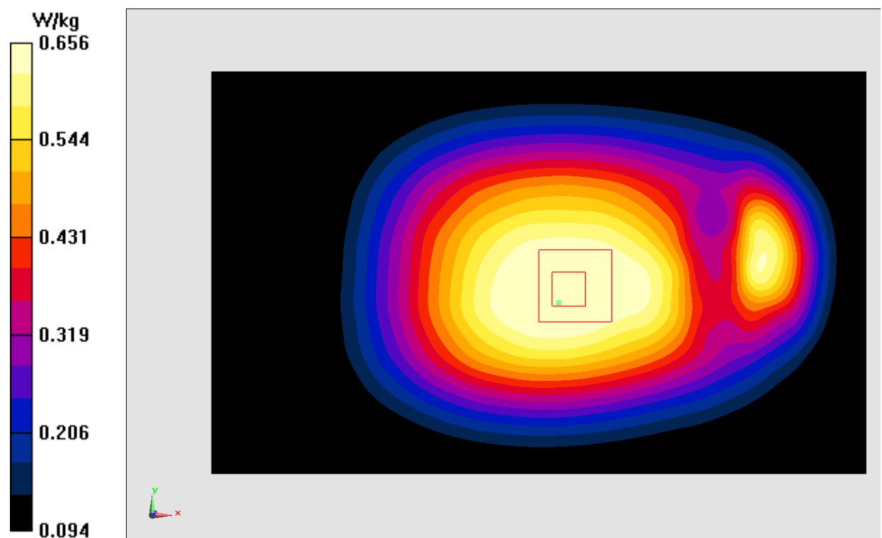
Fig.2 850 MHz
