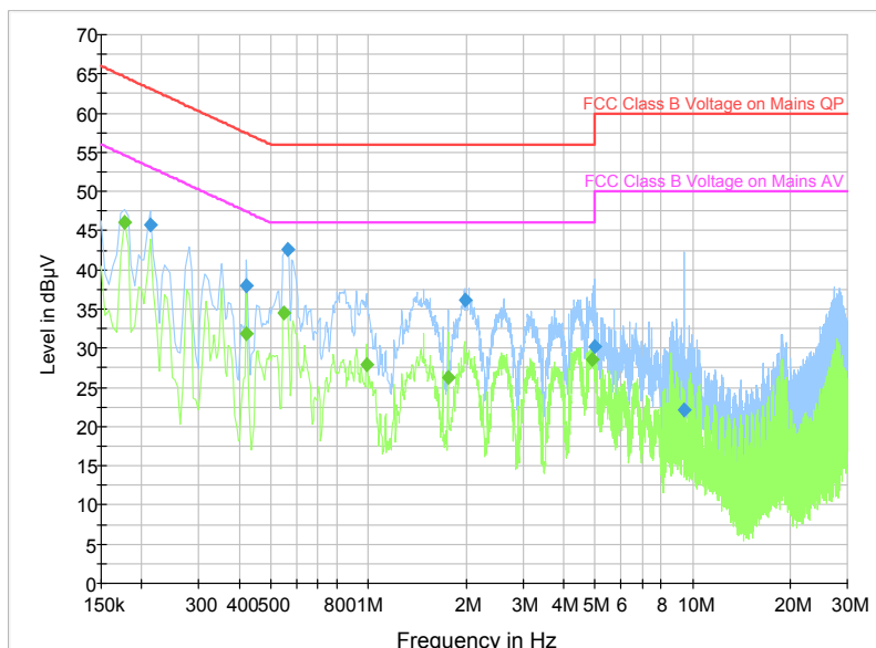
Figure A.9 Conducted Emission
