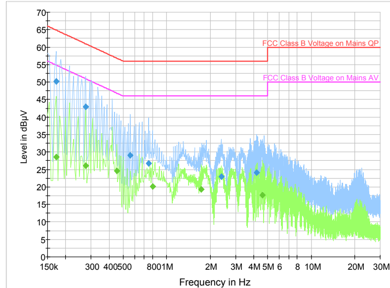
Figure A.7 Conducted Emission
