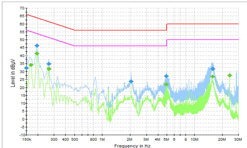
Fig.12 Conducted Emission
