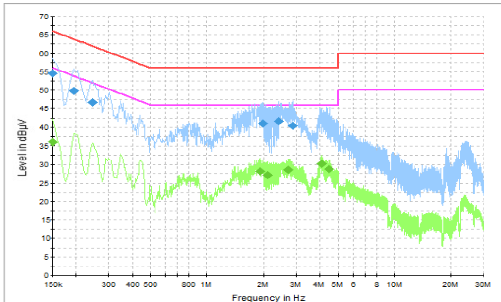
Fig.11 Conducted Emission
