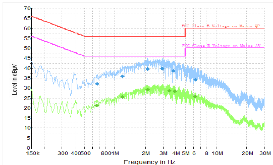
Fig.12 Conducted Emission
