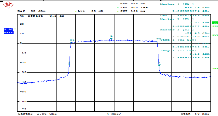
(Channel Bandwidth:20 MHz) LCH_QPSK_100RB#0
