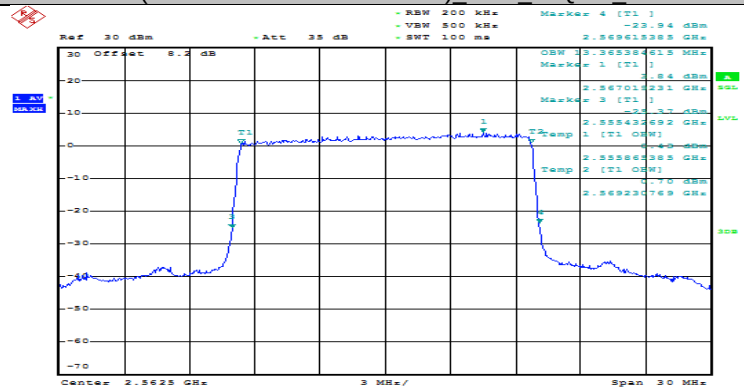
(Channel Bandwidth:15 MHz) HCH_16QAM_75RB#0
