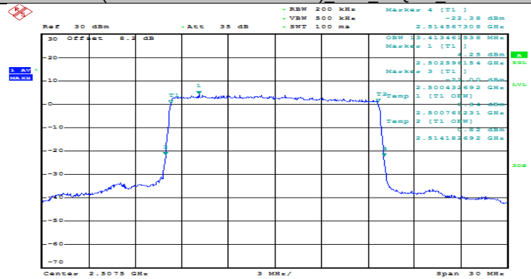
(Channel Bandwidth:15 MHz) LCH_16QAM_75RB#0
