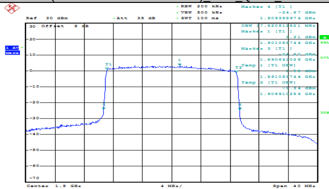
(Channel Bandwidth:20 MHz) HCH_QPSK_100RB#0
