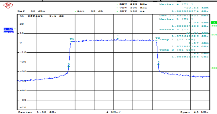
(Channel Bandwidth:20 MHz) MCH_QPSK_100RB#0
