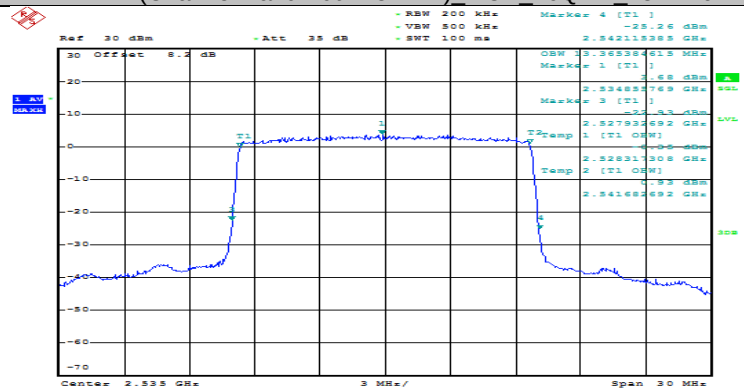
(Channel Bandwidth:15 MHz) MCH_16QAM_75RB#0
