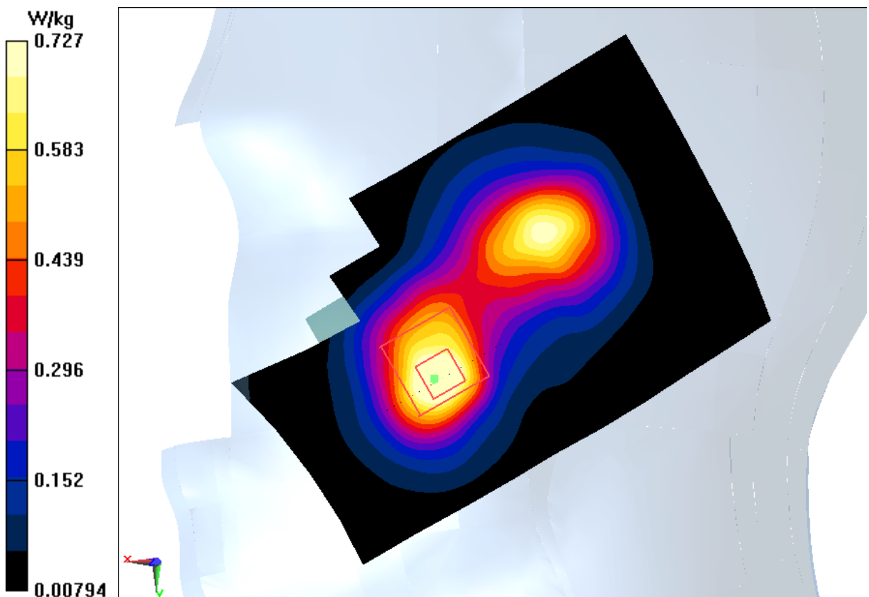
Fig.I.3 1900 MHz
