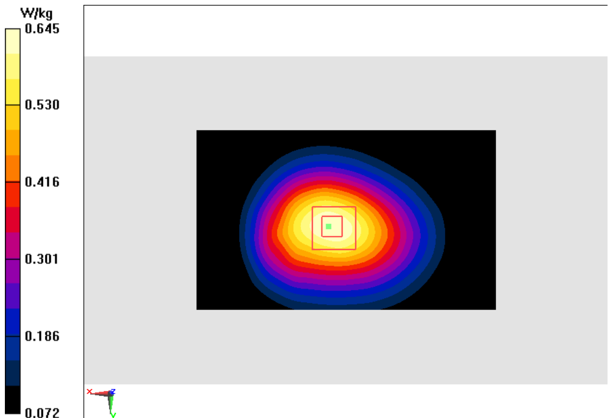
Fig.I.2 850 MHz
