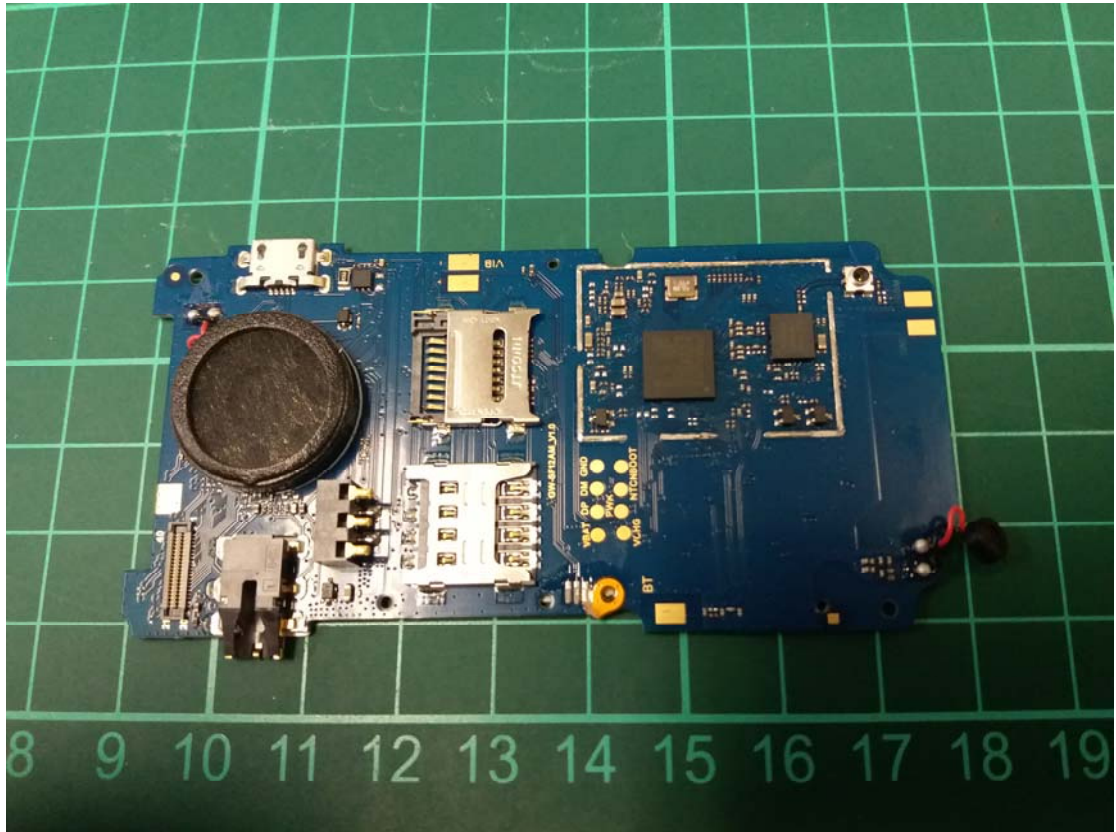
2053X Mobile Phone Disassembly
