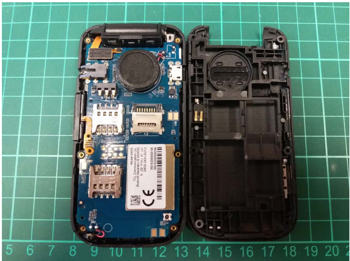
2053D Mobile Phone
