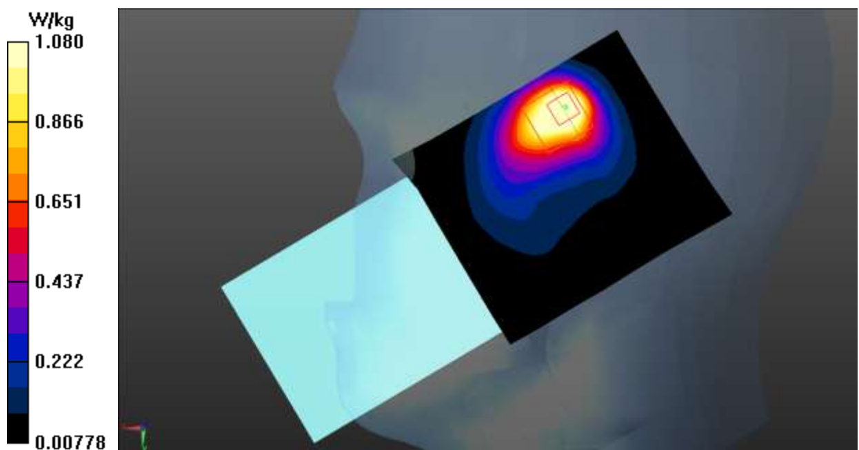
Fig.3 GSM 1900 Head
