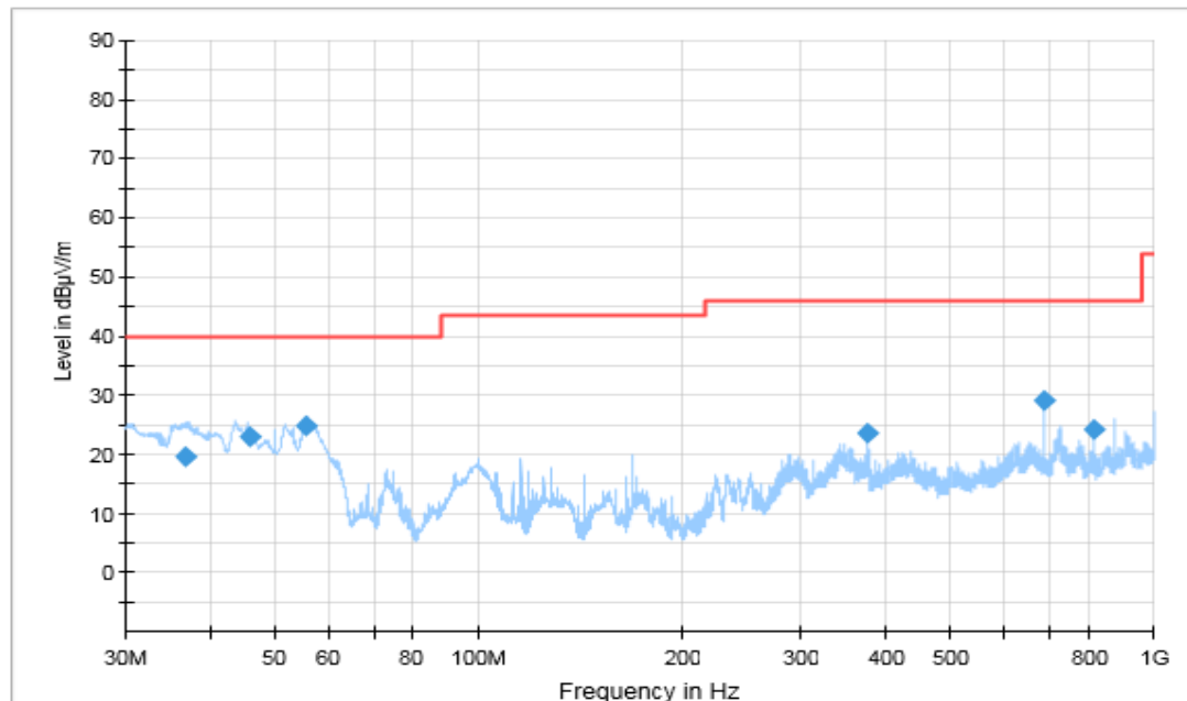
Figure A.13 Radiated Emission (Set.1,FM Mode, 30MHz to 1GHz)
