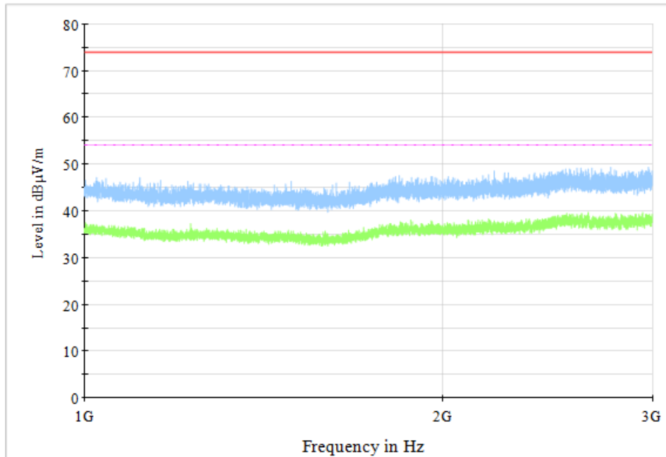
Figure A.20 Radiated Emission (Set.3, Data Transfer Mode/PC to EUT, 1GHz to 3GHz)
