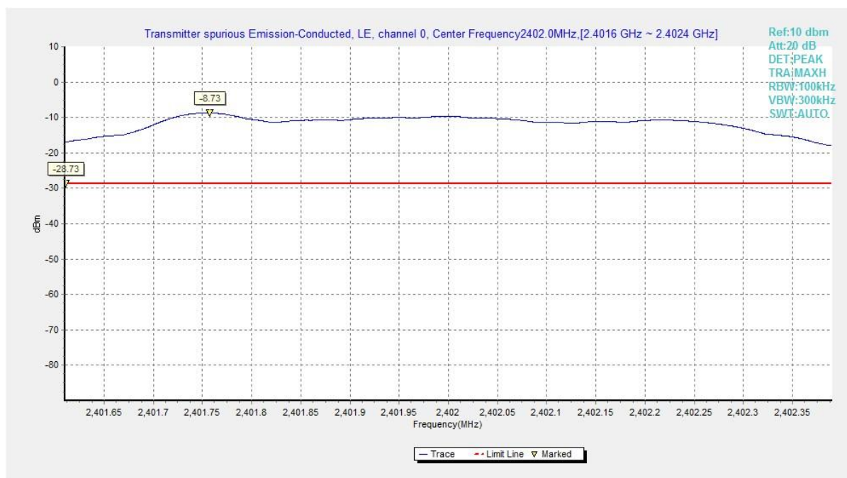
Fig.9 Conducted Spurious Emission (Ch0, Center Frequency), LE 1M
