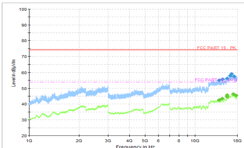
Figure A.26 Radiated Emission (Set.3, Data Transfer : TF Card to PC, 1GHz to 18GHz) Final_Results_PK
