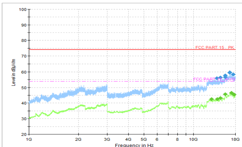
Figure A.22 Radiated Emission (Set.3, Data Transfer: PC to EUT, 1GHz to 18GHz)
