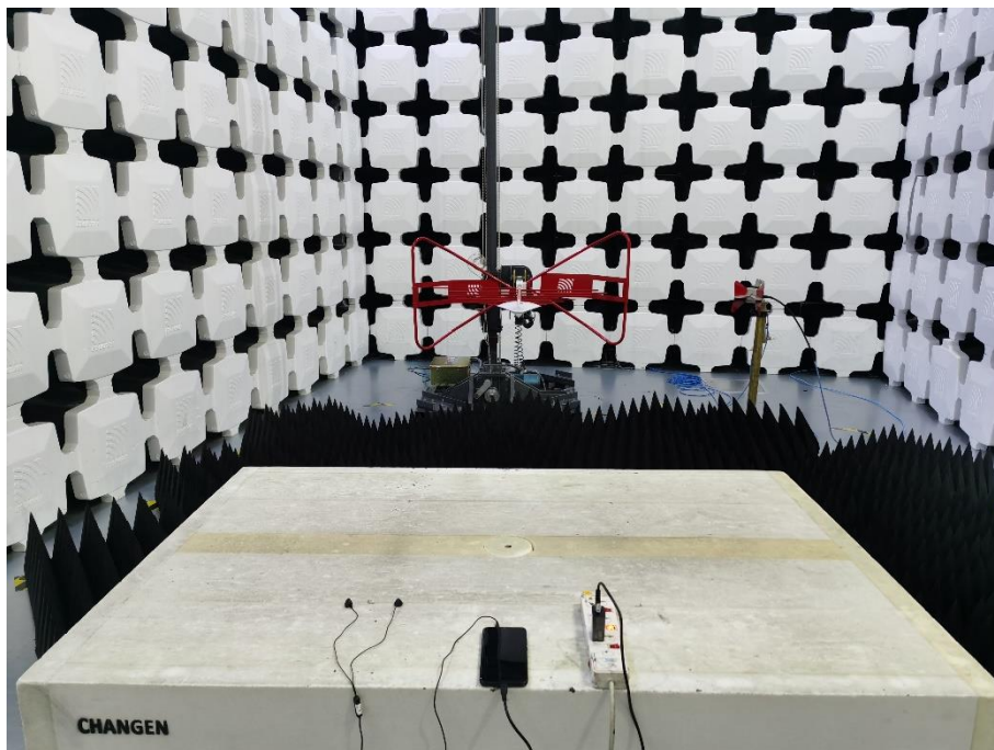
6. Radiated Emissions (Part 15B Charging Mode with FM Mode, 1GHz-18GHz)
