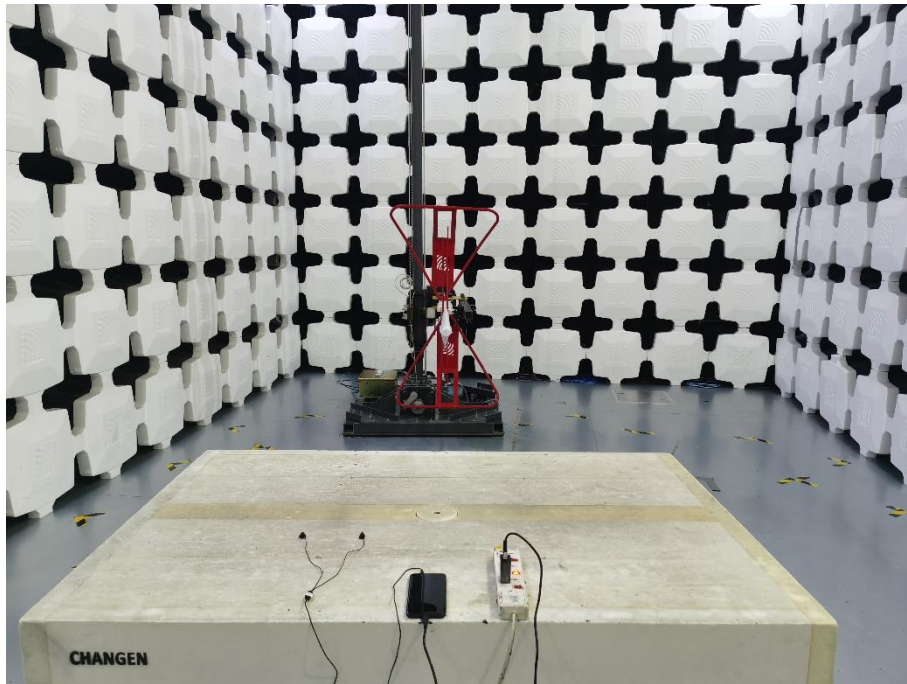
5. Radiated Emissions (Part 15B Charging Mode with FM Mode, 30MHz-1GHz)
