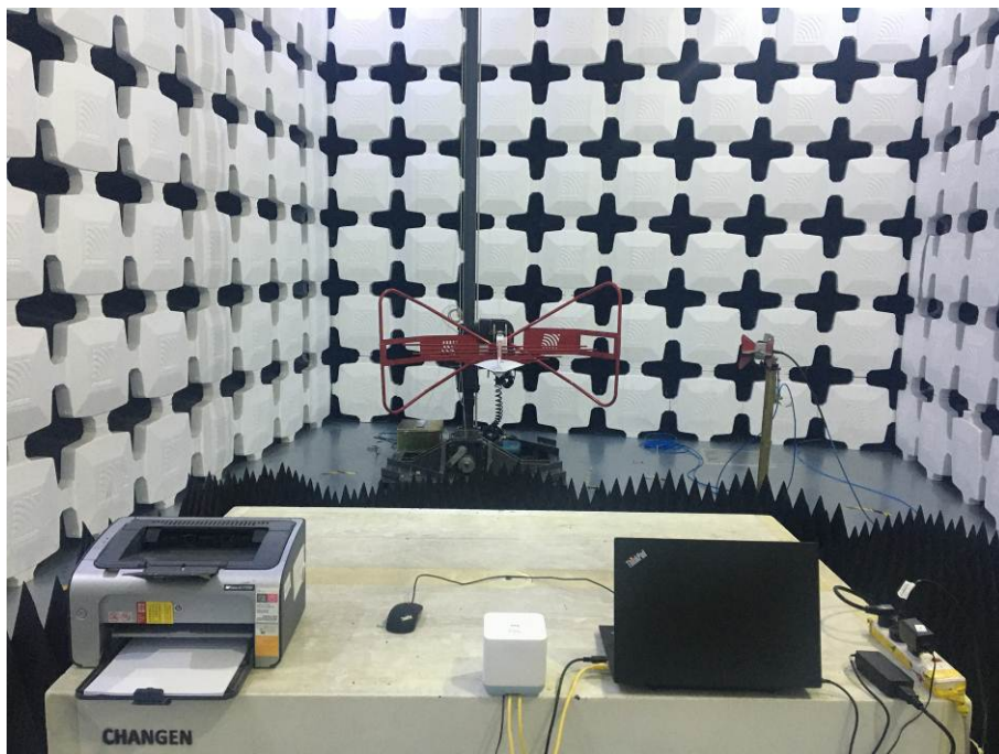
2. Radiated Emissions (Part 15B, 1GHz-18GHz)
