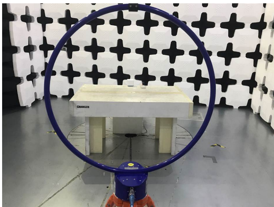
4. Radiated Emissions (Part 15C&15E) (9kHz-30MHz)
