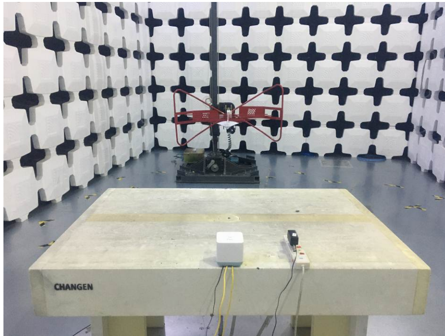
5. Radiated Emissions (Part 15C&15E) (30MHz-1GHz)
