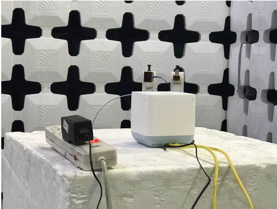
7. Radiated Emissions (Part 15C&15E) (18-40GHz)
