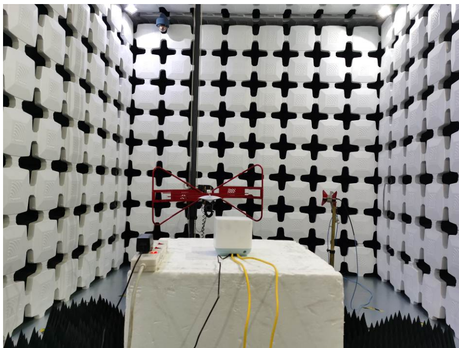
6. Radiated Emissions (Part 15C&15E) (1-18GHz)
