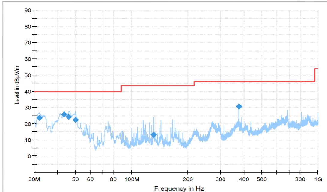
Figure A.4 Radiated Emission (Set.1, Charging and WCDMA Band 5 idle, 30MHz to 1GHz) Final_Result
