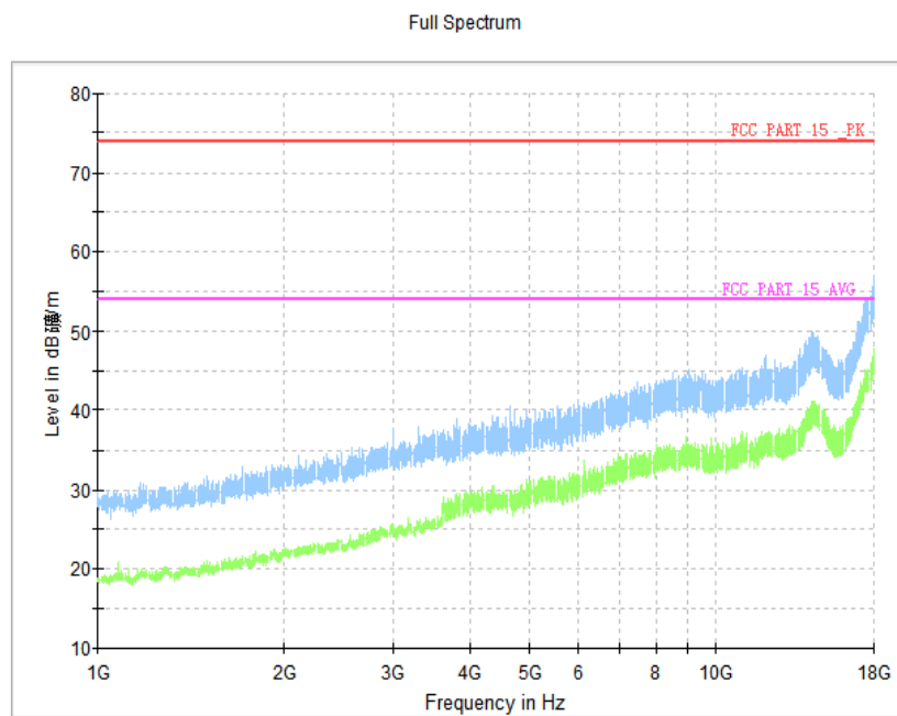
Figure A.4 Radiated Emission from 1GHz to 18GHz
