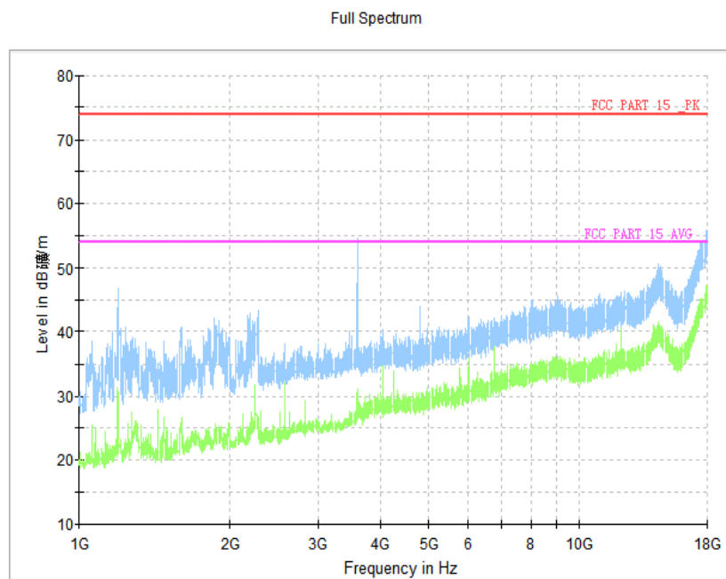
Figure A.6 Radiated Emission from 1GHz to 18GHz
