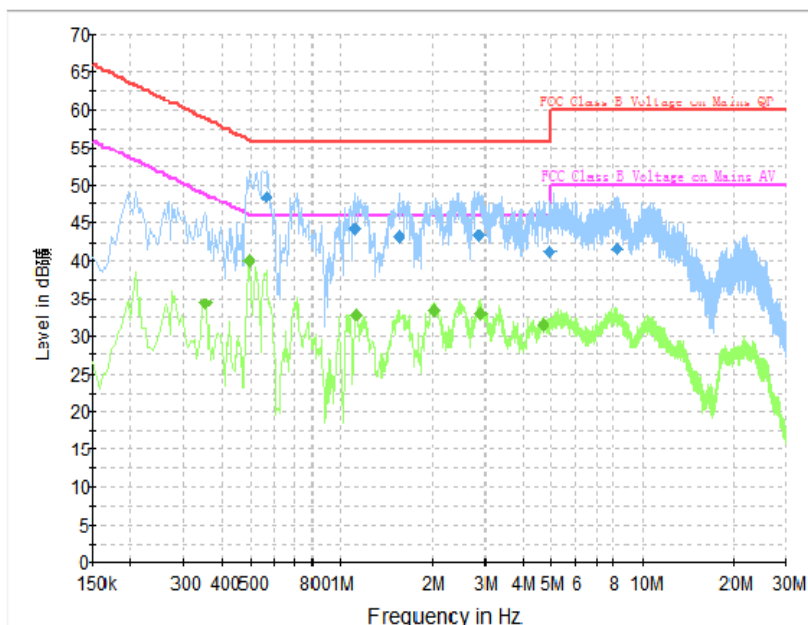
Figure A.11 Conducted Emission
