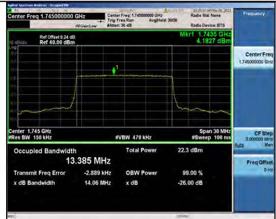
Band66-15MHz-QPSK-132322-75RB#0-13.385
