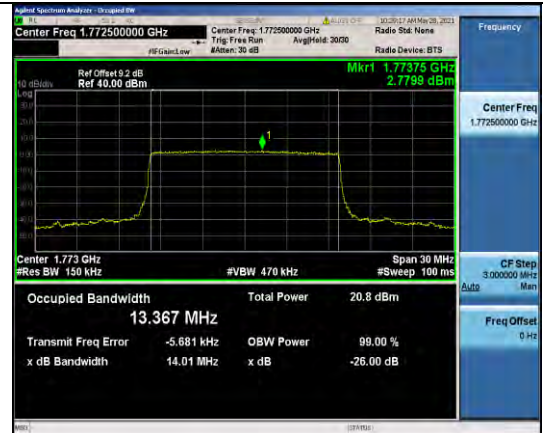
Band66-15MHz-16QAM-132597-75RB#0-13.367
