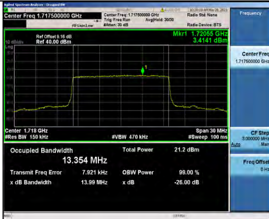
Band66-15MHz-16QAM-132047-75RB#0-13.354
