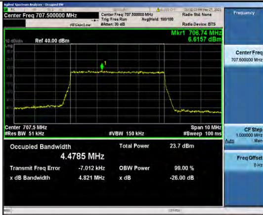
Band12-5MHz-QPSK-23095-25RB#0-4.4785
