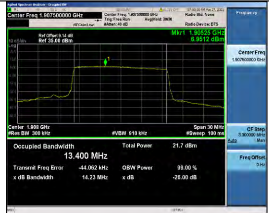
Band25-15MHz-QPSK-26615-75RB#0-13.400
