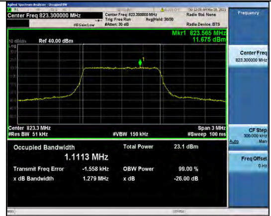
Band26-1.4MHz-QPSK-26783-6RB#0-1.1113
