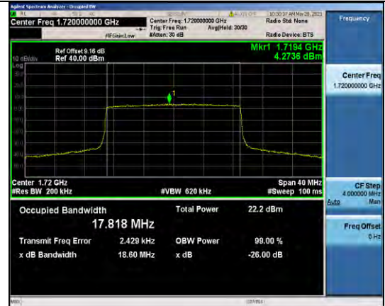
Band66-20MHz-QPSK-132072-100RB#0-17.818
