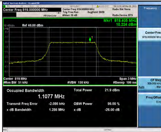
Band26-1.4MHz-16QAM-26740-6RB#0-1.1077
