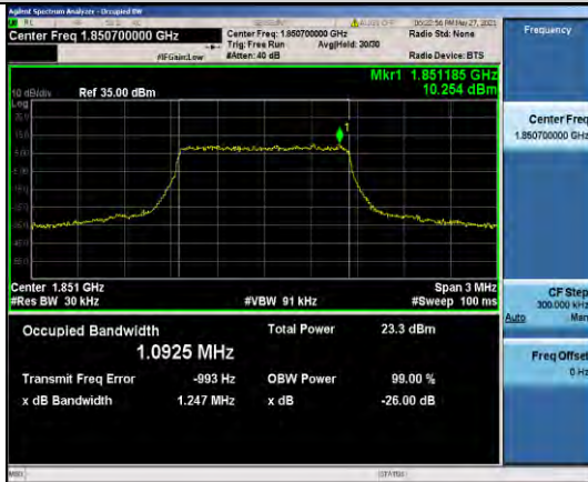
Band25-1.4MHz-QPSK-26047-6RB#0-1.0925
