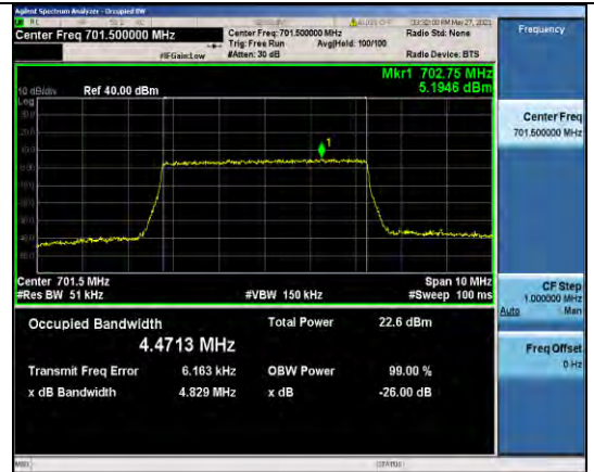
Band12-5MHz-16QAM-23035-25RB#0-4.4713
