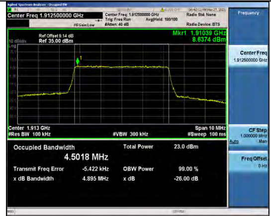
Band25-5MHz-QPSK-26665-25RB#0-4.5018
