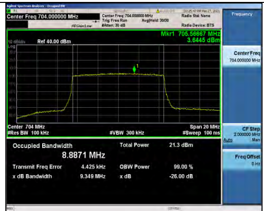
Band12-10MHz-16QAM-23060-50RB#0-8.8871
