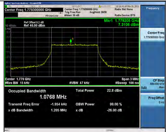
Band66-1.4MHz-16QAM-132665-6RB#0-1.0768
