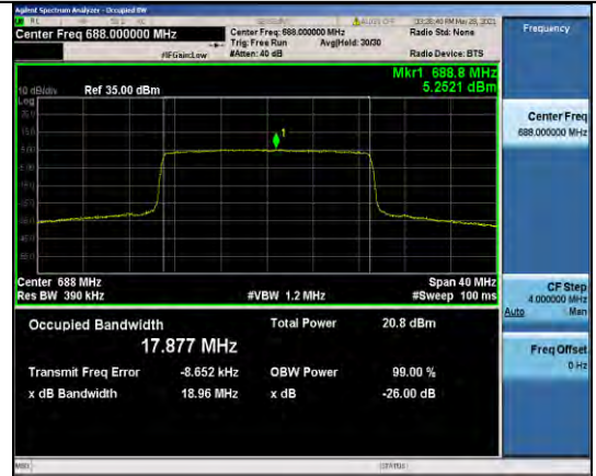
Band71-20MHz-16QAM-133372-100RB#0-17.877
