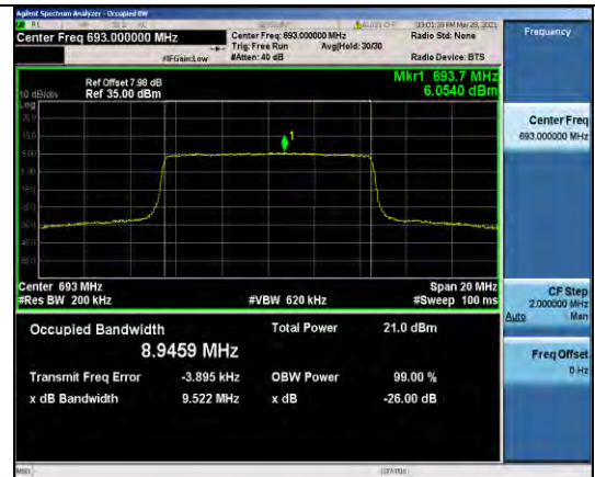
Band71-10MHz-16QAM-133422-50RB#0-8.9459
