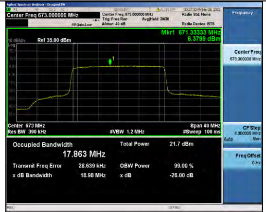
Band71-20MHz-QPSK-133222-100RB#0-17.863
