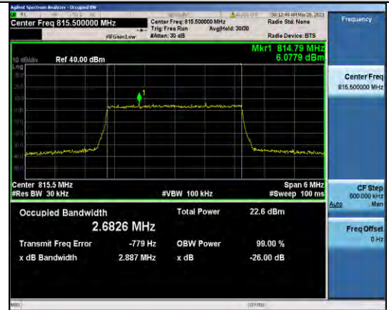
Band26-3MHz-16QAM-26705-15RB#0-2.6826
