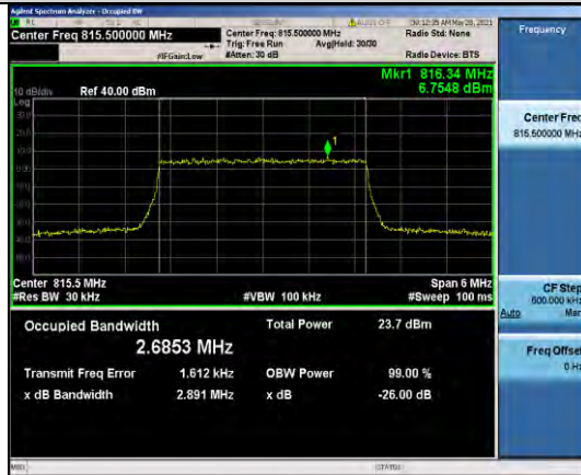
Band26-3MHz-QPSK-26705-15RB#0-2.6853
