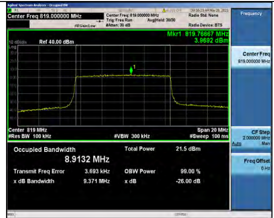
Band26-10MHz-16QAM-26740-50RB#0-8.9132
