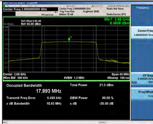
Band41-20MHz-QPSK-41490-100RB#0-17.893
