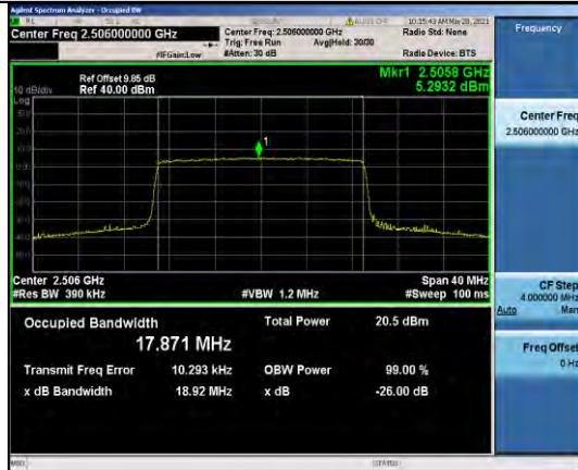
Band41-20MHz-16QAM-39750-100RB#0-17.871
