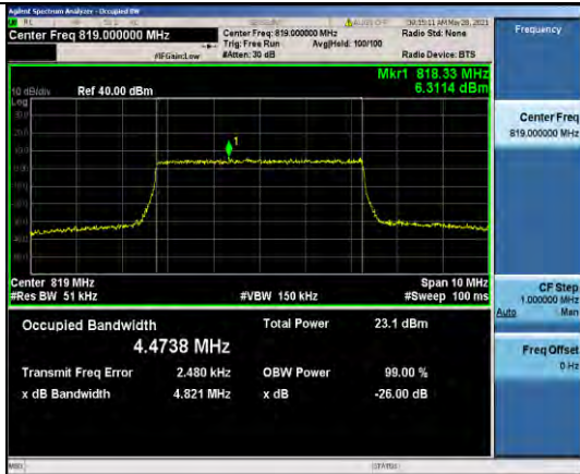
Band26-5MHz-16QAM-26740-25RB#0-4.4738
