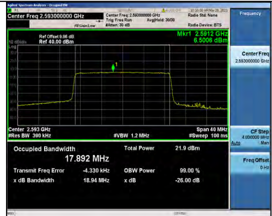
Band41-20MHz-QPSK-40620-100RB#0-17.892
