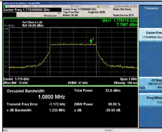
Band66-1.4MHz-QPSK-132665-6RB#0-1.0800
