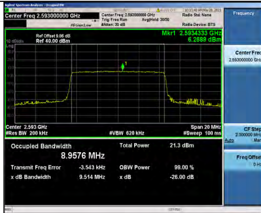
Band41-10MHz-16QAM-40620-50RB#0-8.9576
