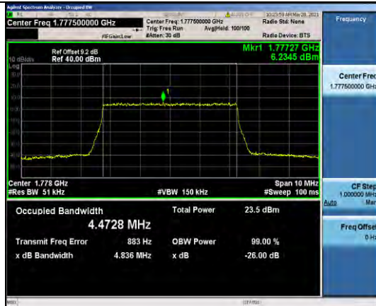
Band66-5MHz-QPSK-132647-25RB#0-4.4728
