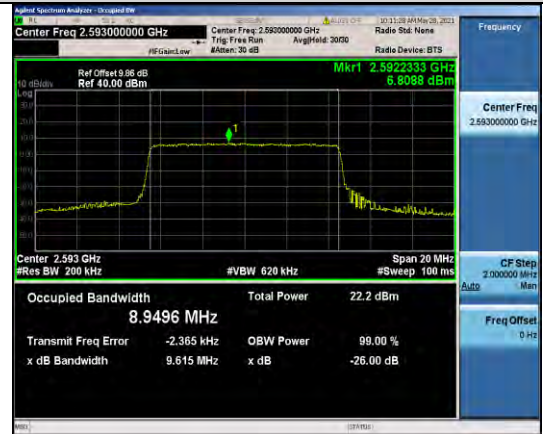
Band41-10MHz-QPSK-40620-50RB#0-8.9496
