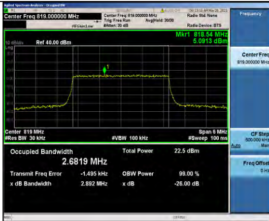
Band26-3MHz-16QAM-26740-15RB#0-2.6819
