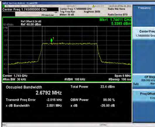
Band66-3MHz-16QAM-132322-15RB#0-2.6792
