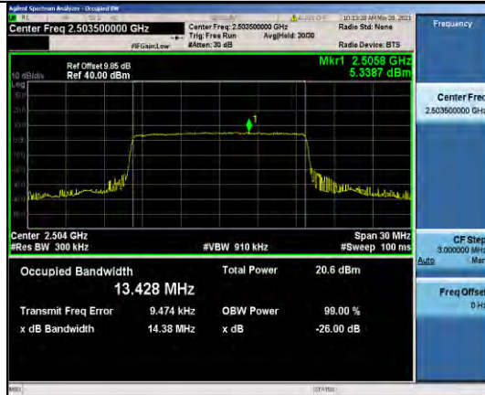
Band41-15MHz-16QAM-39725-75RB#0-13.428
