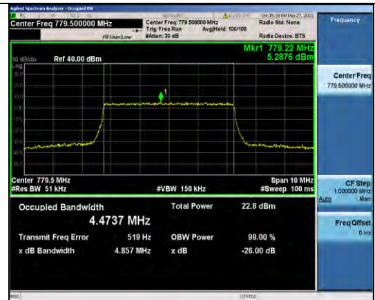
Band13-5MHz-16QAM-23205-25RB#0-4.4737
