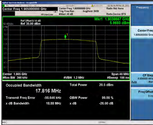
Band25-20MHz-16QAM-26590-100RB#0-17.816
