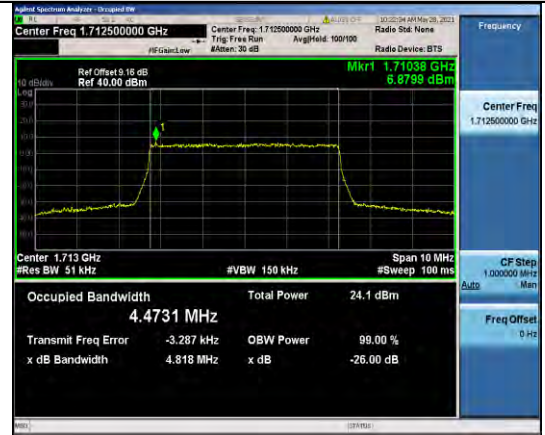
Band66-5MHz-QPSK-131997-25RB#0-4.4731
