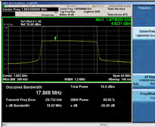
Band25-20MHz-16QAM-26365-100RB#0-17.868
