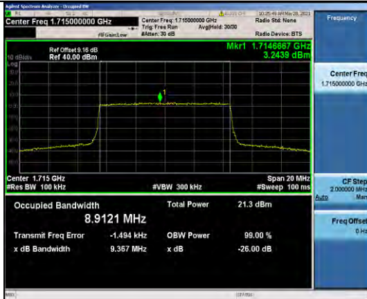
Band66-10MHz-16QAM-132022-50RB#0-8.9121
