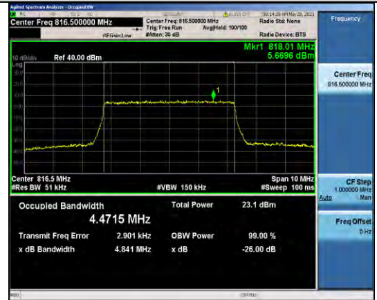
Band26-5MHz-16QAM-26715-25RB#0-4.4715
