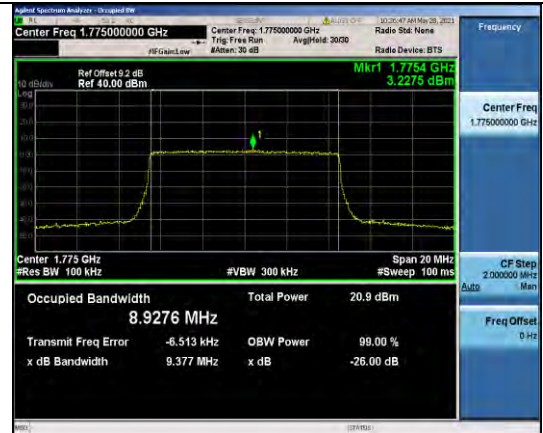
Band66-10MHz-16QAM-132622-50RB#0-8.9276
