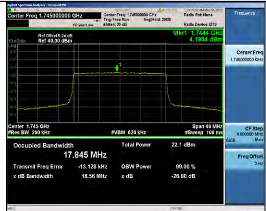
Band66-20MHz-QPSK-132322-100RB#0-17.845
