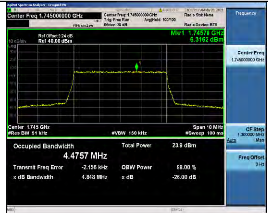
Band66-5MHz-QPSK-132322-25RB#0-4.4757
