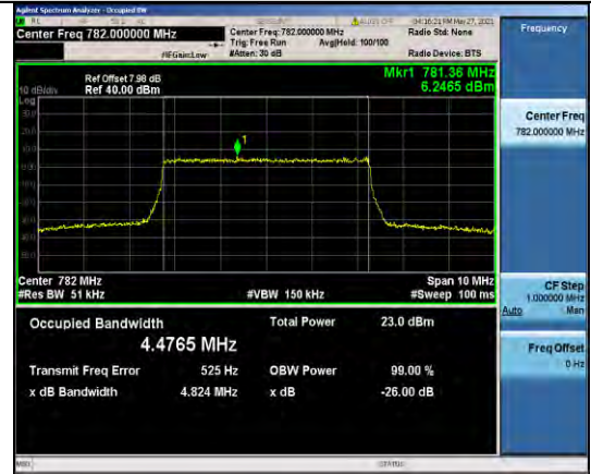
Band13-5MHz-16QAM-23230-25RB#0-4.4765
