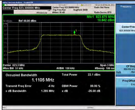
Band26-1.4MHz-16QAM-26783-6RB#0-1.1105
