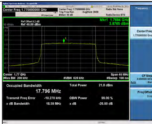
Band66-20MHz-QPSK-132572-100RB#0-17.796
