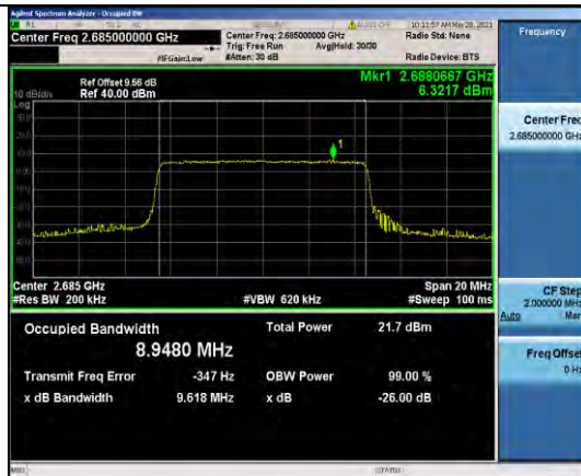
Band41-10MHz-QPSK-41540-50RB#0-8.9480
