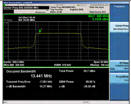
Band71-15MHz-16QAM-133397-75RB#0-13.441
