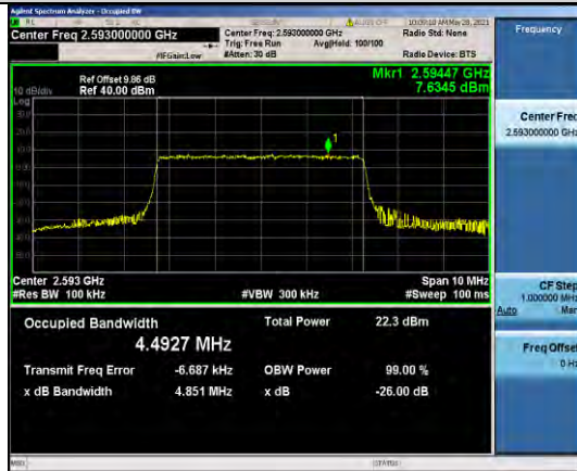
Band41-5MHz-16QAM-40620-25RB#0-4.4927
