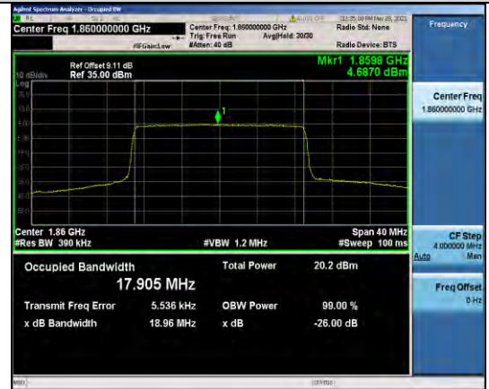
Band25-20MHz-16QAM-26140-100RB#0-17.905
