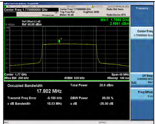
Band66-20MHz-16QAM-132572-100RB#0-17.802
