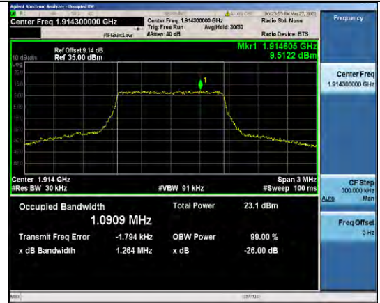
Band25-1.4MHz-QPSK-26683-6RB#0-1.0909
