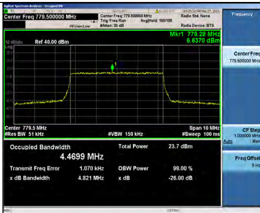
Band13-5MHz-QPSK-23205-25RB#0-4.4699
