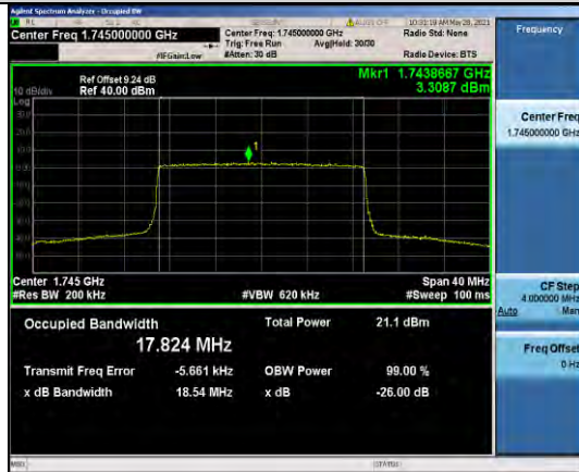
Band66-20MHz-16QAM-132322-100RB#0-17.824
