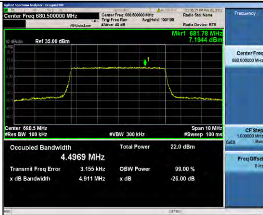
Band71-5MHz-16QAM-133297-25RB#0-4.4969
