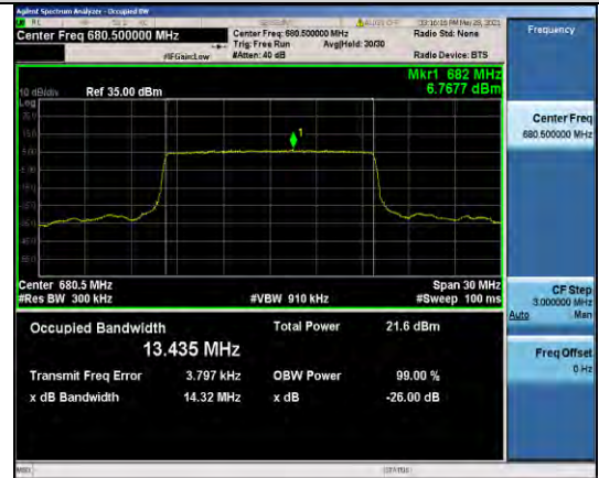
Band71-15MHz-QPSK-133297-75RB#0-13.435
