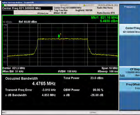
Band26-5MHz-16QAM-26765-25RB#0-4.4765
