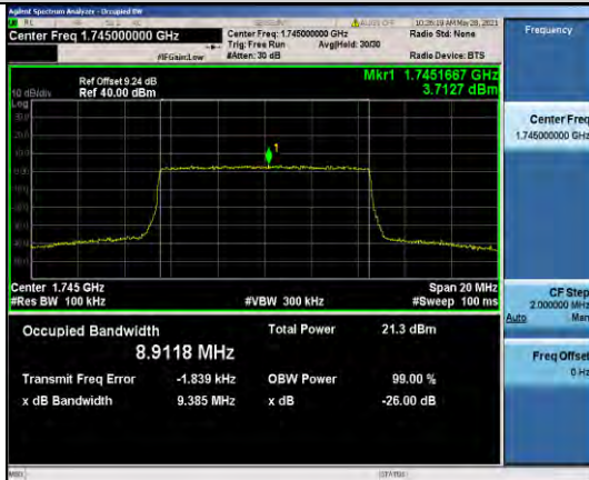
Band66-10MHz-16QAM-132322-50RB#0-8.9118
