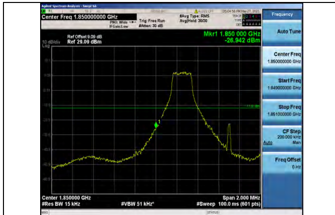
Band2-1.4MHz-QPSK-18607-1RB#0
