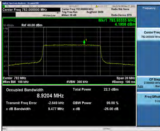
Band13-10MHz-QPSK-23230-50RB#0-8.9204
