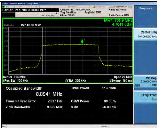
Band12-10MHz-QPSK-23060-50RB#0-8.8941
