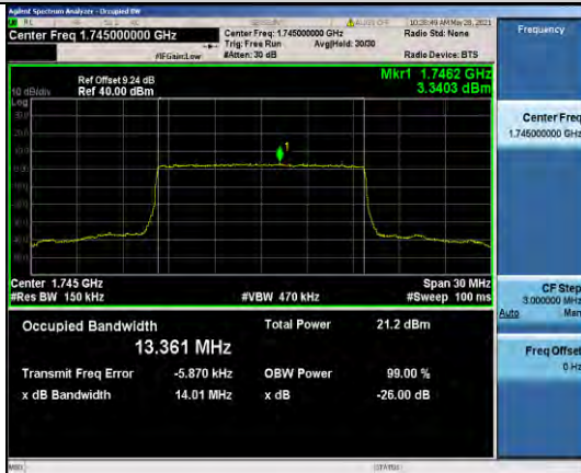
Band66-15MHz-16QAM-132322-75RB#0-13.361
