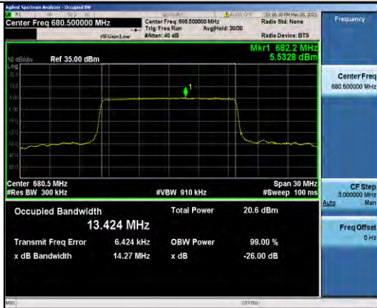
Band71-15MHz-16QAM-133297-75RB#0-13.424
