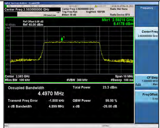
Band41-5MHz-QPSK-40620-25RB#0-4.4970
