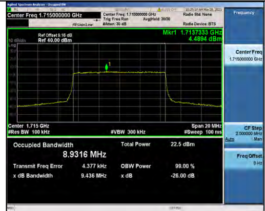
Band66-10MHz-QPSK-132022-50RB#0-8.9316
