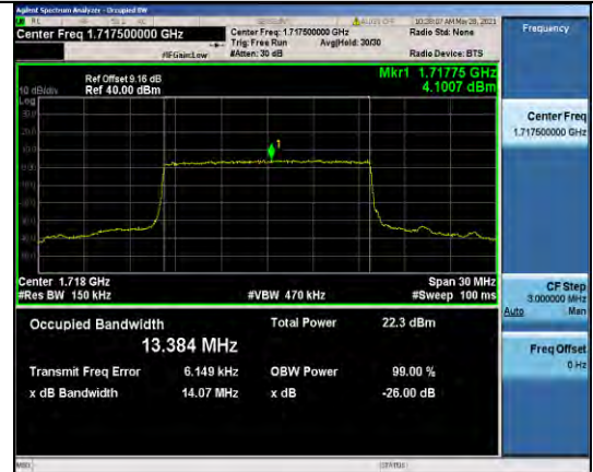
Band66-15MHz-QPSK-132047-75RB#0-13.384
