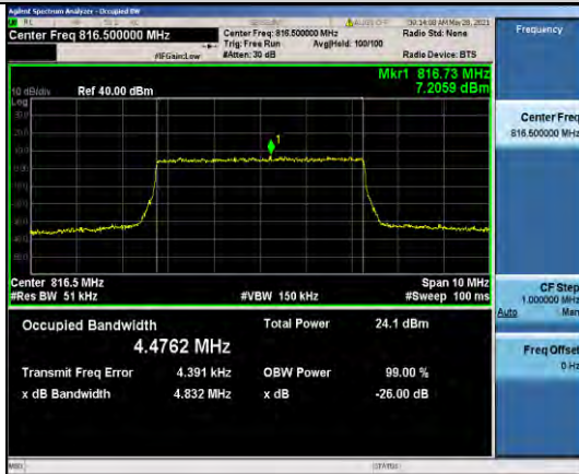
Band26-5MHz-QPSK-26715-25RB#0-4.4762
