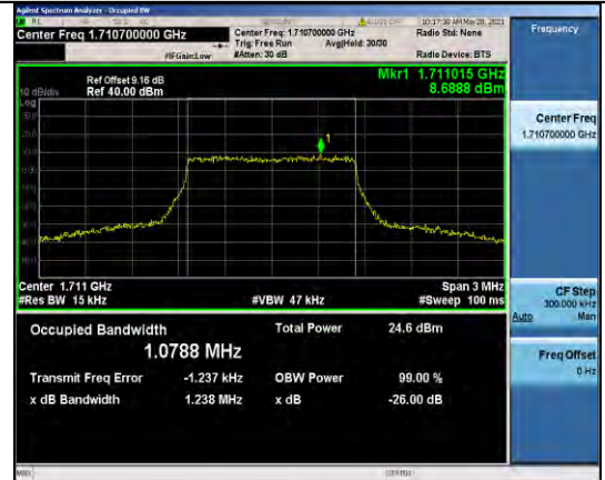
Band66-1.4MHz-QPSK-131979-6RB#0-1.0788
