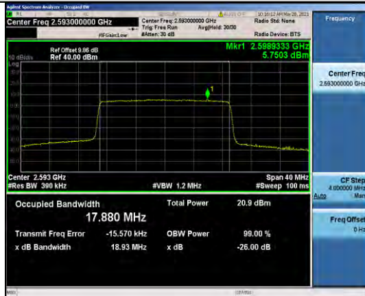
Band41-20MHz-16QAM-40620-100RB#0-17.880
