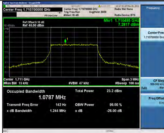
Band66-1.4MHz-16QAM-131979-6RB#0-1.0787
