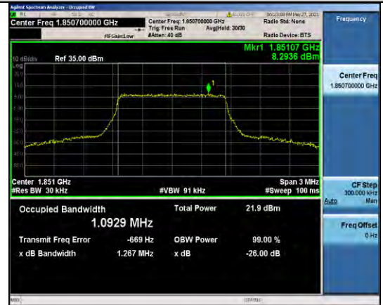
Band25-1.4MHz-16QAM-26047-6RB#0-1.0929
