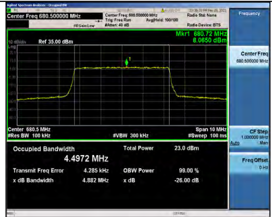
Band71-5MHz-QPSK-133297-25RB#0-4.4972
