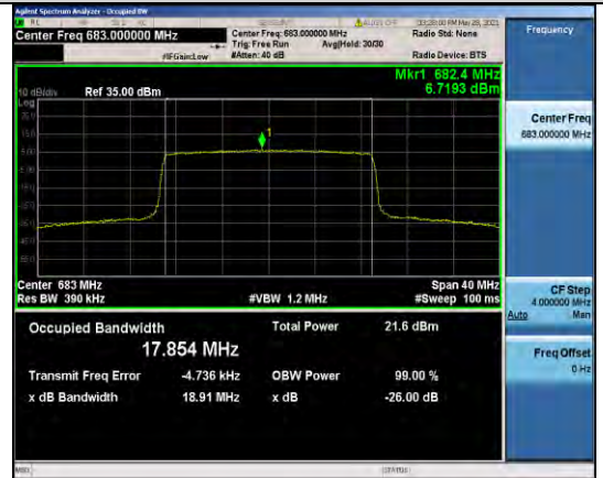
Band71-20MHz-QPSK-133322-100RB#0-17.854
