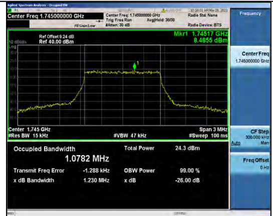
Band66-1.4MHz-QPSK-132322-6RB#0-1.0782
