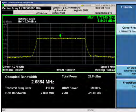
Band66-3MHz-QPSK-132657-15RB#0-2.6884
