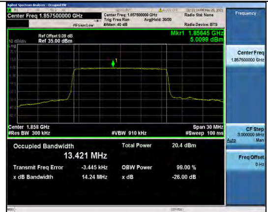
Band25-15MHz-16QAM-26115-75RB#0-13.421
