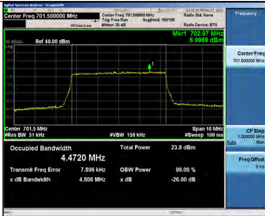
Band12-5MHz-QPSK-23035-25RB#0-4.4720
