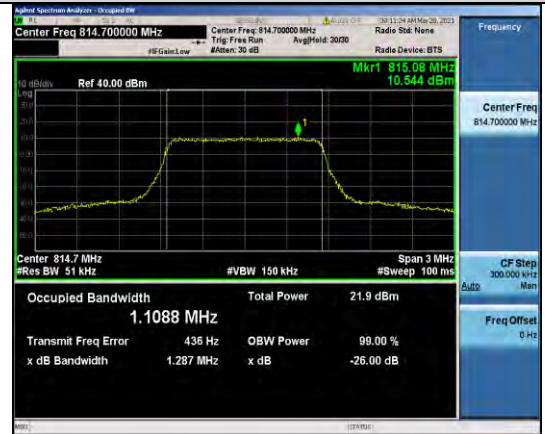
Band26-1.4MHz-16QAM-26697-6RB#0-1.1088
