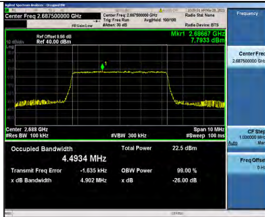
Band41-5MHz-QPSK-41565-25RB#0-4.4934
