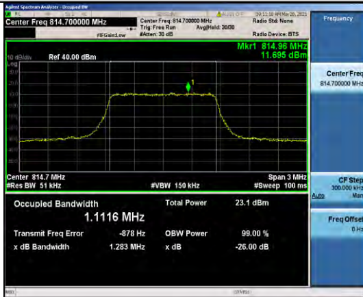
Band26-1.4MHz-QPSK-26697-6RB#0-1.1116
