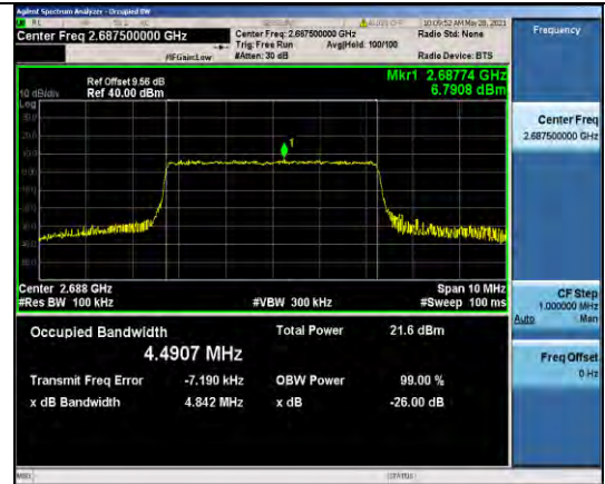
Band41-5MHz-16QAM-41565-25RB#0-4.4907
