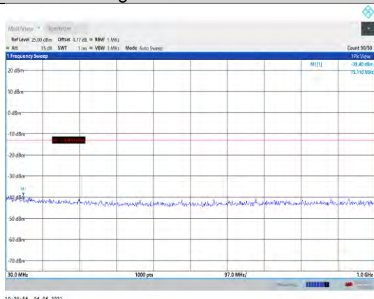
Band66-10MHz-16QAM-132022-1RB#0- Range1:30~1000MHz
