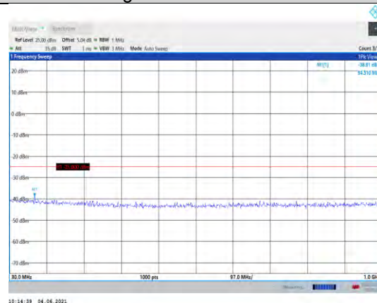
Band41-20MHz-16QAM-39750-1RB#0- Range1:30~1000MHz
