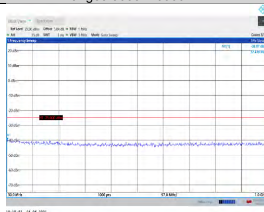
Band41-20MHz-QPSK-40620-1RB#0- Range1:30~1000MHz
