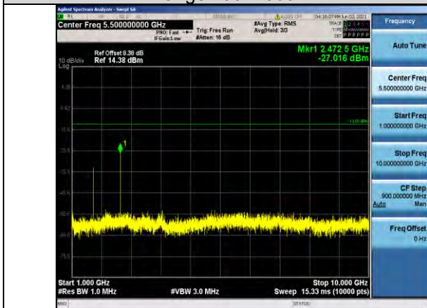
Band5-1.4MHz-QPSK-20407-1RB#0- Range2:1000~10000MHz
