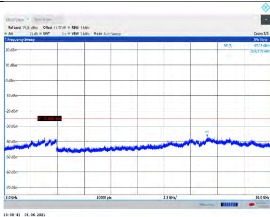
Band41-15MHz-QPSK-40620-1RB#0- Range3:3000~26000MHz
