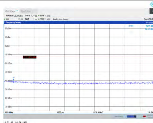
Band66-10MHz-QPSK-132322-1RB#0- Range1:30~1000MHz
