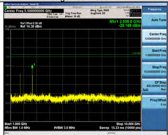
Band5-1.4MHz-QPSK-20525-1RB#0- Range2:1000~10000MHz
