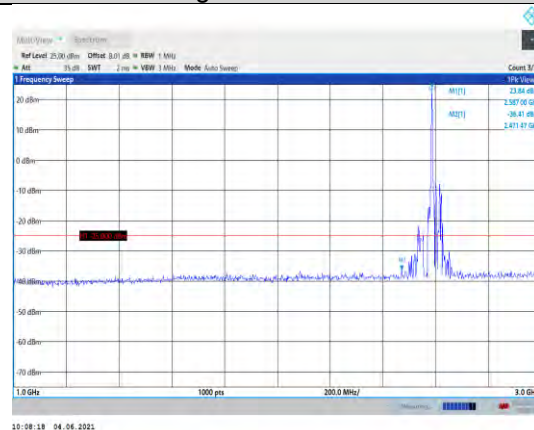
Band41-15MHz-QPSK-40620-1RB#0- Range2:1000~3000MHz
