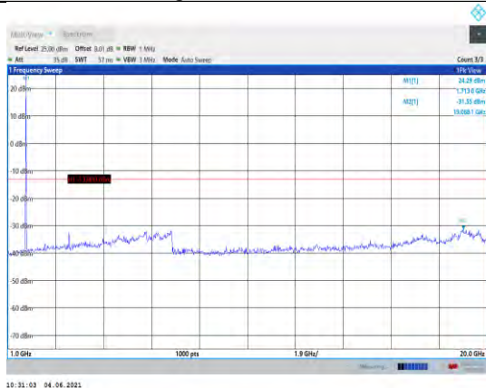
Band66-10MHz-16QAM-132022-1RB#0- Range2:1000~20000MHz
