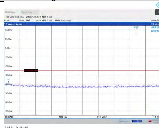
Band41-15MHz-16QAM-39725-1RB#0- Range1:30~1000MHz
