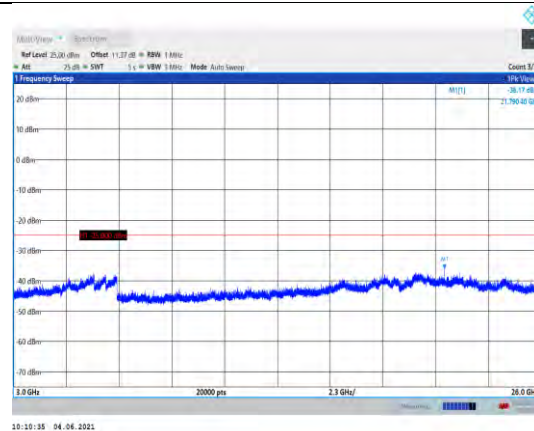
Band41-15MHz-QPSK-41515-1RB#0- Range3:3000~26000MHz
