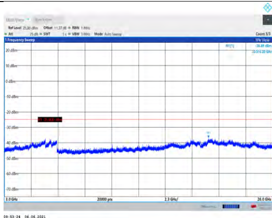
Band41-10MHz-16QAM-39700-1RB#0- Range3:3000~26000MHz
