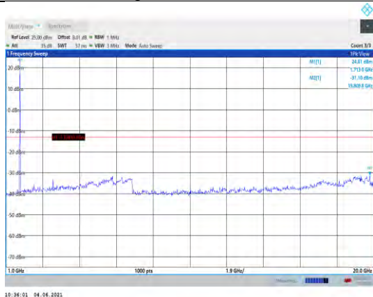
Band66-15MHz-QPSK-132047-1RB#0- Range2:1000~20000MHz
