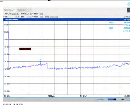
Band66-15MHz-QPSK-132322-1RB#0- Range2:1000~20000MHz
