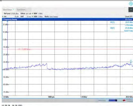
Band66-15MHz-16QAM-132597-1RB#0- Range2:1000~20000MHz
