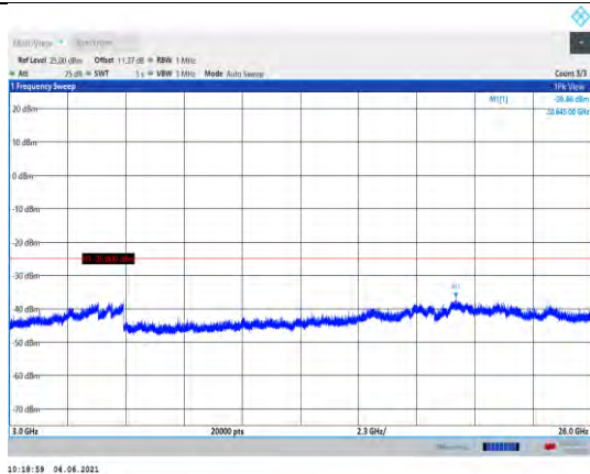
Band41-20MHz-16QAM-41490-1RB#0- Range3:3000~26000MHz
