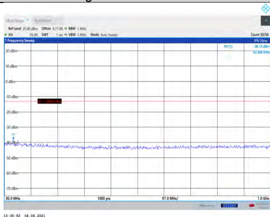
Band66-15MHz-QPSK-132047-1RB#0- Range1:30~1000MHz
