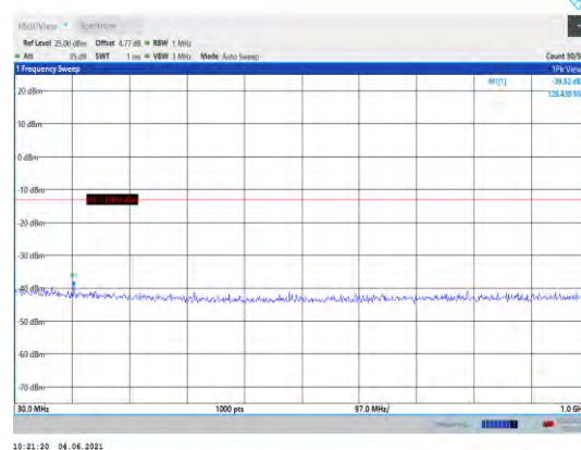
Band66-1.4MHz-QPSK-132665-1RB#0- Range1:30~1000MHz
