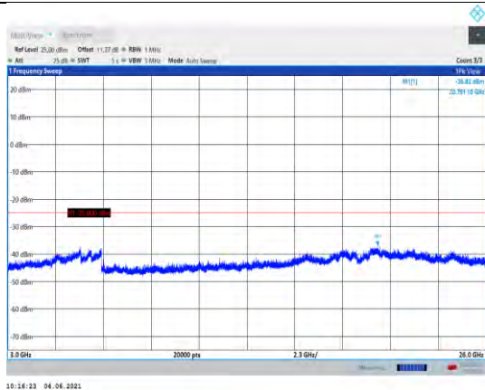
Band41-20MHz-QPSK-40620-1RB#0- Range3:3000~26000MHz
