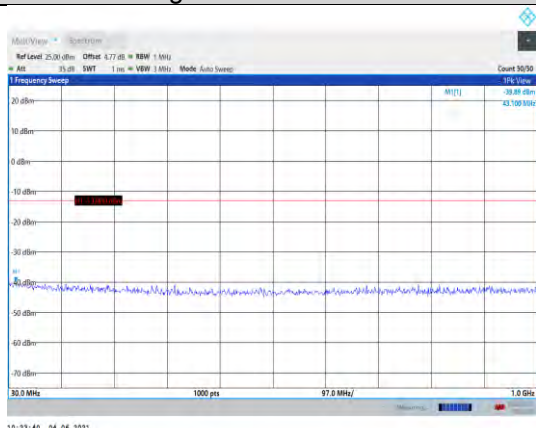
Band66-3MHz-16QAM-131987-1RB#0- Range1:30~1000MHz
