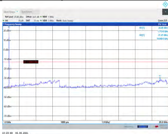
Band66-3MHz-16QAM-131987-1RB#0- Range2:1000~20000MHz
