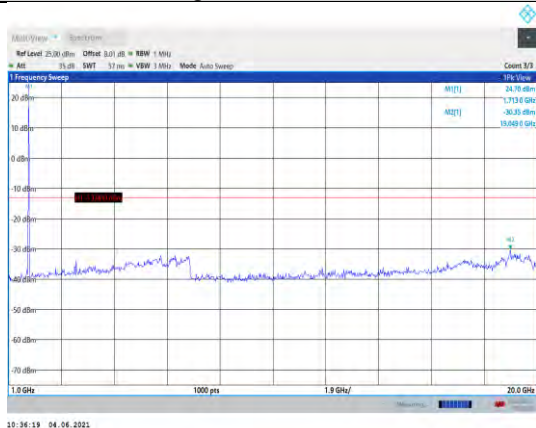
Band66-15MHz-16QAM-132047-1RB#0- Range2:1000~20000MHz
