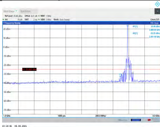
Band41-20MHz-16QAM-40620-1RB#0- Range2:1000~3000MHz
