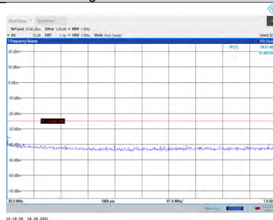
Band41-20MHz-16QAM-41490-1RB#0- Range1:30~1000MHz
