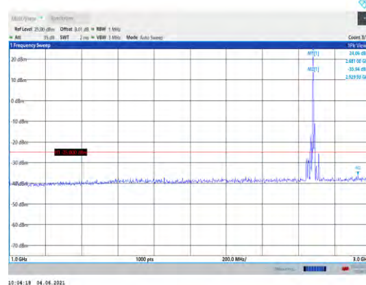
Band41-10MHz-16QAM-41540-1RB#0- Range2:1000~3000MHz
