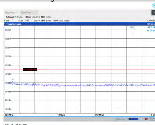
Band41-10MHz-16QAM-41540-1RB#0- Range1:30~1000MHz
