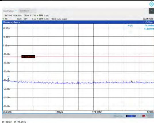
Band66-20MHz-16QAM-132072-1RB#0- Range1:30~1000MHz
