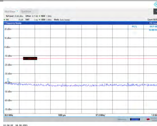
Band66-3MHz-16QAM-132322-1RB#0- Range1:30~1000MHz
