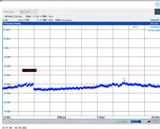
Band41-15MHz-16QAM-39725-1RB#0- Range3:3000~26000MHz
