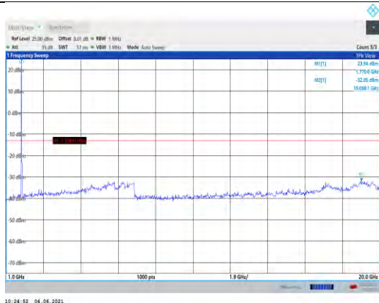
Band66-3MHz-QPSK-132657-1RB#0- Range2:1000~20000MHz
