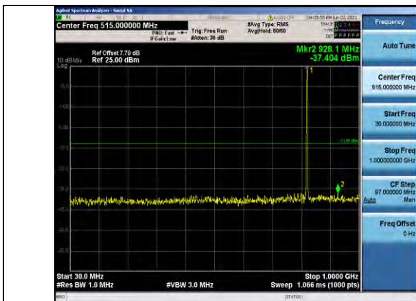
Band5-1.4MHz-QPSK-20407-1RB#0- Range1:30~1000MHz
