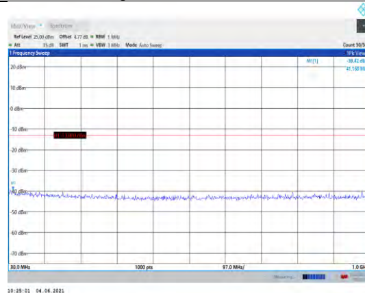
Band66-3MHz-16QAM-132657-1RB#0- Range1:30~1000MHz
