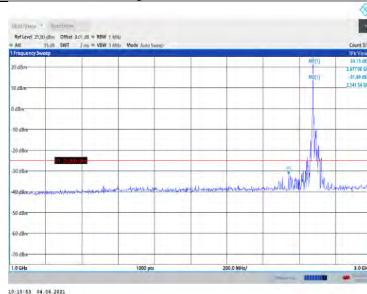
Band41-15MHz-16QAM-41515-1RB#0- Range2:1000~3000MHz
