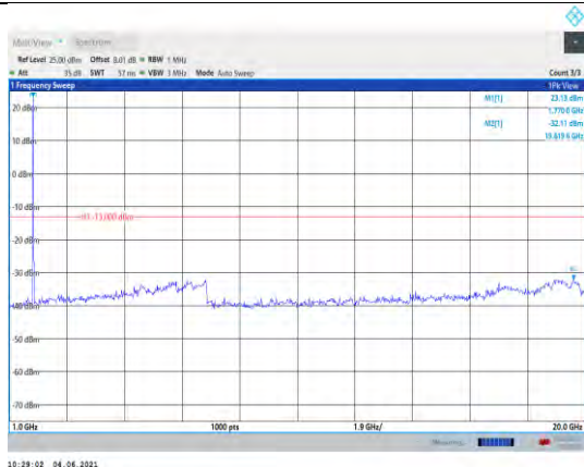
Band66-5MHz-16QAM-132647-1RB#0- Range2:1000~20000MHz
