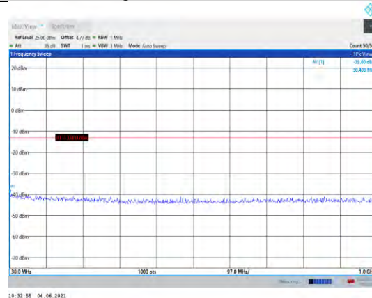
Band66-10MHz-QPSK-132622-1RB#0- Range1:30~1000MHz
