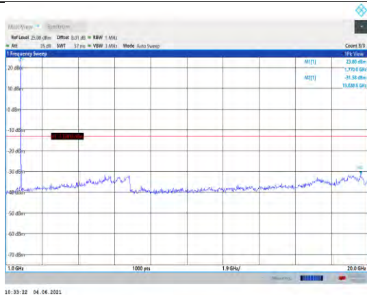
Band66-10MHz-16QAM-132622-1RB#0- Range2:1000~20000MHz
