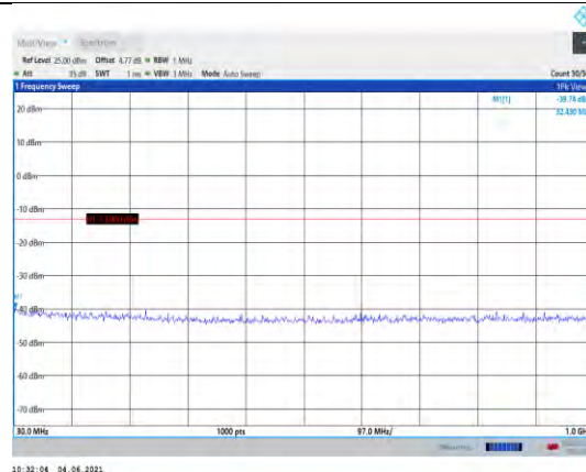
Band66-10MHz-16QAM-132322-1RB#0- Range1:30~1000MHz
