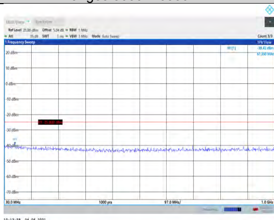
Band41-20MHz-QPSK-39750-1RB#0- Range1:30~1000MHz
