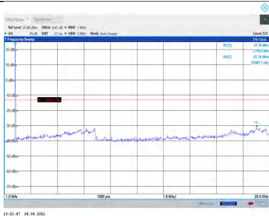
Band66-1.4MHz-16QAM-132665-1RB#0- Range2:1000~20000MHz
