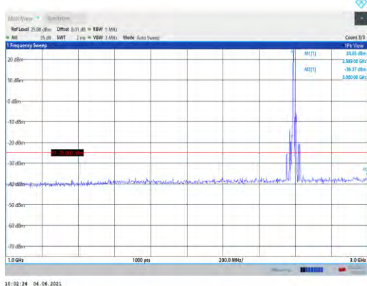
Band41-10MHz-16QAM-40620-1RB#0- Range2:1000~3000MHz
