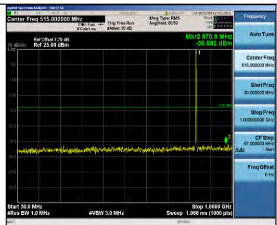
Band5-1.4MHz-QPSK-20525-1RB#0- Range1:30~1000MHz
