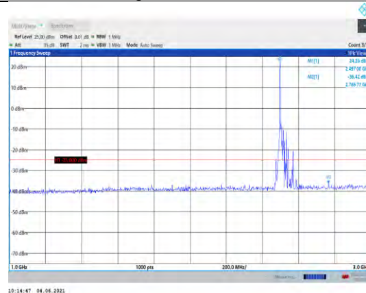
Band41-20MHz-16QAM-39750-1RB#0- Range2:1000~3000MHz
