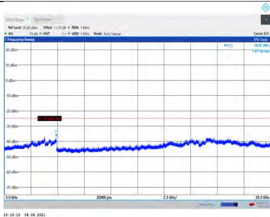
Band41-20MHz-16QAM-39750-1RB#0- Range3:3000~26000MHz
