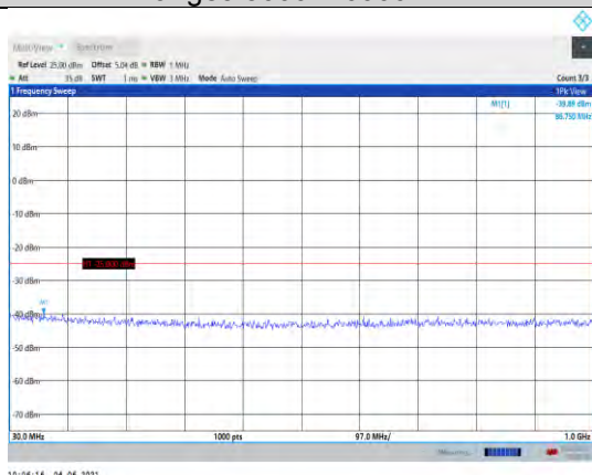
Band41-15MHz-QPSK-39725-1RB#0- Range1:30~1000MHz
