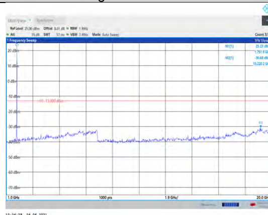
Band66-3MHz-16QAM-132322-1RB#0- Range2:1000~20000MHz
