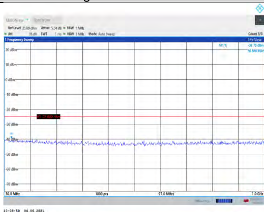
Band41-15MHz-16QAM-40620-1RB#0- Range1:30~1000MHz
