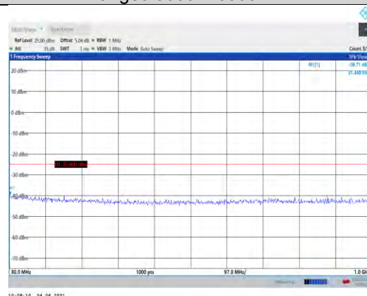
Band41-15MHz-QPSK-40620-1RB#0- Range1:30~1000MHz
