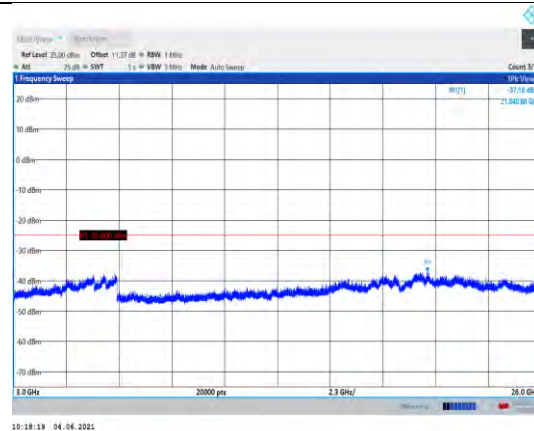
Band41-20MHz-QPSK-41490-1RB#0- Range3:3000~26000MHz
