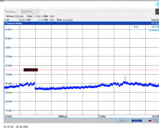
Band41-15MHz-16QAM-40620-1RB#0- Range3:3000~26000MHz
