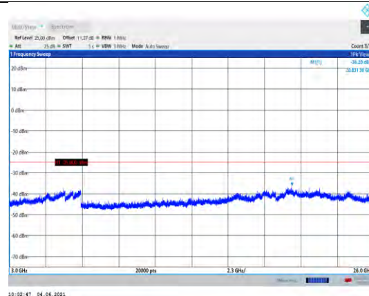
Band41-10MHz-16QAM-40620-1RB#0- Range3:3000~26000MHz
