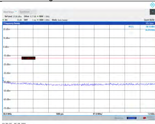
Band66-10MHz-QPSK-132022-1RB#0- Range1:30~1000MHz
