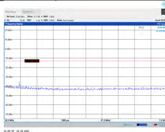
Band66-5MHz-QPSK-132647-1RB#0- Range1:30~1000MHz
