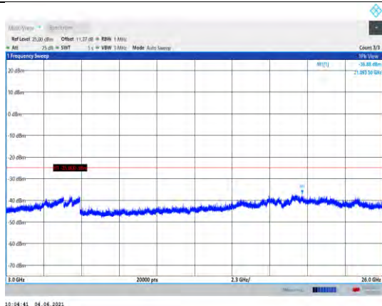
Band41-10MHz-16QAM-41540-1RB#0- Range3:3000~26000MHz
