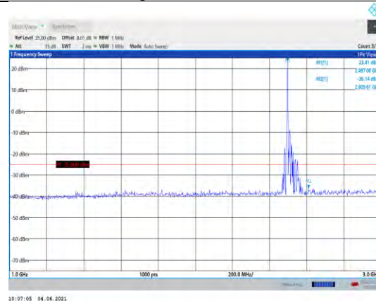
Band41-15MHz-16QAM-39725-1RB#0- Range2:1000~3000MHz
