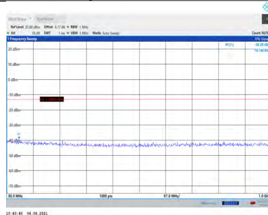
Band66-20MHz-16QAM-132572-1RB#0- Range1:30~1000MHz
