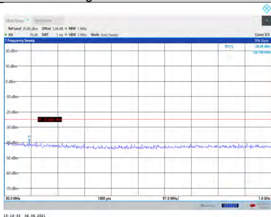
Band41-20MHz-16QAM-40620-1RB#0- Range1:30~1000MHz
