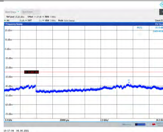
Band41-20MHz-16QAM-40620-1RB#0- Range3:3000~26000MHz
