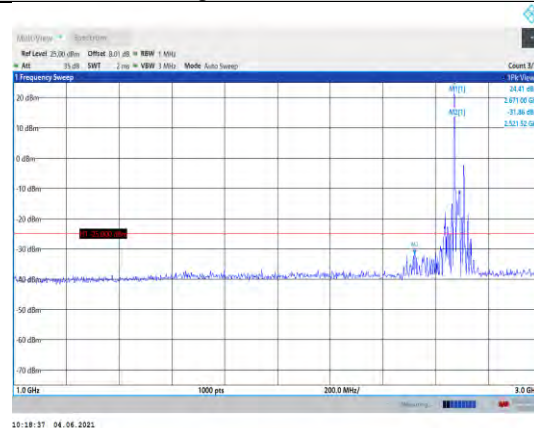
Band41-20MHz-16QAM-41490-1RB#0- Range2:1000~3000MHz
