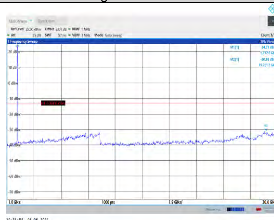
Band66-10MHz-QPSK-132322-1RB#0- Range2:1000~20000MHz
