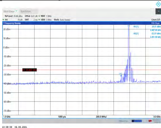
Band41-15MHz-16QAM-40620-1RB#0- Range2:1000~3000MHz
