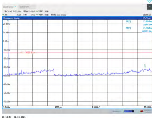
Band66-1.4MHz-QPSK-131979-1RB#0- Range2:1000~20000MHz
