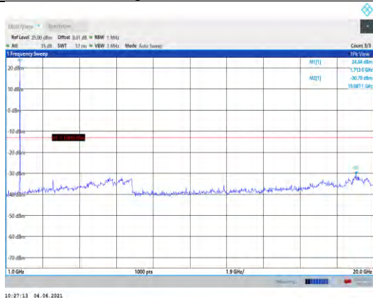
Band66-5MHz-16QAM-131997-1RB#0- Range2:1000~20000MHz
