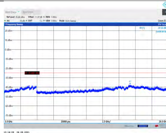
Band41-20MHz-QPSK-39750-1RB#0- Range3:3000~26000MHz
