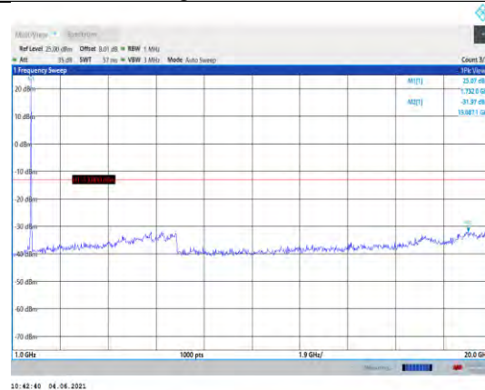
Band66-20MHz-16QAM-132322-1RB#0- Range2:1000~20000MHz
