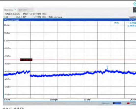
Band41-15MHz-QPSK-39725-1RB#0- Range3:3000~26000MHz
