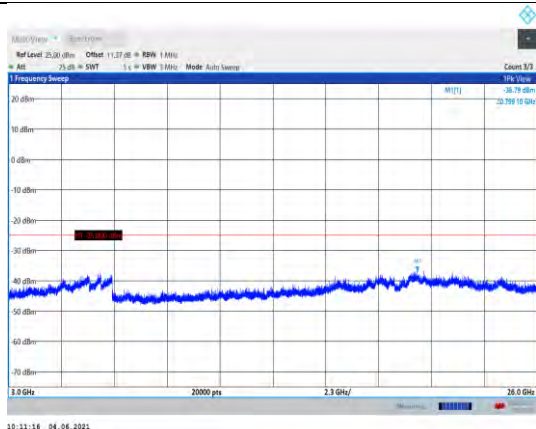
Band41-15MHz-16QAM-41515-1RB#0- Range3:3000~26000MHz
