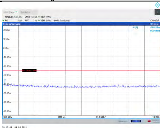
Band41-15MHz-QPSK-41515-1RB#0- Range1:30~1000MHz
