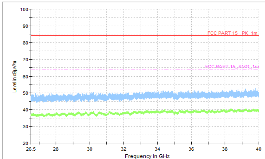
Figure A.12 Radiated Emission (Set.1, LTE Band 5 Receiver, 26.5GHz to 40GHz)
