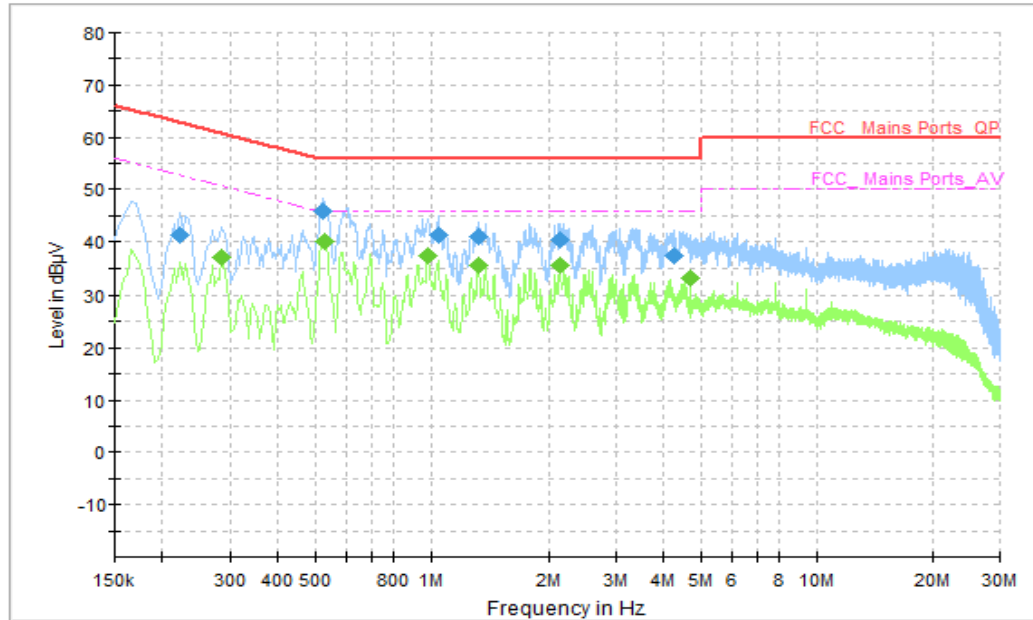
Figure B.10 Conducted Emission(Set.4, FM receiver)
