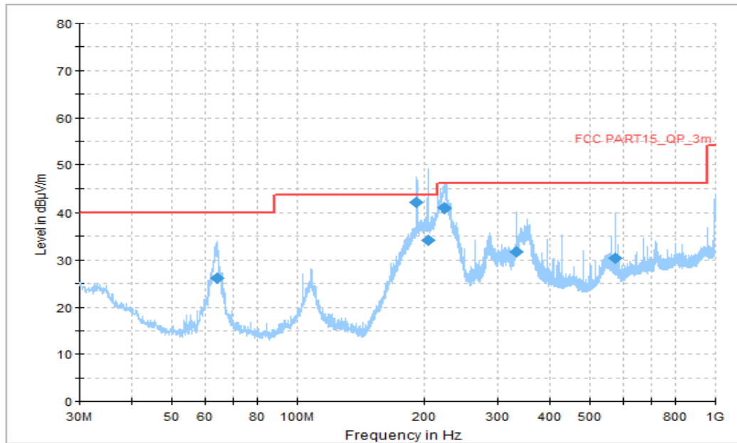
Figure A.69 Radiated Emission (Set.5, Data Transfer Mode: TF Card to PC, 30MHz to 1GHz)
