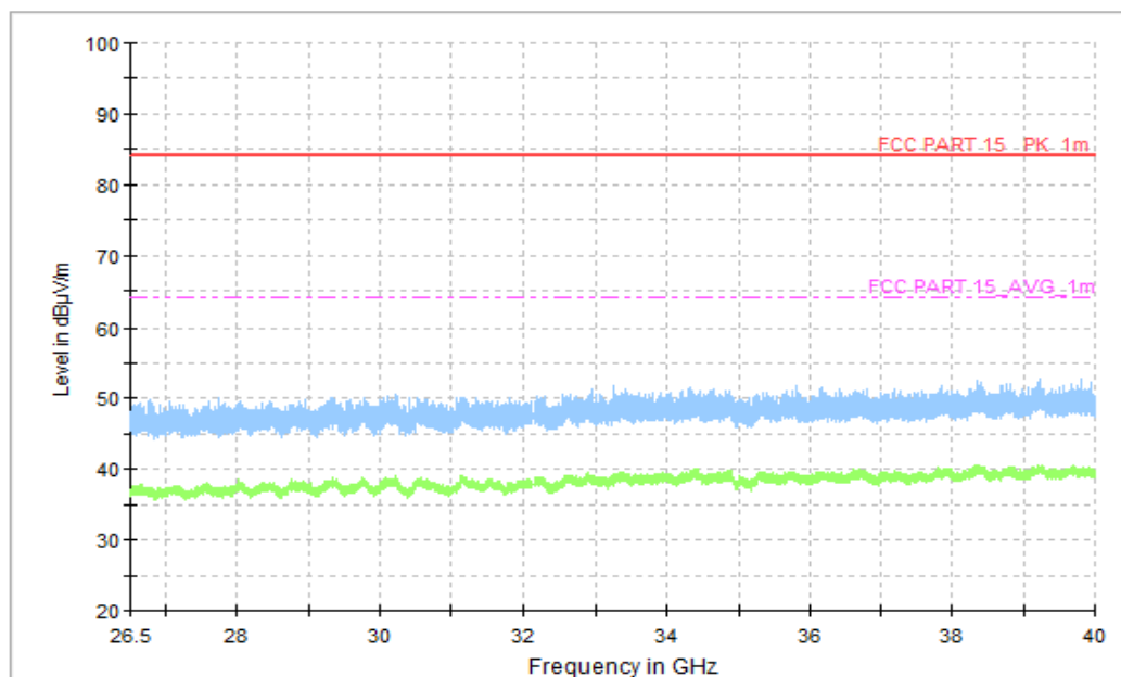
Figure A.20 Radiated Emission (Set.2, LTE Band 12 Receiver, 26.5GHz to 40GHz)
