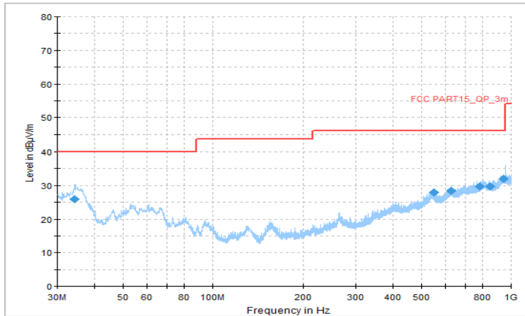
Figure A.37 Radiated Emission (Set.2, LTE Band 13 Receiver, 30MHz to 1GHz)
