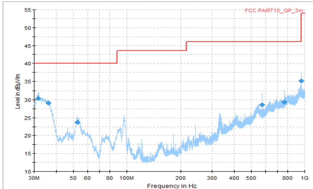
Figure A.13 Radiated Emission (Set.1, LTE Band 12 Receiver, 30MHz to 1GHz)
