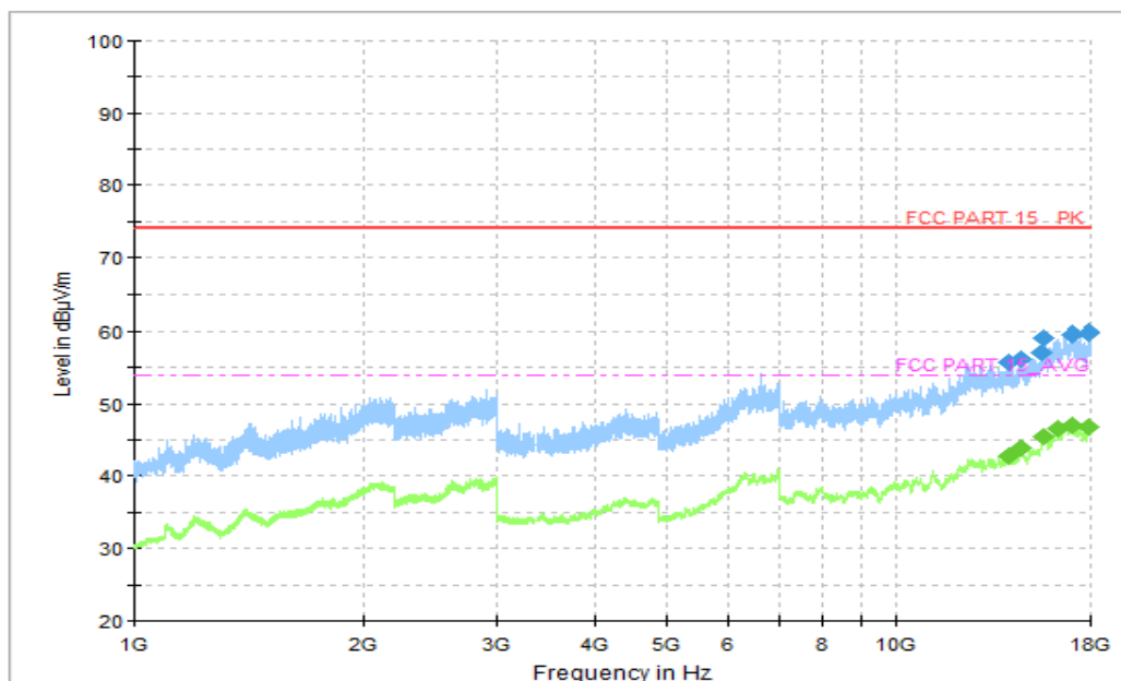
Figure A.74 Radiated Emission (Set.6, Data Transfer Mode: TF Card to PC, 1GHz to 18GHz)
