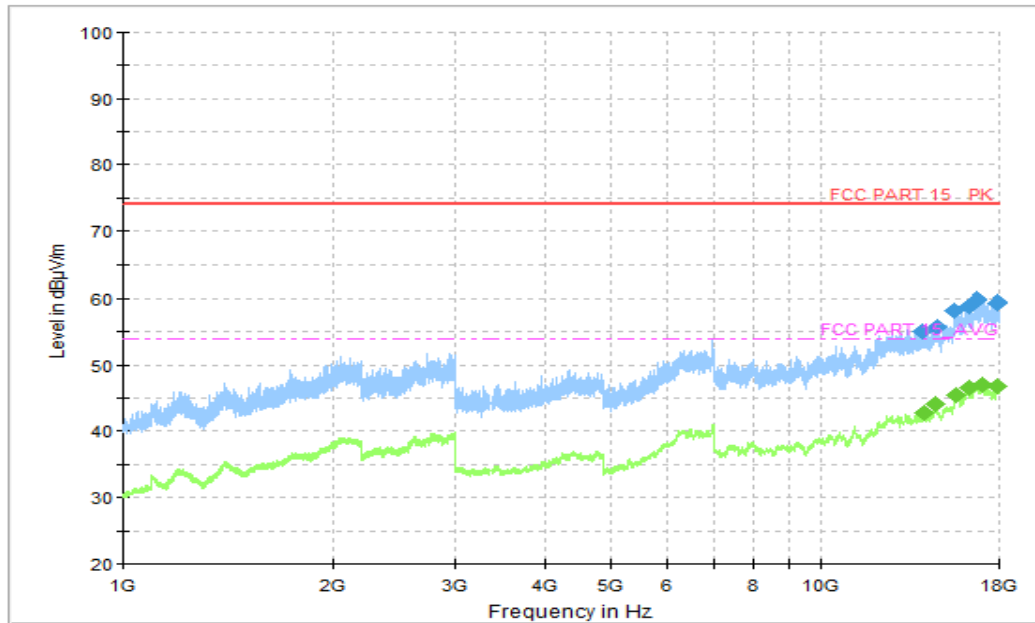
Figure A.66 Radiated Emission (Set.5, Data Transfer Mode: PC to TF Card, 1GHz to 18GHz)
