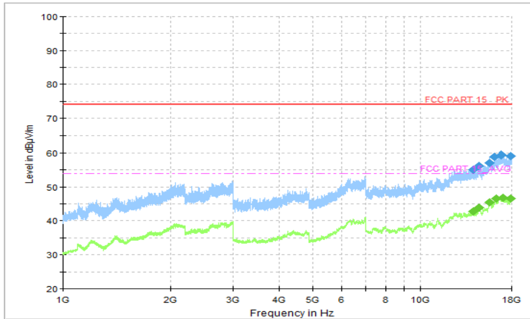
Figure A.62 Radiated Emission (Set.5, Data Transfer Mode: PC to EUT, 1GHz to 18GHz)
