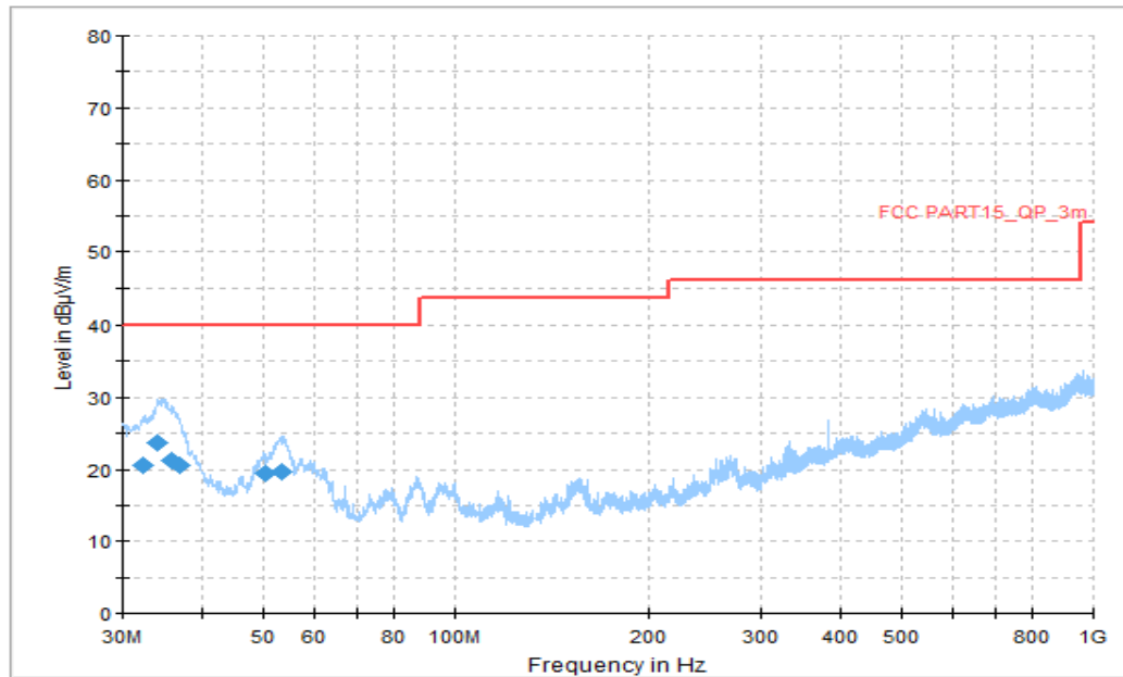
Figure A.53 Radiated Emission (Set.2 Video Player Mode, 30MHz to 1GHz)
