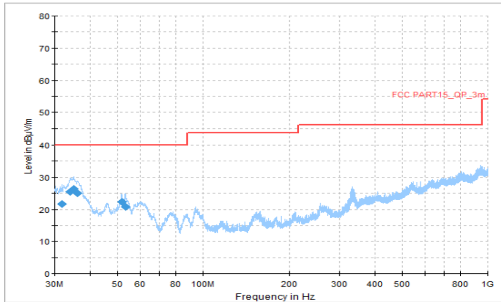
Figure A.17 Radiated Emission (Set.2, LTE Band 12 Receiver, 30MHz to 1GHz)
