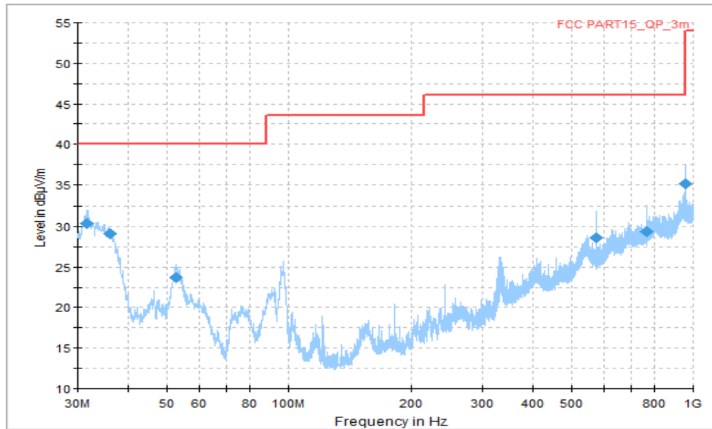
Figure A.9 Radiated Emission (Set.1, LTE Band 5 Receiver, 30MHz to 1GHz)
