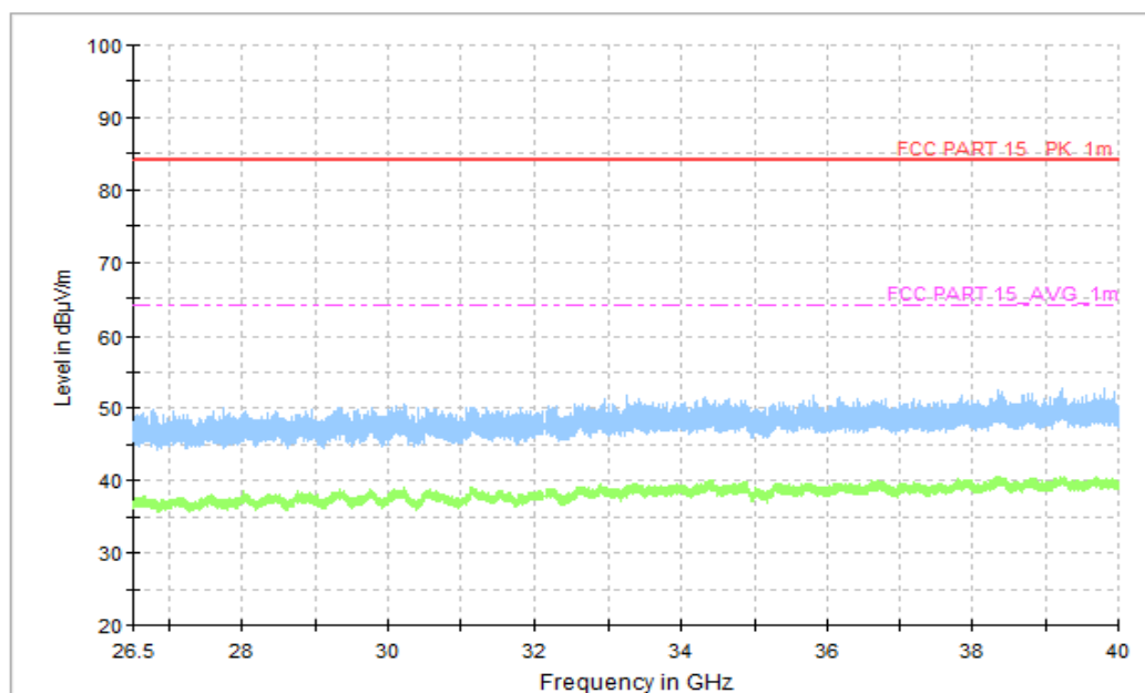
Figure A.52 Radiated Emission (Set.1, Video Player Mode, 26.5GHz to 40GHz)
