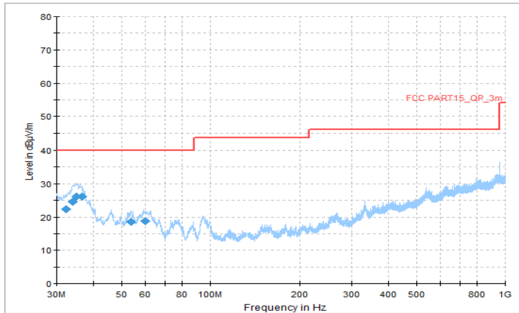
Figure A.49 Radiated Emission (Set.1, Video Player Mode, 30MHz to 1GHz)
