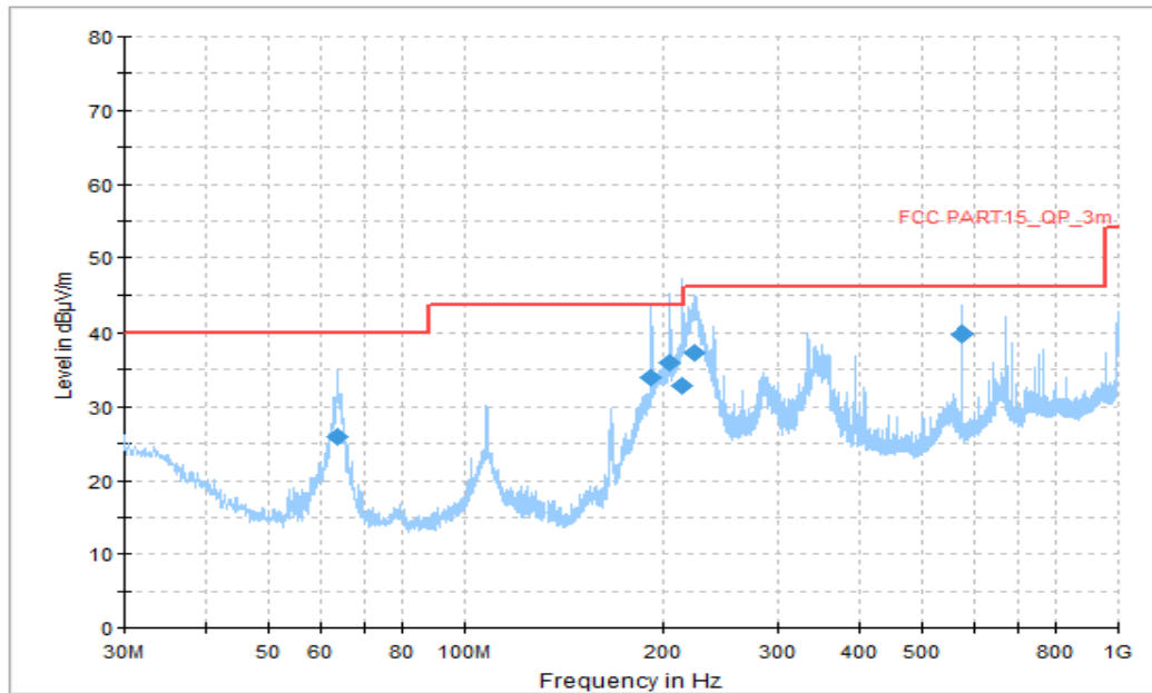
Figure A.65 Radiated Emission (Set.5, Data Transfer Mode: PC to TF Card, 30MHz to 1GHz)
