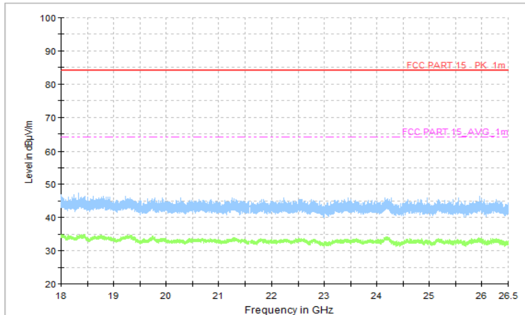
Figure A.11 Radiated Emission (Set.1, LTE Band 5 Receiver, 18GHz to 26.5GHz)
