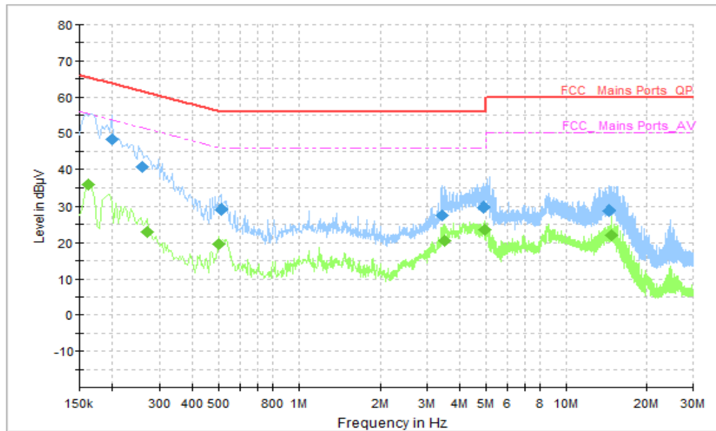
Figure B.11 Conducted Emission(Set.5, Data Transfer Mode)
