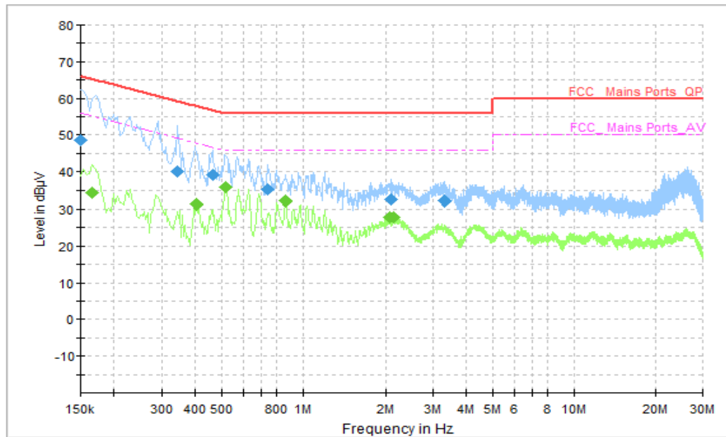
Figure B.3 Conducted Emission(Set.3, FM receiver)
