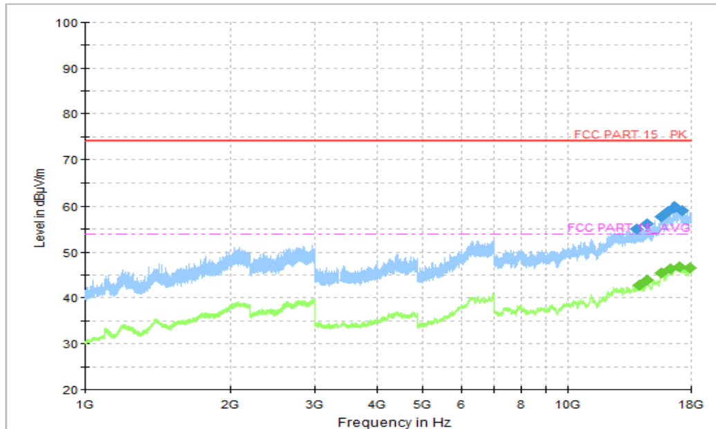
Figure A.58 Radiated Emission (Set.5, Data Transfer Mode: EUT to PC, 1GHz to 18GHz)
