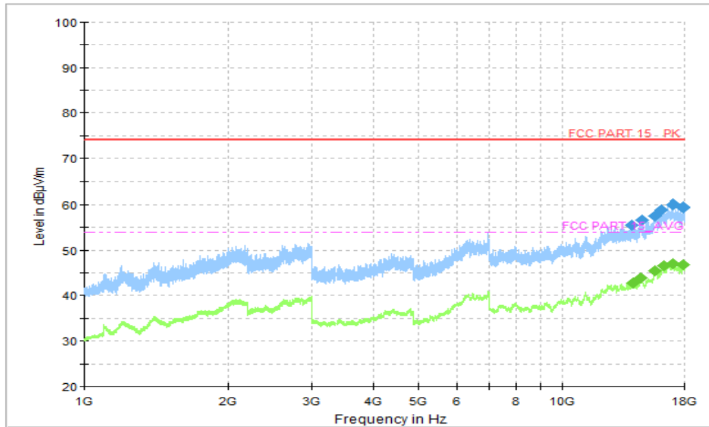
Figure A.70 Radiated Emission (Set.5, Data Transfer Mode: TF Card to PC, 1GHz to 18GHz)
