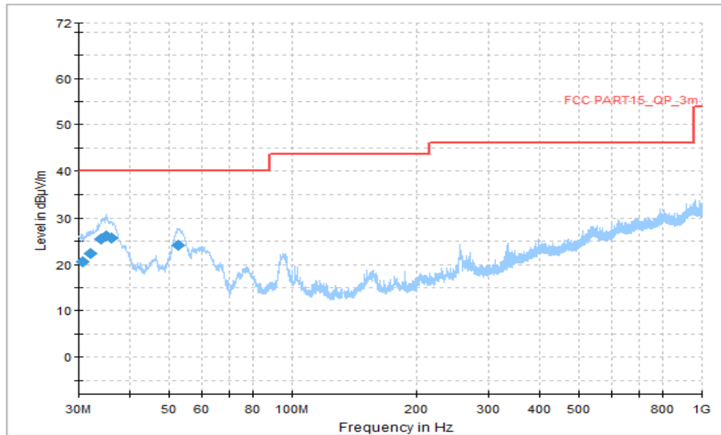
Figure A.21 Radiated Emission (Set.1, LTE Band 13 Receiver, 30MHz to 1GHz)
