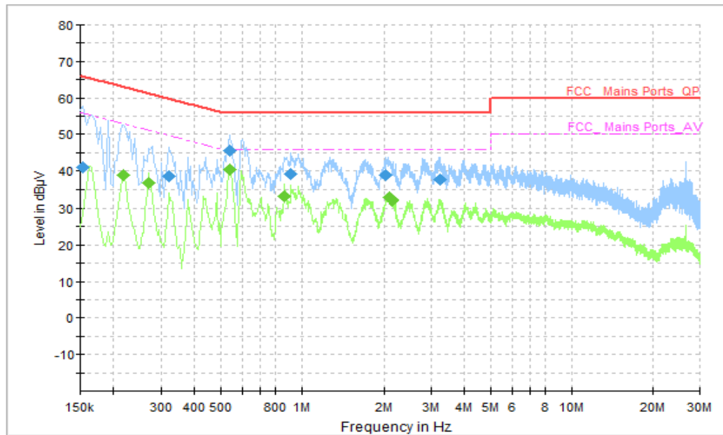
Figure B.9 Conducted Emission(Set.3, FM receiver)
