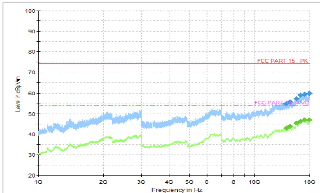
Figure A.18 Radiated Emission (Set.2, LTE Band 12 Receiver , 1GHz to 18GHz)
