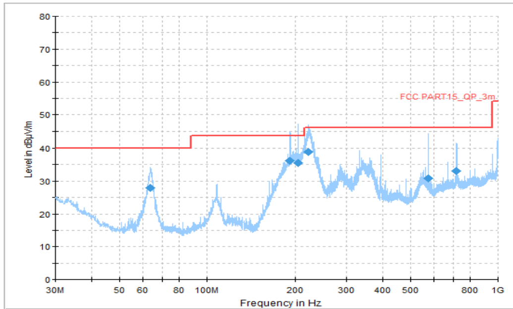
Figure A.57 Radiated Emission (Set.5, Data Transfer Mode: EUT to PC, 30MHz to 1GHz)
