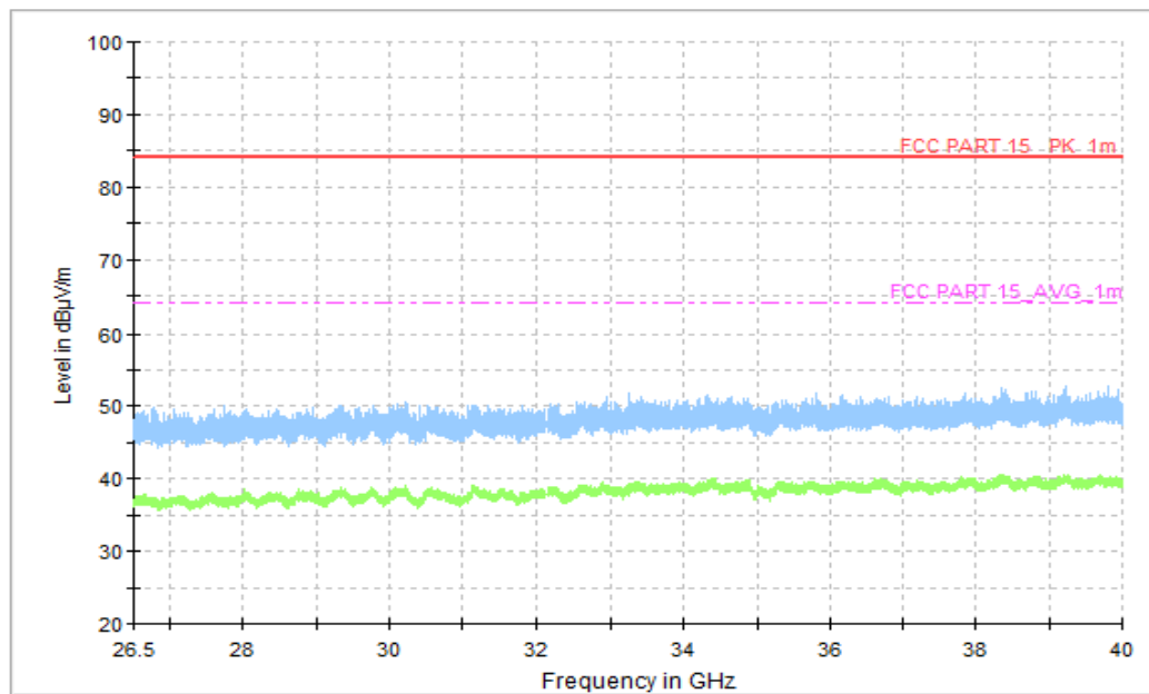
Figure A.44 Radiated Emission (Set.1, Camera Mode , 26.5GHz to 40GHz)
