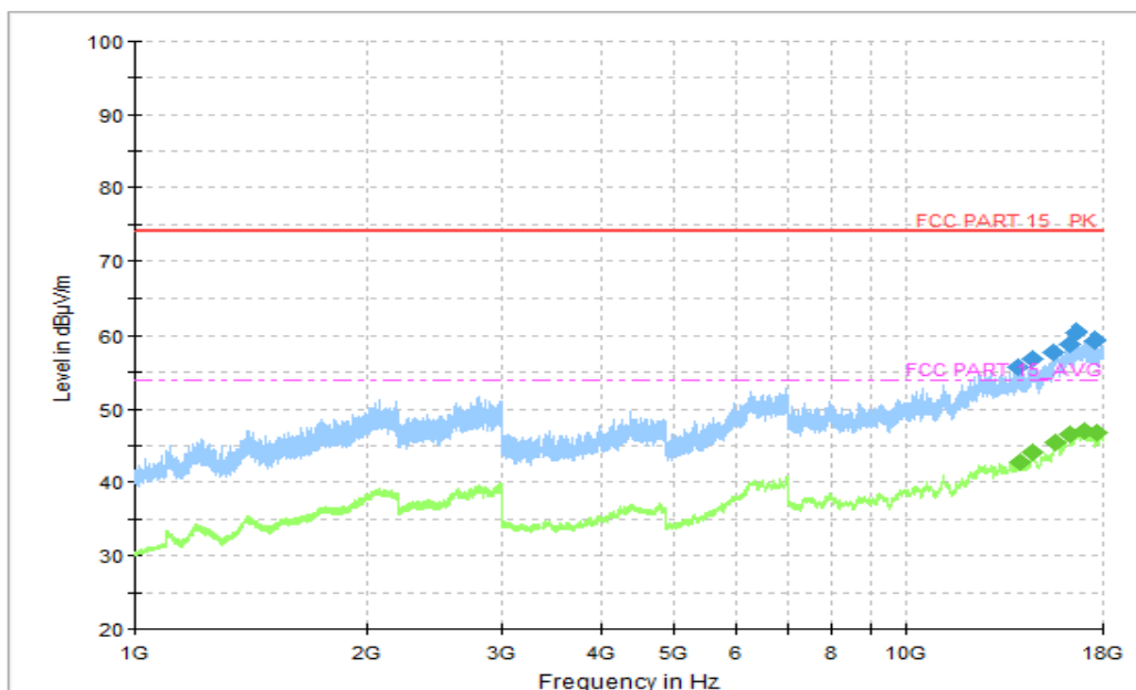
Figure A.14 Radiated Emission (Set.1, LTE Band 12 Receiver , 1GHz to 18GHz)
