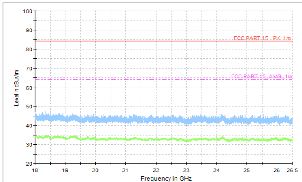
Figure A.51 Radiated Emission (Set.1, Video Player Mode, 18GHz to 26.5GHz)
