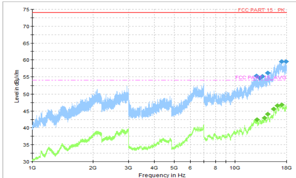
Figure A.34 Radiated Emission (Set.2, LTE Band 5 Receiver , 1GHz to 18GHz)
