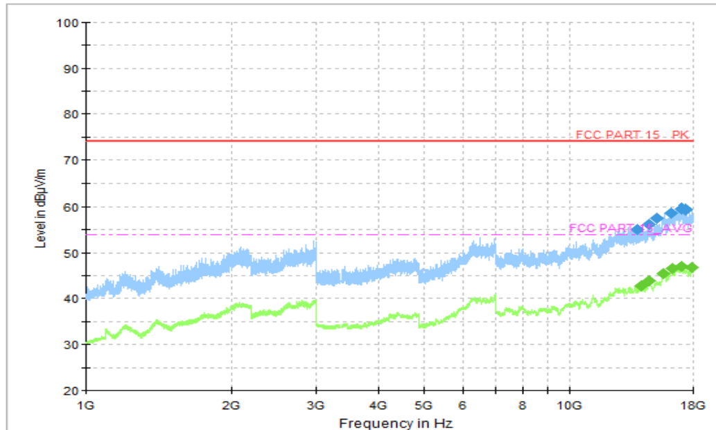
Figure A.38 Radiated Emission (Set.2, LTE Band 13 Receiver , 1GHz to 18GHz)
