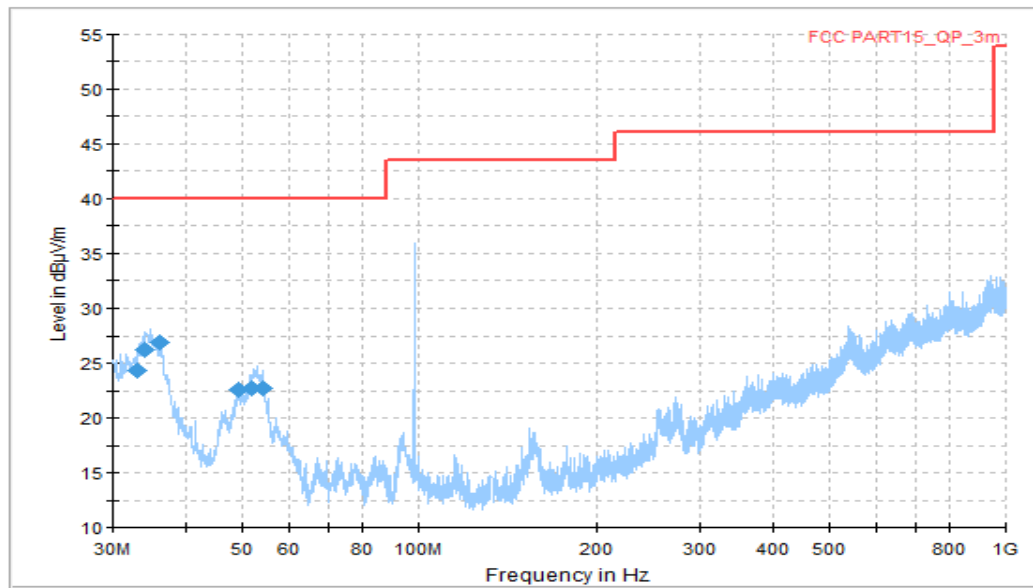
Figure A.45 Radiated Emission (Set.3,FM receiver, 30MHz to 1GHz)
