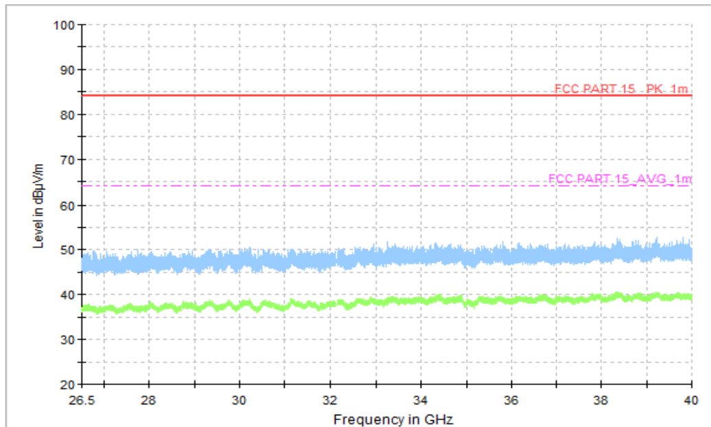
Figure A.68 Radiated Emission (Set.5, Data Transfer Mode: PC to TF Card, 26.5GHz to 40GHz)
