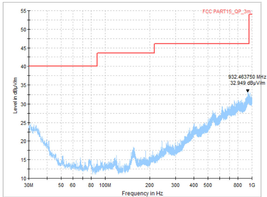
Fig.22 Radiated Spurious Emission (Ch19, 30 MHz - 1 GHz), 1M
